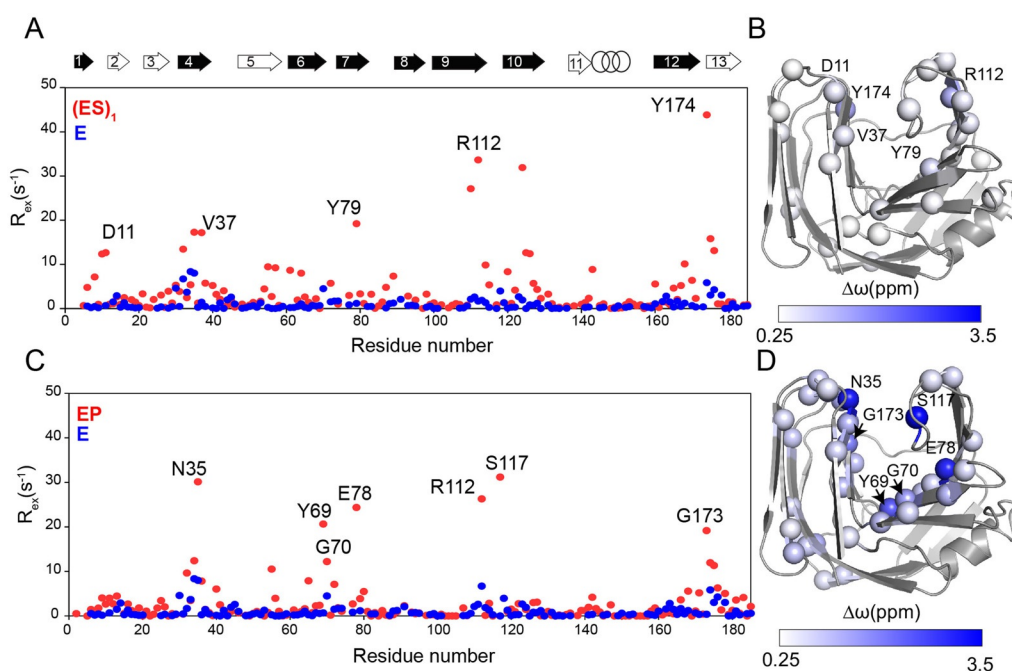
Figure 3. Non-covalent interactions enhance BCX millisecond time scale dynamics in the (ES) 1 and EP states. A,C) Overlay of the R_{\text{ex}} values of (ES) 1 (A) or EP (C) (red dots) and E states (blue dots) plotted versus the residue number. Several residues that show a prominent difference in R_{\text{ex}} are labeled. The secondary structure elements of BCX are represented by black arrows for \beta -strands of sheet A and in white ones for sheet B and the \alpha -helix in rings. The “thumb” loop connects \beta -strands 9 and 10. B,D) Amide nitrogen atoms used in the RD global fit for (ES) 1 (B) and EP (D) are shown in spheres on the BCX crystal structure (PDB ID: 2bv) colored by their \Delta\omega between the ground and excited states, using a white/blue gradient. The \Delta\omega were derived from a global two-state fit to the dispersion curves.
