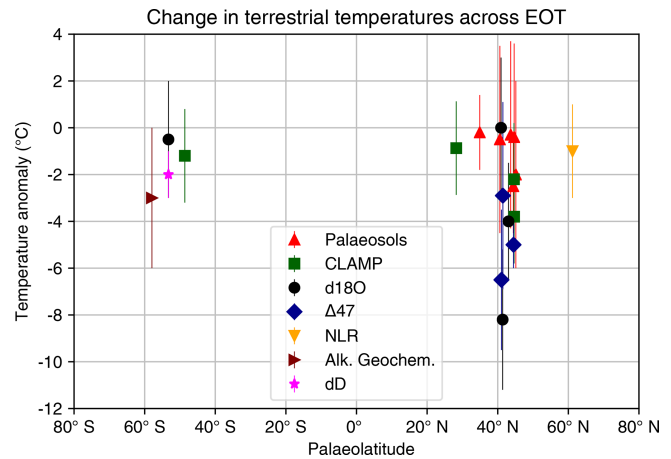
Figure 4. Summary of terrestrial air temperature change across the EOT from proxies palaeosols, CLAMP, \delta^{18}\text{O} , \Delta_{47} , nearest living relative (NLR), alkaline geochemistry and \delta\text{D} (hydrogen isotopes). Data are compiled from Boardman and Secord (2013), Colwyn and Hren (2019), Eldrett et al. (2009), Fan et al. (2017), Gallagher and Sheldon (2013), Hérán et al. (2010), Herman et al. (2017), Hinojosa and Villagrán (2005), Hren et al. (2013), Kohn et al. (2004), Kvaček et al. (2014), Lielke et al. (2012), Meyers (2003), Page et al. (2019), Passchier et al. (2013), Roth-Nebelsick et al. (2017), Sheldon and Tabor (2009) and Zanazzi et al. (2007). Where possible, we apply the same method as in Fig. 3; i.e. the “late Eocene” is taken the average temperature from 38 to 33.9 Ma, the “early Oligocene” is taken as the average from 33.9 to 30 Ma and the temperature change shown here is the difference. However, in a number of cases only a relative temperature change across the EOT was given in the original literature. We therefore limit our compilation to temperature anomaly only. The compilation shown above is provided in digital form in Table S2 in the Supplement.
