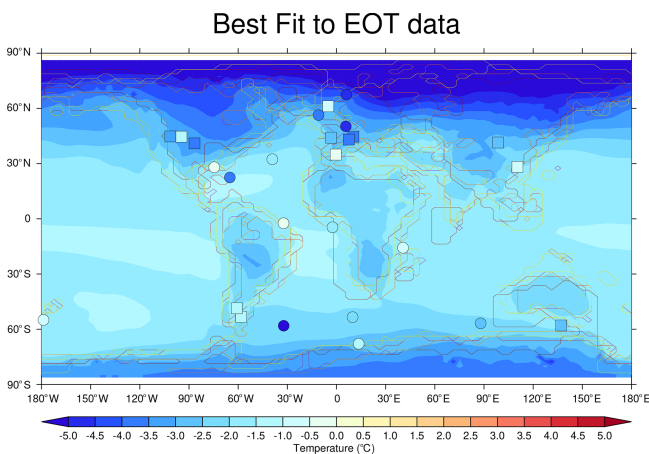
Figure 8. Ensemble mean modelled SAT response to a CO 2 decrease from 885 to 560 ppmv, representing the best fit to the proxy data. The marine proxy data are shown as filled circles, while the terrestrial proxy data are shown as filled squares. Coastlines from each model are plotted to illustrate the uncertainties associated with the palaeogeographic reconstructions.
