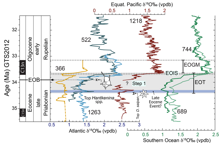
Figure 1. Oxygen stable isotope and chronostratigraphic characteristics of the Eocene–Oligocene transition (EOT) from deep marine records and EOT terminology on the GTS2012 timescale. Benthic foraminiferal \delta^{18}\text{O} from six deep-sea drill holes are shown: tropical Atlantic Site 366, South Atlantic sites 522 and 1263 (Zachos et al., 1996; Langton et al., 2016); Southern Ocean sites 744 and 689 (Zachos et al., 1996; Diester-Haass and Zahn, 1996) and equatorial Pacific Site 1218 (Coxall and Wilson 2011). Due to different sample resolutions, running means are applied using a three-point filter for sites 522, 689 and 1263; five-point filter for sites 366 and 744; and a seven-point filter for Site 1218. Timescale conversions were made by aligning common magnetostratigraphic tie points. The EOT is defined as a ca. 790 kyr long phase of accelerated climatic and biotic change that began before and ended after the Eocene–Oligocene boundary (EOB) (after Coxall and Pearson, 2007). It is bounded at the base by the “top” D. saipanensis nannofossil extinction event and above by the EOIS- \delta^{18}\text{O} maximum. Benthic data are all Cibicidoides spp. or “ Cibs. equivalent” and have not been adjusted to seawater equilibrium values. “Step 1” comprises a modest \delta^{18}\text{O} increase linked to ocean cooling (Lear et al., 2008; Bohaty et al., 2012). The “top Hantkenina spp.” marker corresponds to the position of this extinction event at DSDP Site 522 (including sampling bracket) with respect to the corresponding Site 522 \delta^{18}\text{O} curve. That it coincides with the published calibrated age of this event (33.9 Myr) is entirely independent. The “late Eocene event” \delta^{18}\text{O} maximum (after Katz et al., 2008) may represent a failed glaciation.
