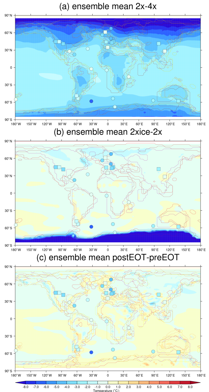
Figure 7. Ensemble mean modelled SAT response to (a) \text{CO}_2 halving ( \Delta T_{\text{CO}_2} ), (b) onset of ice on Antarctica ( \Delta T_{\text{ICE}} ) and (c) palaeogeographic change ( \Delta T_{\text{GEO}} ) across the EOT. The continental outlines for all models in each ensemble are shown. The marine proxy data are shown as filled circles, while the terrestrial proxy data are shown as filled squares.
