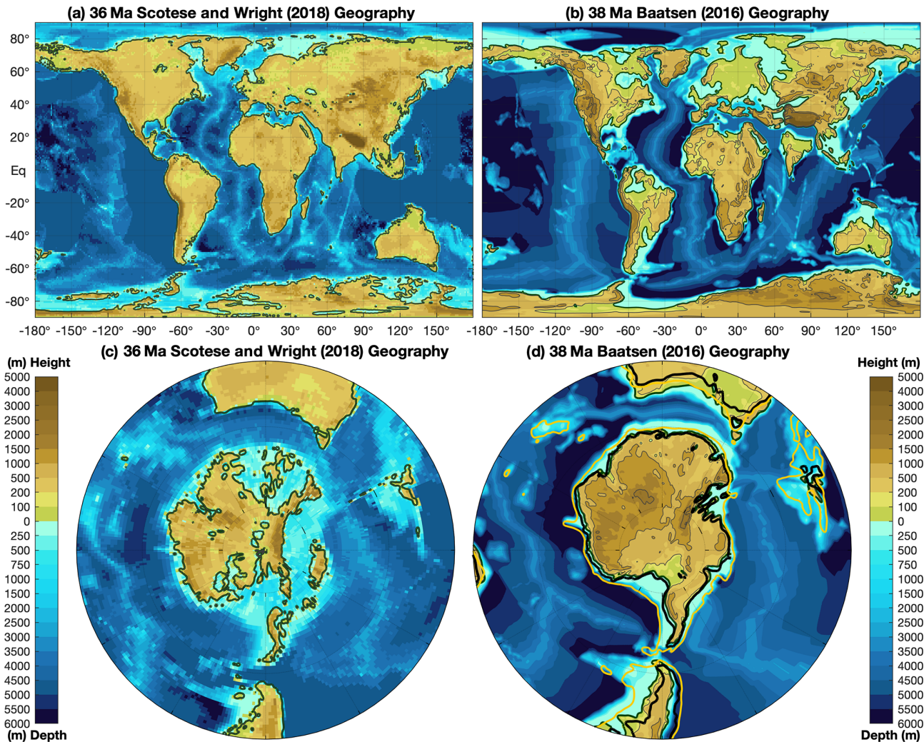
Figure 2. Palaeogeography in the late Eocene showing two alternative reconstructions. Panels (a) and (c) use the hot spot reference frame, using the Scotese and Wright (2018) palaeogeography at 36 Ma, while panels (b) and (d) use the palaeomagnetic reference frame showing the reconstruction of Baatsen et al. (2016) at 38 Ma. These two reconstructions use different methodologies and are presented as broadly indicative of the uncertainties in palaeogeography at this time. Also shown in panel (d) are post-EOT coastlines at 30 Ma (black contours) and 1000 m depth (orange contours), which illustrate the widening of the Southern Ocean gateways during the 8 Myr interval around the EOT.
