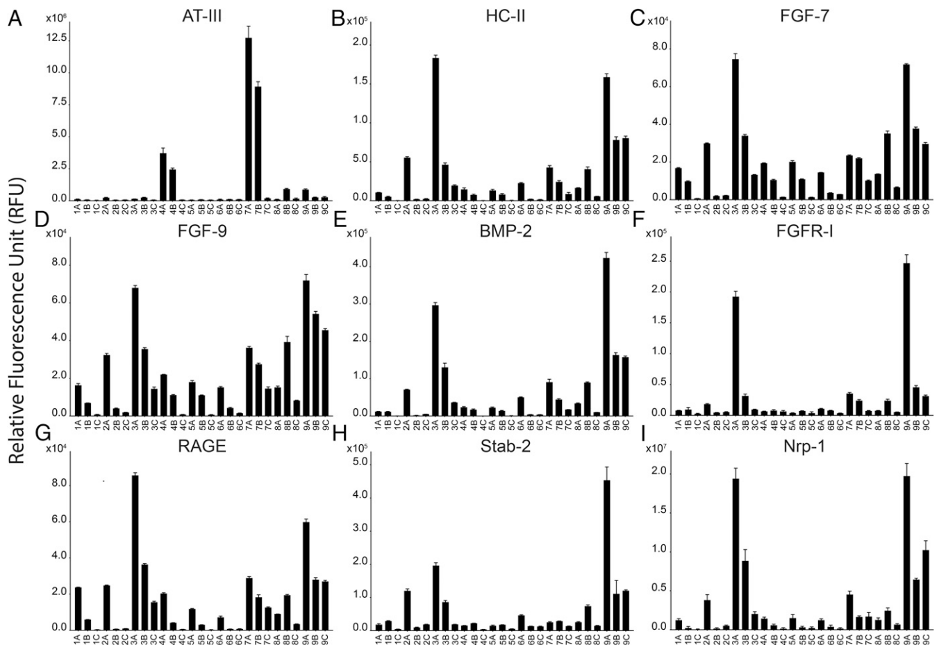
Fig. 4. Screening various HS recognizing proteins for their binding against an array of synthetic hexasaccharides printed at 100 \mu\text{M} concentration in a replicate of six. (A) AT-III/Human serpinC1 (10 \mu\text{g}/\text{mL} ). (B) HC-II/Human serpinD1 (3 \mu\text{g}/\text{mL} ). (C) Human FGF-7 (0.3 \mu\text{g}/\text{mL} ). (D) Human FGF-9 (0.1 \mu\text{g}/\text{mL} ). (E) Human BMP-2 (1 \mu\text{g}/\text{mL} ). (F) Human FGFR-1/CD331 (10 \mu\text{g}/\text{mL} ). (G) RAGEWRAGE RAGE/advanced glycosylation end product AGER (1 \mu\text{g}/\text{mL} ). (H) Human stabilin-2/Stab-2 (30 \mu\text{g}/\text{mL} ). (I) Mouse Nrp-1 (30 \mu\text{g}/\text{mL} ). List of protein source (type of fusion tag, if present), primary antibodies, and secondary antibodies (type of fluorophore, if present) screened against HS microarray are presented in SI Appendix, Table S1 . For dose–response of various HS recognizing protein screened for their binding to HS microarray, see SI Appendix Fig. S2 . Data are presented as mean \pm SD ( n = 4 ). Representative data are shown for each protein, which was repeated at least three times.
