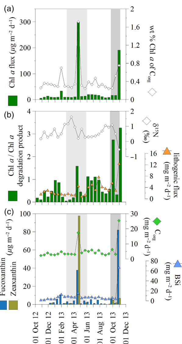
Fig. 8. Phytoplankton pigment content at M4U: (a) fluxes of total Chl a (bars) and relative weight % of Chl a fluxes to \text{C}_{\text{org}} (diamonds), (b) Chl a/Chl a degradation product ratio (bars), \delta^{15}\text{N} values (diamonds) and lithogenic flux (triangles), (c) fluxes of fucoxanthin and zeaxanthin (bars), organic carbon (diamonds) and fluxes of biogenic silica (triangles).
