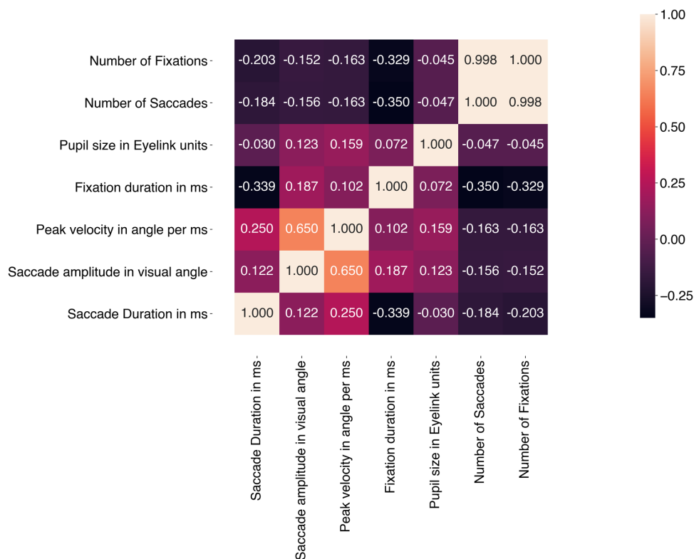
Figure 4. Correlation matrix of base feature measurements.
