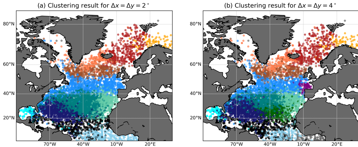
Figure C2. Clustering of Q for the drifter data set and different bin sizes, with trajectory lengths restricted to 1 year, 20 clusters as in Fig. 6, plotted at initial time and the drifter release location. (a) \Delta x = \Delta y = 2^\circ . (b) \Delta x = \Delta y = 4^\circ . The main features of Fig. 6 are still visible, although some structures change: the Bay of Biscay is not detected in (a) , and the structure of the clusters in the centre of the Subtropical Gyre change compared to Fig. 6. There are also new clusters in black (a, b) and dark green (b) . Note that the main features of the North Atlantic Ocean, such as the Subtropical–Subpolar Gyre boundary, the Western Boundary Current region, the Caribbean Sea and the Nordic Seas, are still detected; see the result in Fig. 6.
