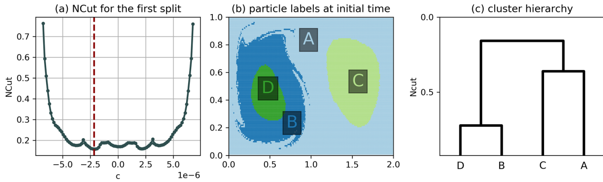
Figure B6. Hierarchical clustering result of the double gyre using algorithm 2 of Sect. 3.3 and \Delta x = \Delta y = 0.1 . (a) Ncut for the first split as a function of the cutoff c , where c = 0 corresponds to a cut along the transport boundary, the red line indicating the minimum found by our algorithm. (b) Result of the hierarchical clustering. (c) Dendrogram representing the hierarchy, where the horizontal lines correspond to the Ncut value after each split. There is only a local minimum at c = 0 , which is why the transport boundary is still not detected. This situation is similar to the one described by Froyland and Padberg (2009) for the transfer operator framework.
