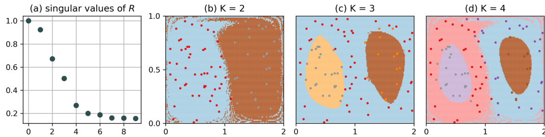
Figure 5. Clustering of \mathbf{Q} for the incomplete data set, where 500 particles are retained and 80 % of the data points subsequently deleted. (a) Singular values of \mathbf{R} for the incomplete data set, with \Delta x = \Delta y = 0.4 . (b–d) Points representing the initial position of those particles that have data at initial time. Background: result for the full trajectory with \Delta x = \Delta y = 0.04 (cf. Fig. 3).
