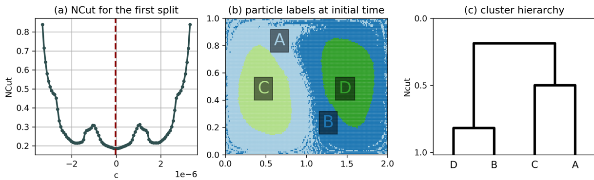
Figure B7. Hierarchical clustering result of the double gyre using algorithm 2 of Sect. 3.3 and \Delta x = \Delta y = 0.2 . (a) Ncut for the first split as a function of the cutoff c , where c = 0 corresponds to a cut along the transport boundary. (b) Result of the hierarchical clustering. (c) Dendrogram representing the hierarchy, where the horizontal lines correspond to the Ncut value after each split. There is a global minimum at c = 0 , so that the transport boundary is detected as the first split.
