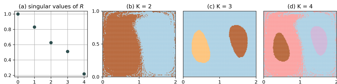
Figure 4. Clustering of \mathbf{Q} with \Delta x = 2/3 , \Delta y = 1/3 of the full data set, i.e. N = 20\,000 and \tau = 201 . The most dominant structure is still visible to high accuracy, although the problem is effectively nine-dimensional.
