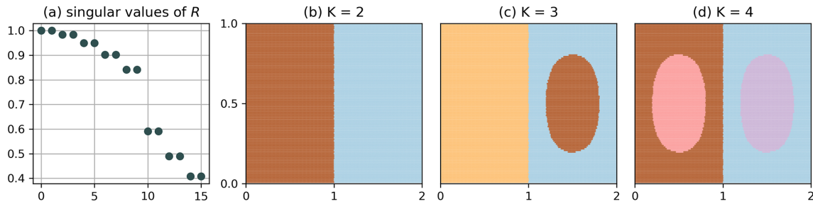
Figure B1. Clustering of \mathbf{Q} for the autonomous double gyre with \Delta x = \Delta y = 0.1 , i.e. an optimal partition, and the simultaneous K -way NCut (algorithm 1 in Sect. 3.3). The singular values are doubly degenerate as the network \mathbf{Q} consists of two disconnected sets.
