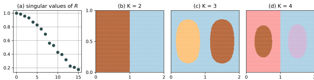
Figure B2. Clustering of \mathbf{Q} for the autonomous double gyre with \Delta x = \Delta y = 0.15 , i.e. a non-optimal partition, and the simultaneous K -way NCut (algorithm 1 in Sect. 3.3). The main separation at x = 1 is still resolved, but only at every even clustering step. The degeneracy of the singular values (see Fig. B1) is lifted.
