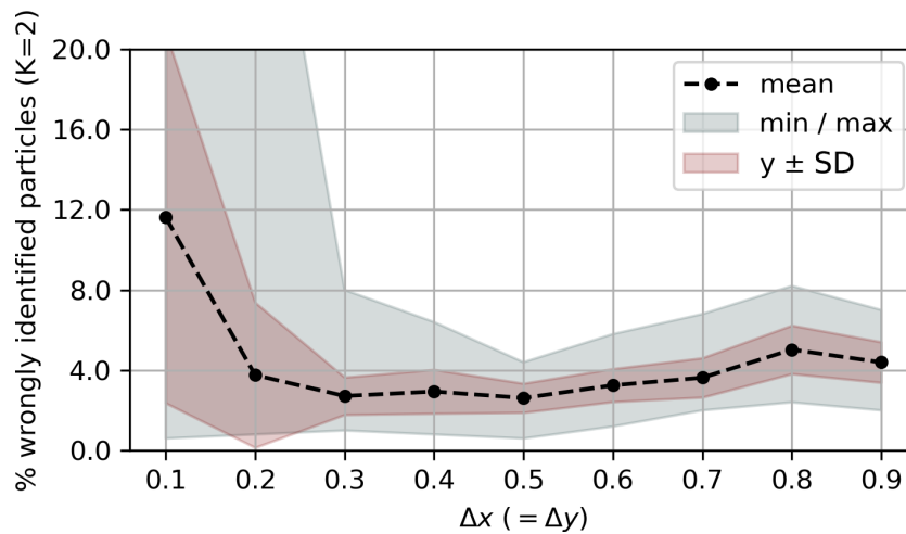
Figure B3. Share of incorrectly assigned particle labels for the double-gyre flow (simultaneous K -way clustering) for varying \Delta x = \Delta y , K = 2 and the incomplete ( N = 500 ) data set, compared to the baseline of the complete data set with \Delta x = \Delta y = 0.04 ; cf. Fig. 3. The values were obtained with 100 random incomplete data sets for each value of \Delta x (= \Delta y) . The filled areas show the minimum and maximum ranges, 1 standard deviation, and the points the corresponding means. It is visible that for too small bin spacing, the number of wrongly assigned labels is very high. This is most likely because the network becomes less connected, such that it is more difficult to find structure in the eigenvector corresponding to the second smallest eigenvalue of \mathbf{L}_s[\mathbf{Q}] . As explained in the main text, for bin sizes that do not exactly fit the domain, the x and y directions were artificially extended.
