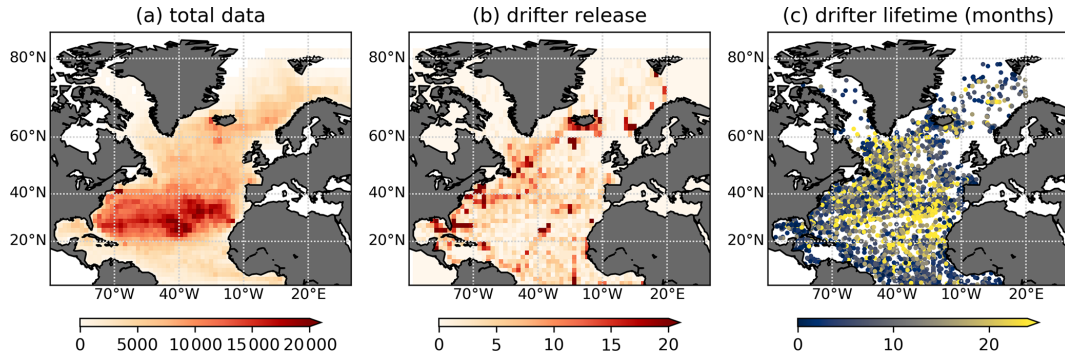
Figure 1. (a) Total counts of all drifter locations (6-hourly for each trajectory), computed with a binning of 2° in both longitude and latitude. (b) Distribution of drifter release per 2° bin. (c) Scatter plot of initial drifter location, the colour indicating the drifter lifetime in months.
