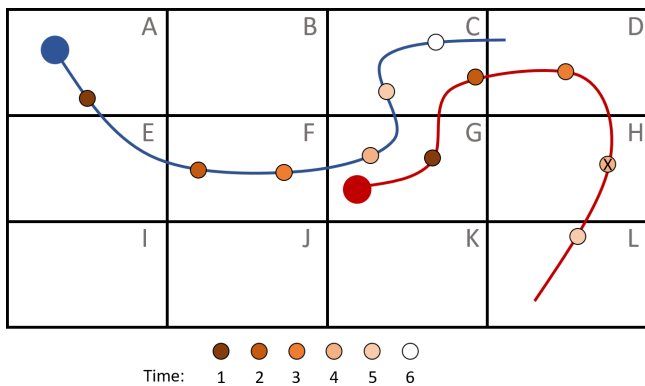
Figure 2. Two example trajectories on a binned fluid domain, with alphabet A, ..., L and \tau = 7 . The markers along the trajectories represent the points in time the location is stored. The itinerary for the blue particle is AAFFGCC. The red particle has itinerary GGCD_L_. Here, “_” denotes a missing data point, the one at time t = 4 , indicated by an “X” in the respective marker. The last data point of the red trajectory is also missing, as its lifetime is shorter than \tau time instances.
