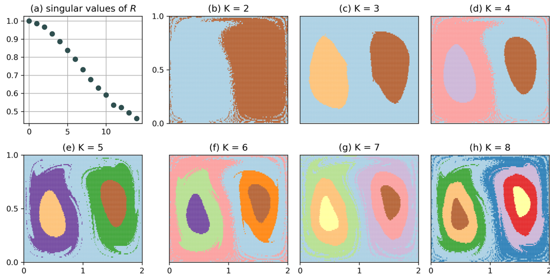
Figure 3. Clustering of \mathbf{Q} with \Delta x = \Delta y = 0.04 of the full data set, i.e. N = 20\,000 and \tau = 201 .
