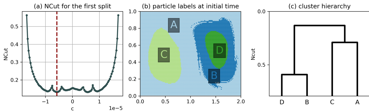
Figure B5. Hierarchical clustering result of the double gyre using algorithm 2 of Sect. 3.3 and \Delta x = \Delta y = 0.04 . (a) Ncut for the first split as a function of the cutoff c , where c = 0 corresponds to a cut along the transport boundary, the red line indicating the minimum found by our algorithm. (b) Result of the hierarchical clustering. (c) Dendrogram representing the hierarchy, where the horizontal lines correspond to the Ncut value after each split. There is no global or local minimum at c = 0 in (a) , which is why the transport boundary is not detected. Instead, two global minima are present in (a) , but our implementation selects the left minimum for the first split due to the choice of sampling points.
