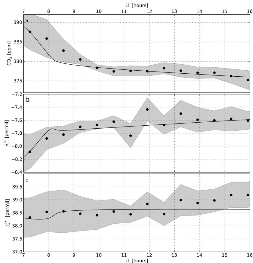
Fig. 4. Diurnal evolution of the (a) CO 2 , (b) δ a 13 and (c) δ a 18 . Treatment of observations and model results similar to Fig. 2.
