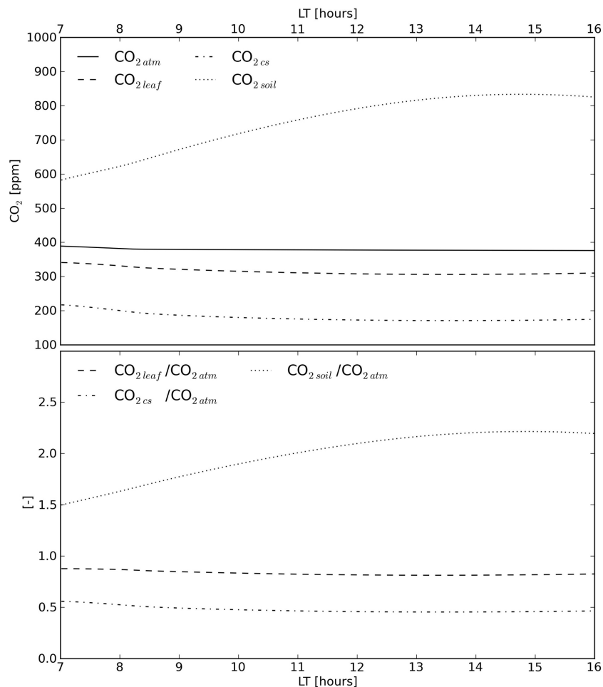
Fig. 6. Diurnal evolution of the CO 2 mixing ratio used in the plant and soil parameterizations: atmospheric mixed-layer, inner leaf ( c_{leaf} ), mesophyll ( c_{cs} ) and soil ( c_{soil} ) (a) and the ratio of the leaf, mesophyll and soil CO 2 with respect to the atmospheric value. Note that the atmospheric CO 2 mixing ratio evolution is the same as the one shown in Fig. 4a.
