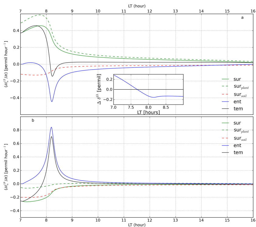
Fig. 10. Diurnal evolution of the contributions of the individual components of the total budget: (a) \delta^{13} according to Eq. (7) and (b) \delta^{18} . tem is the temporal term, surf is the surface contribution including the individual contributions by plants and soil processes and ent is the entrainment term. The inset figure in (a) shows the change of the sign of the \Delta\delta^{13} defined as the difference on the isotopic signature of \delta_u^{13} in the free troposphere and the mixed-layer value.
