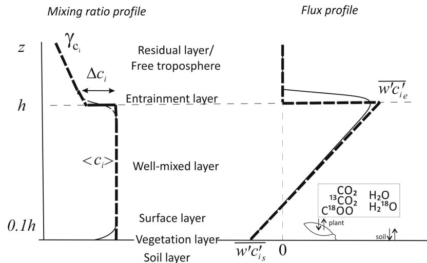
Fig. 1. Main processes governing the diurnal evolution of each stable isotopologue in an interactive atmosphere-land system. Surface flux exchanges ( \overline{w'c'_i}_s ) depend on the vegetation conditions (represented by the A-gs model and soil efflux). For the turbulent fluxes, a negative sign indicates an uptake of the compound c_i from the ABL by the plant or soil. In the mixed-layer, the mean profile (left) is constant with height and the flux profile is linear (right). The thin continuous lines indicate more realistic profile and the thick dashed line the profiles after mixed-layer assumptions are applied. The flux exchange at the interface between the residual layer/free troposphere and the atmospheric boundary layer is represented by an entrainment flux ( \overline{w'c'_i}_e ). In the mixed-layer model this entrainment flux is parameterized as a product of the ABL growth rate (entrainment velocity) and the stable isotope jump ( \Delta c_i ). This jump depends on the lapse rate ( \gamma_{c_i} in the residual or free tropospheric layers). Note that large scale forcings like advection ( Adv(c_i) ) and mean vertical velocity subsidence influencing h are not included in the figure, but they can be prescribed in the numerical experiments.
