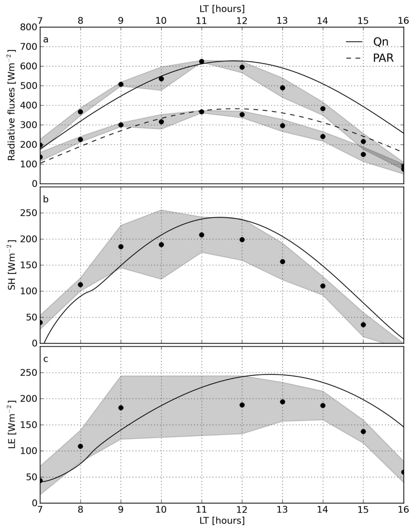
Fig. 2. Diurnal evolution of the (a) net available energy and photosynthetic active radiation, (b) sensible and (c) latent heat fluxes. The observations are aggregated of four consecutive days under similar conditions (16–19th September 2011). Averaged values are shown as dots and the shaded region represents the standard deviations. MXL results are expressed by continuous and dashed lines. Observations were taken above the canopy, at 27.9 m above ground level. For LE, the observations at 10 and 11 LT were missing for the four successive days.
