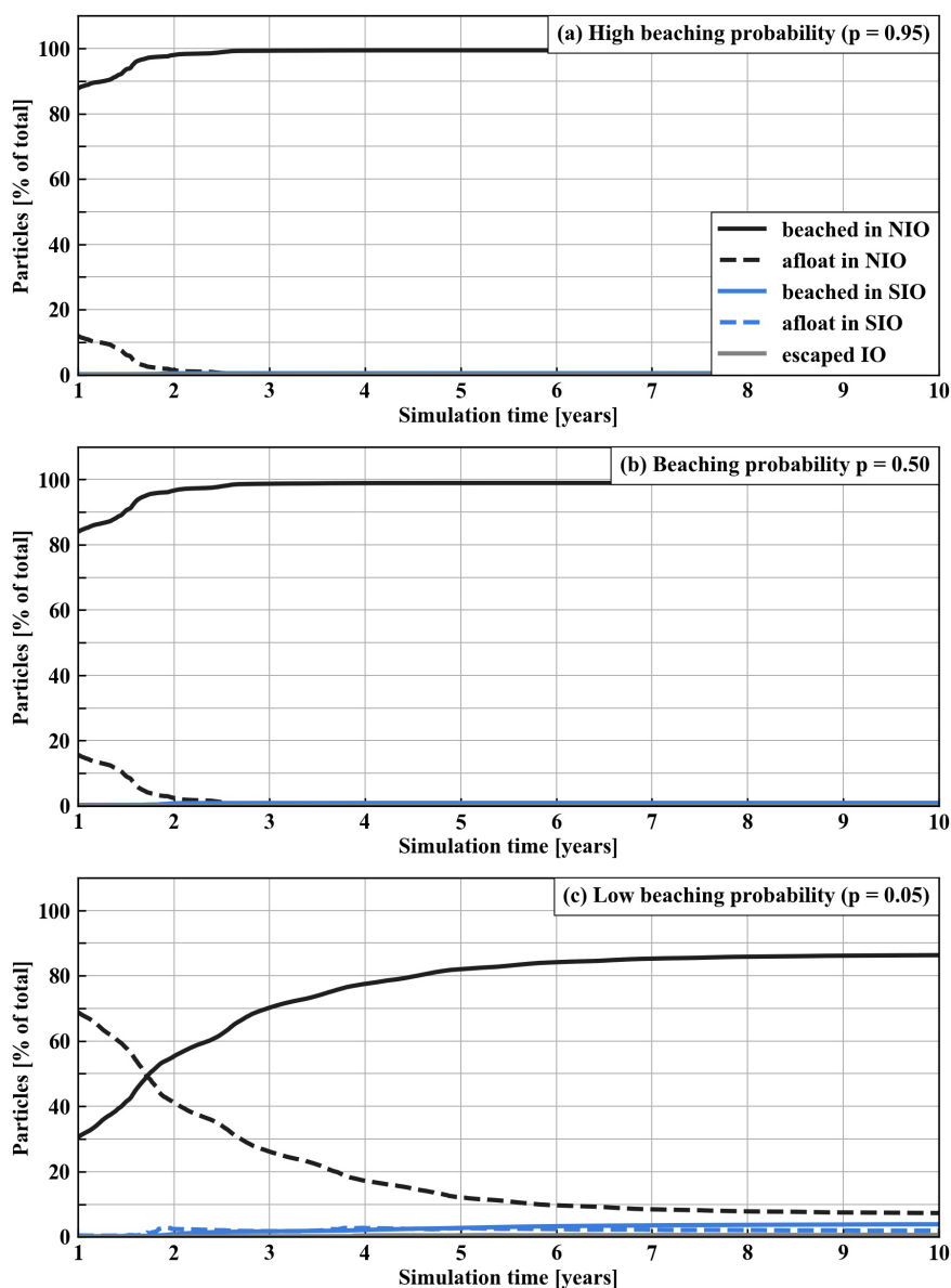
Figure 4. Percentage of total simulated particles as a function of the simulation duration that have beached in the Northern Hemisphere (NIO) or Southern Hemisphere Indian Ocean (SIO), are afloat in the NIO or SIO, or have left the Indian Ocean entirely under (a) a high beaching probability of p = 0.95 (5 \text{ d})^{-1} , (b) a beaching probability of p = 0.50 (5 \text{ d})^{-1} , and (c) a low beaching probability of p = 0.05 (5 \text{ d})^{-1} . Percentages are shown after all particles have been released after 1 year of simulation, and up to 10 years of simulation, after which the simulation results have reached a steady state in all cases.
