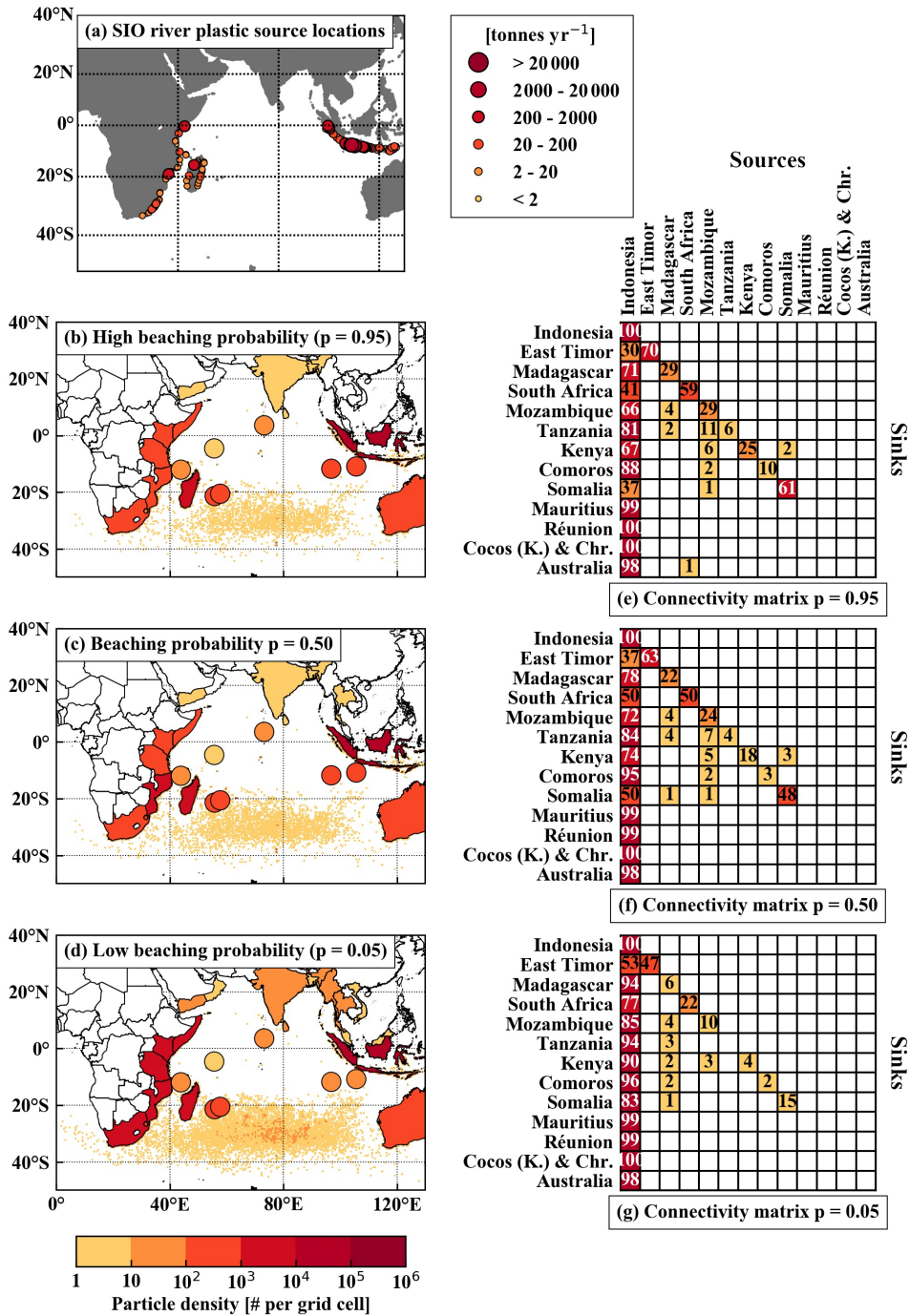
Figure 6. (a) Locations of plastic waste input from rivers in the Southern Hemisphere Indian Ocean based on Lebreton et al. (2017). Density of beached particles per country or island and density of particles in the ocean per 0.5^\circ \times 0.5^\circ grid cell for particles released from river source locations in the Southern Hemisphere Indian Ocean after 21 years of simulation, with (b) a high beaching probability, i.e. p = 0.95 (5 \text{ d})^{-1} (10-year animation of simulation results available at https://doi.org/10.5446/47058 , van der Mheen et al., 2020c); (c) a beaching probability of p = 0.50 (5 \text{ d})^{-1} (10-year animation of simulation results available at https://doi.org/10.5446/47057 , van der Mheen et al., 2020b); and (d) a low beaching probability, i.e. p = 0.05 (5 \text{ d})^{-1} (10-year animation of simulation results available at https://doi.org/10.5446/47056 , van der Mheen et al., 2020a). Filled circles highlight islands that do not clearly show up on the map otherwise, from north to south these represent: the Maldives, Seychelles, the British Indian Ocean Territory, Christmas Island, Cocos (Keeling) Islands, Comoros, Mauritius, and Réunion. Connectivity matrices showing the percentage of particles that beach in selected countries (rows) against countries of origin (columns) for (e) a high beaching probability, i.e. p = 0.95 (5 \text{ d})^{-1} ; (f) a beaching probability of p = 0.50 (5 \text{ d})^{-1} ; and (g) a low beaching probability, i.e. p = 0.05 (5 \text{ d})^{-1} . Note that the sum of each row does not always precisely equal 100 % because not all countries with river plastic sources are shown, percentages are rounded to integer numbers, and percentages below 1 % are omitted.
