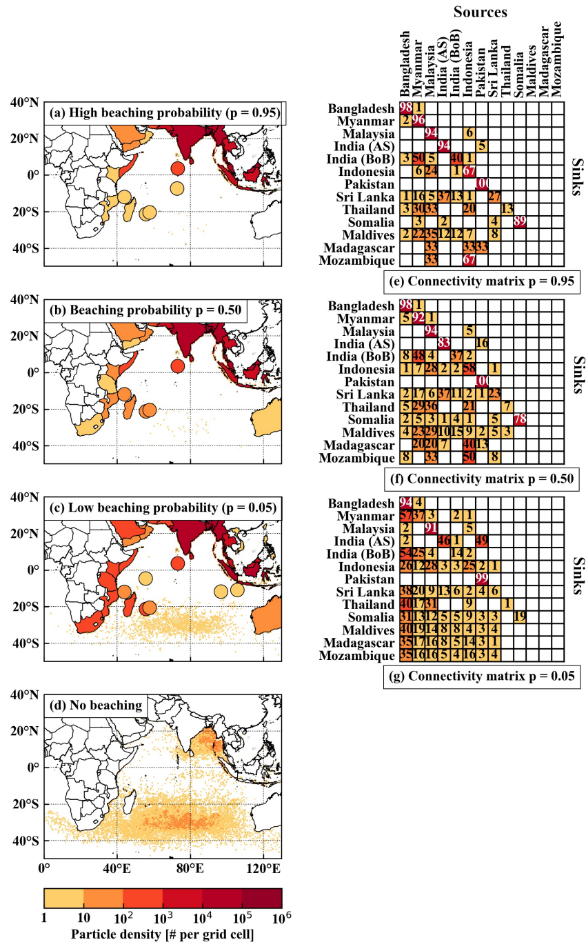
Figure 5. Density of beached particles per country or island and density of particles in the ocean per 0.5^\circ \times 0.5^\circ grid cell for particles released from river source locations in the Northern Hemisphere Indian Ocean after 21 years of simulation, with (a) a high beaching probability, i.e. p = 0.95 (5 \text{ d})^{-1} (10-year animation of simulation results available at https://doi.org/10.5446/47058 , van der Mheen et al., 2020c); (b) a beaching probability of p = 0.50 (5 \text{ d})^{-1} (10-year animation of simulation results available at https://doi.org/10.5446/47057 , van der Mheen et al., 2020b); (c) a low beaching probability, i.e. p = 0.05 (5 \text{ d})^{-1} (10-year animation of simulation results available at https://doi.org/10.5446/47056 , van der Mheen et al., 2020a); and (d) no beaching. Filled circles highlight islands that do not clearly show up on the map otherwise, from north to south these represent: the Maldives, Seychelles, the British Indian Ocean Territory, Christmas Island, Cocos (Keeling) Islands, Comoros, Mauritius, and Réunion. Connectivity matrices showing the percentage of particles that beach in selected countries (rows) against countries of origin (columns), for (e) a high beaching probability, i.e. p = 0.95 (5 \text{ d})^{-1} ; (f) a beaching probability of p = 0.50 (5 \text{ d})^{-1} ; and (g) a low beaching probability, i.e. p = 0.05 (5 \text{ d})^{-1} . In these matrices, India is split into a western side bordering the Arabian Sea, i.e. “India (AS)”, and an eastern side bordering the Bay of Bengal, i.e. “India (BoB)”. Note that the sum of each row does not always precisely equal 100 % because not all countries with river plastic sources are shown, percentages are rounded to integer numbers, and percentages below 1 % are omitted.
