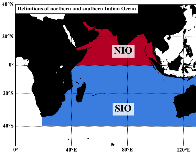
Figure A1. Definition of the Northern Hemisphere Indian Ocean (NIO) and Southern Hemisphere Indian Ocean (SIO). We use these definitions to select release locations of particles from the NIO only and to determine the fate of particles during the simulation (e.g. beached or floating in the NIO or SIO).
