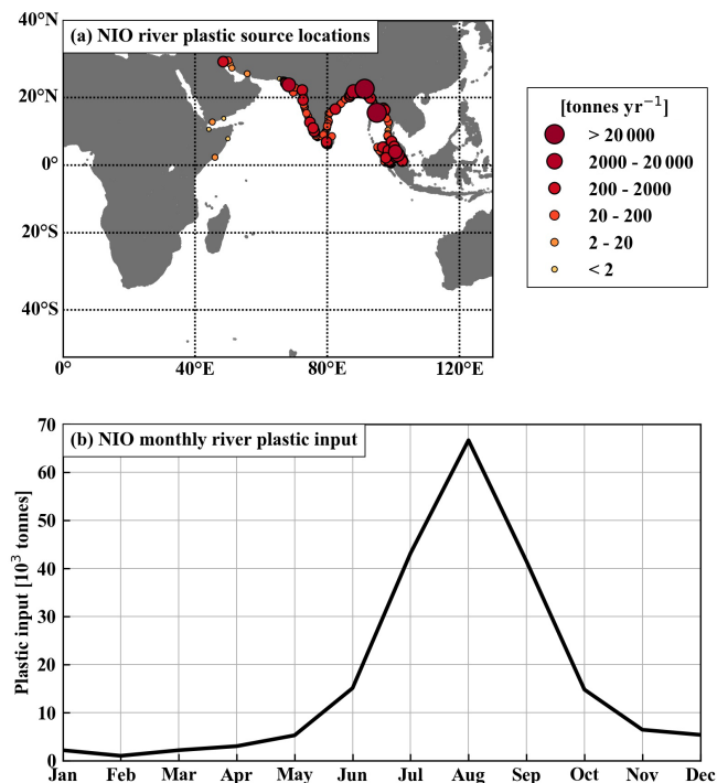
Figure 2. (a) Locations of plastic waste input from rivers in the Northern Hemisphere Indian Ocean based on Lebreton et al. (2017). We release particles from these locations in our particle-tracking simulations (Sect. 2.2). (b) Total plastic waste input in the Northern Hemisphere Indian Ocean for each month. Lebreton et al. (2017) based the monthly variation of plastic input on seasonal variations in river discharges. We release particles following this monthly variation in our particle-tracking simulations, where 1 particle represents 1 t of plastic waste (Sect. 2.2).
