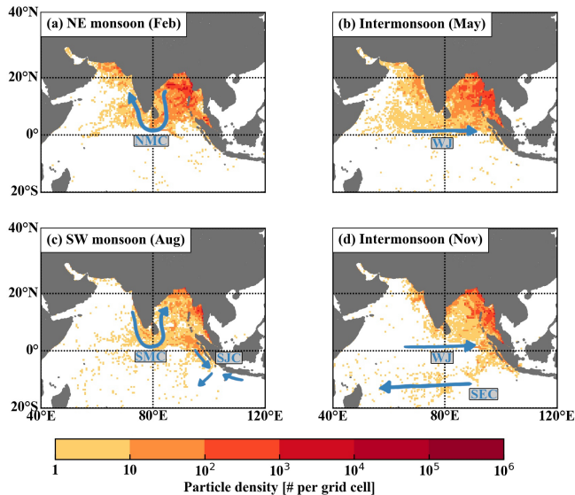
Figure 3. Particle density of simulated particles released from river source locations in the Northern Hemisphere Indian Ocean during neutral Indian Ocean Dipole conditions and without beaching at the end of (a) the northeast monsoon season (February), (b) the intermonsoon period transitioning from the northeast to the southwest monsoon (May), (c) the southwest monsoon season (August), and (d) the intermonsoon period transitioning from the southwest to the northeast monsoon (November). Blue arrows indicate relevant ocean surface currents labelled with their abbreviations: Northeast Monsoon Current (NMC), Wyrki jets (WJ), Southwest Monsoon Current (SMC), South Java Current (SJC), and South Equatorial Current (SEC).
