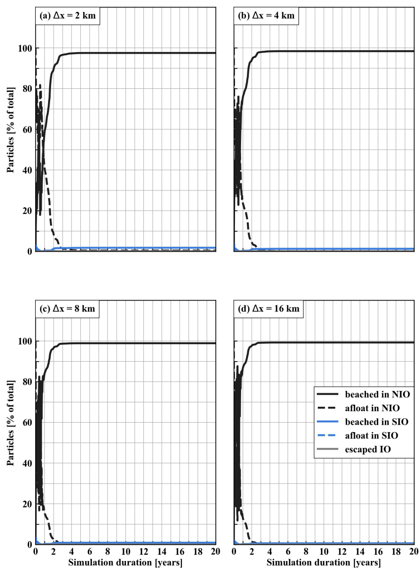
Figure A5. Sensitivity analysis results where beaching occurs with a probability p = 0.50 (5 \text{ d})^{-1} for particles within a distance \Delta x = [2, 4, 8, 16, 32] km to the nearest coastline that are moving towards the coast. Results are not very sensitive to different values for \Delta x , and we use \Delta x = 8 km as the default value in further simulations.
