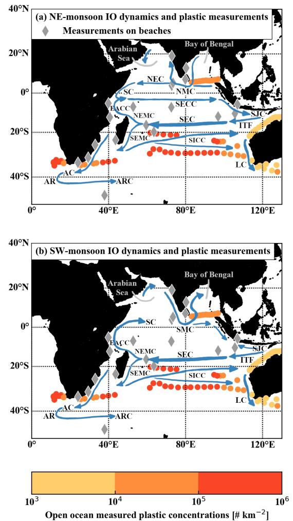
Figure 1. Overview of standardized open-ocean plastic measurements in the Indian Ocean (filled circles), approximate locations of sampling studies of plastics on beaches (grey diamonds), and schematic dominant ocean surface currents (blue arrows) during the (a) northeast monsoon season and (b) southwest monsoon season. Open-ocean sampling studies were performed by Morris (1980), Reisser et al. (2013), Eriksen et al. (2014), and C3zar et al. (2014) and standardized by van Sebille et al. (2015). Sampling studies of plastics on beaches were performed by Ryan (1987), Slip and Burton (1991), Madzena and Lasiak (1997), Unepetty and Evans (1997), Barnes (2004), Jayasiri et al. (2013), Duhec et al. (2015), Nel and Froneman (2015), Bouwman et al. (2016), Kumar et al. (2016), Imhof et al. (2017), and Lavers et al. (2019). Schematic ocean surface currents are based on Schott et al. (2009). The following currents are shown and labelled with their abbreviations: Northeast Monsoon Current (NMC) and Southwest Monsoon Current (SMC), North Equatorial Current (NEC), Somali Current (SC), South Equatorial Countercurrent (SECC), South Java Current (SJC), East African Coastal Current (EACC), Indonesian Throughflow (ITF), Northeast Madagascar Current (NEMC), Southeast Madagascar Current (SEMC), Agulhas Current (AC), Agulhas Retroreflection (AR), Agulhas Return Current (ARC), South Indian Countercurrent (SICC), Leeuwin Current (LC).
