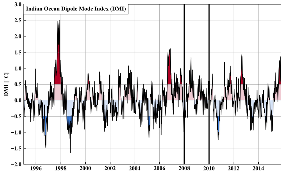
Figure A3. Indian Ocean Dipole Mode Index (DMI) as defined by Saji et al. (1999) and obtained from the National Oceanic and Atmospheric Administration. Red and blue shading indicate positive and negative modes of the Indian Ocean Dipole (IOD), respectively. We use 2008 and 2009 (marked between thick vertical black lines) as neutral IOD years to simulate the influence of monsoon seasons on the transport of plastics in the Indian Ocean.
