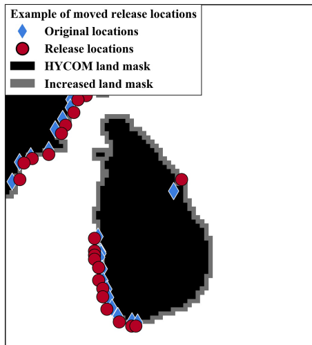
Figure A2. Example of original river source locations estimated by Lebreton et al. (2017) and moved release locations in relation to the HYCOM land mask around Sri Lanka. Release locations are shifted compared to original source locations where necessary to prevent particles from being released on or too close to land in particle-tracking simulations.
