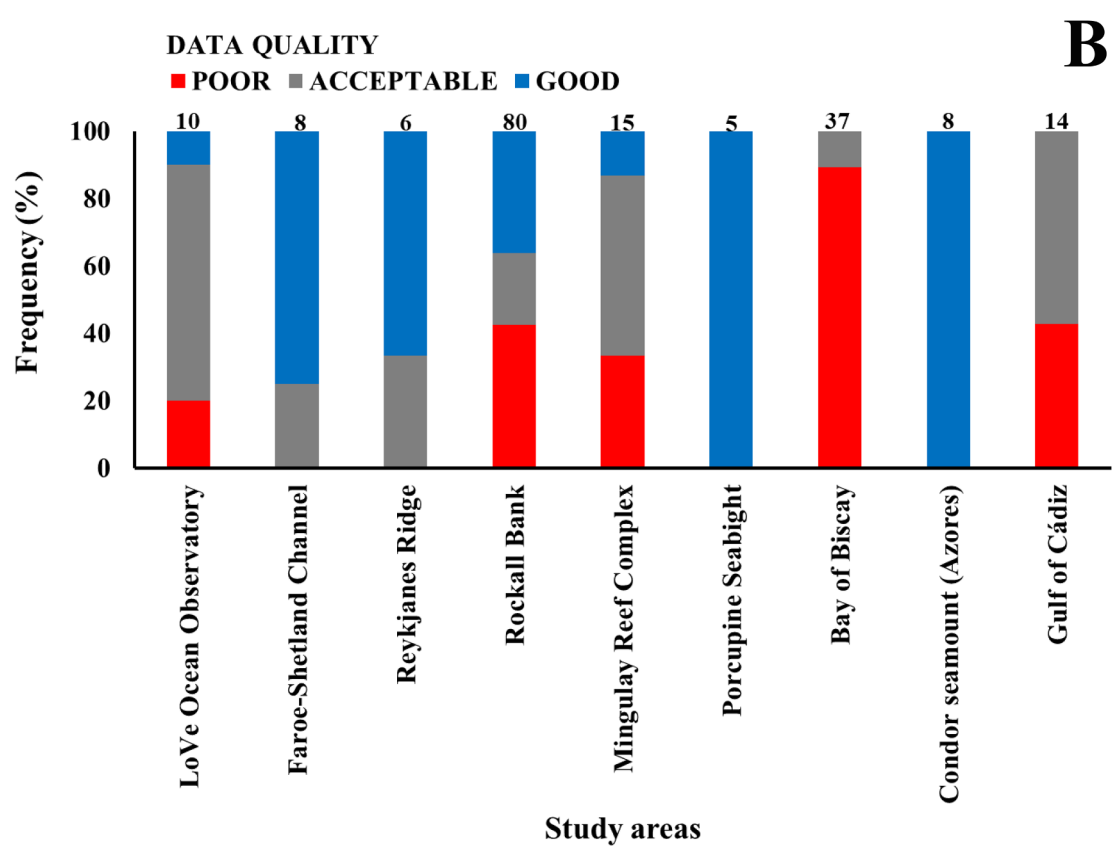
Fig. 5. Data quality (“poor”, “acceptable” and “good”) expressed in % across indicators and descriptors (A) and across study areas (B). In (A) each number on the x axis represents an indicator (see Table 3 for the corresponding indicator name). In (B) the number of indicator values in each study area is shown on the top of the bars.
