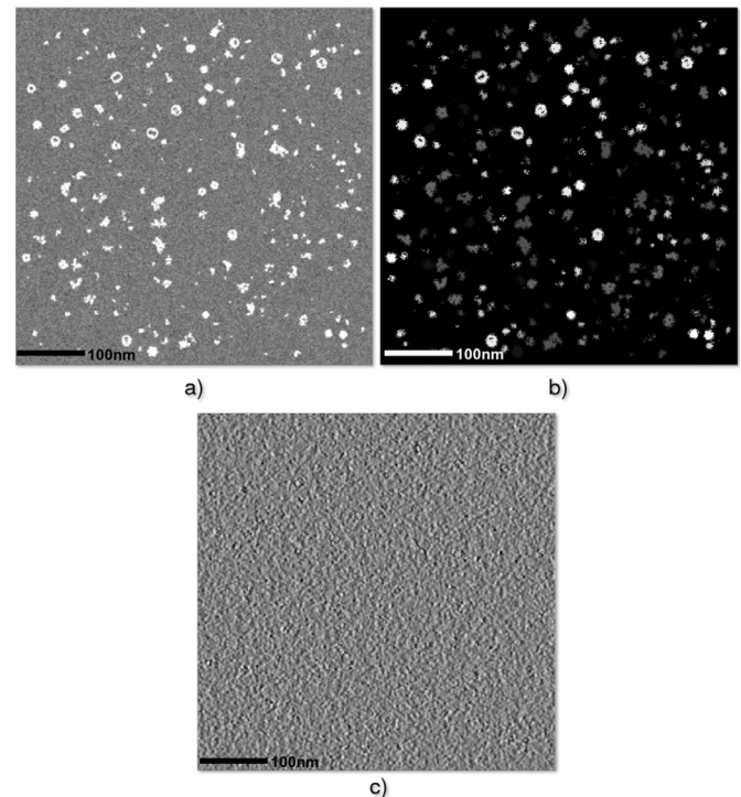
Fig. 3. Central slice of tomogram #1 in the generated dataset: (a) ground truth volume of the sample that was used for reconstruction, (b) class mask, where each voxel is annotated by class, (c) tomographic reconstruction
