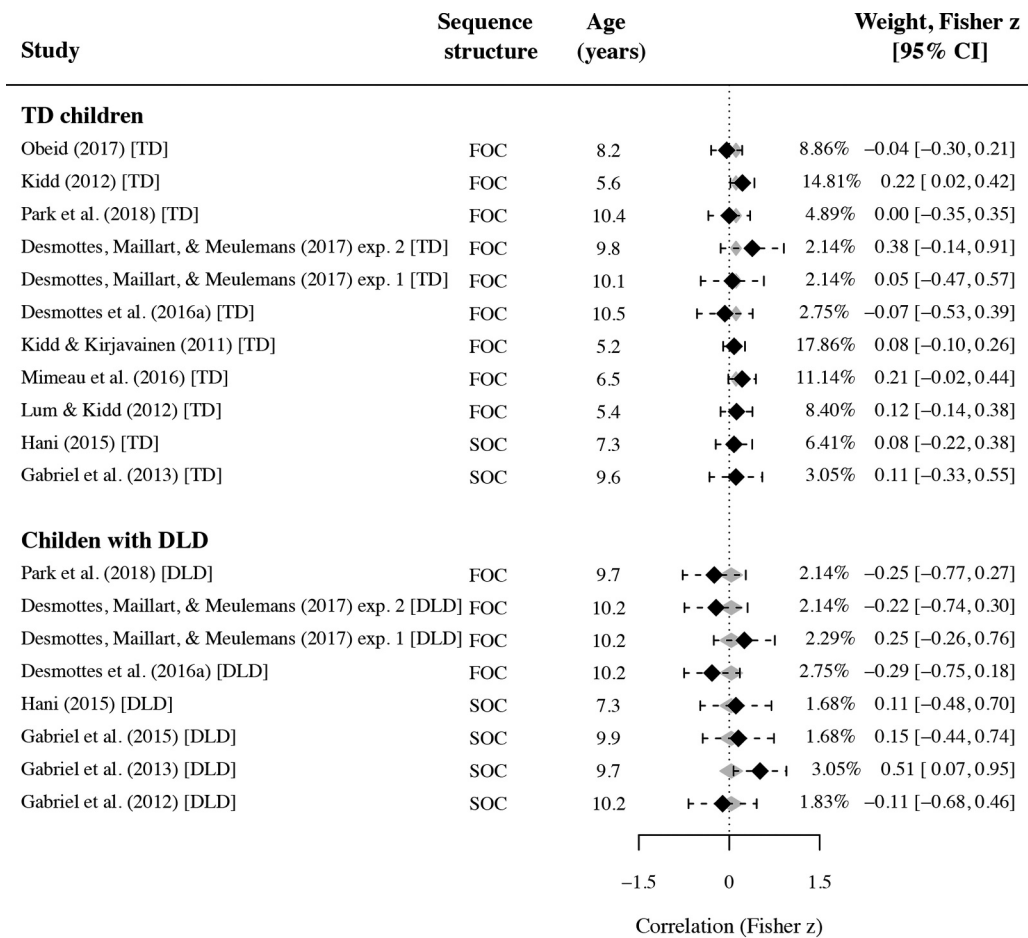
Figure 5. Forest plot showing overall and individual mean weighed effect sizes (Fisher z), divided per group. The shaded diamonds represent the mean weighed effect size per group (DLD or typically developing). FOC = first order conditional; SOC = second order conditional.
