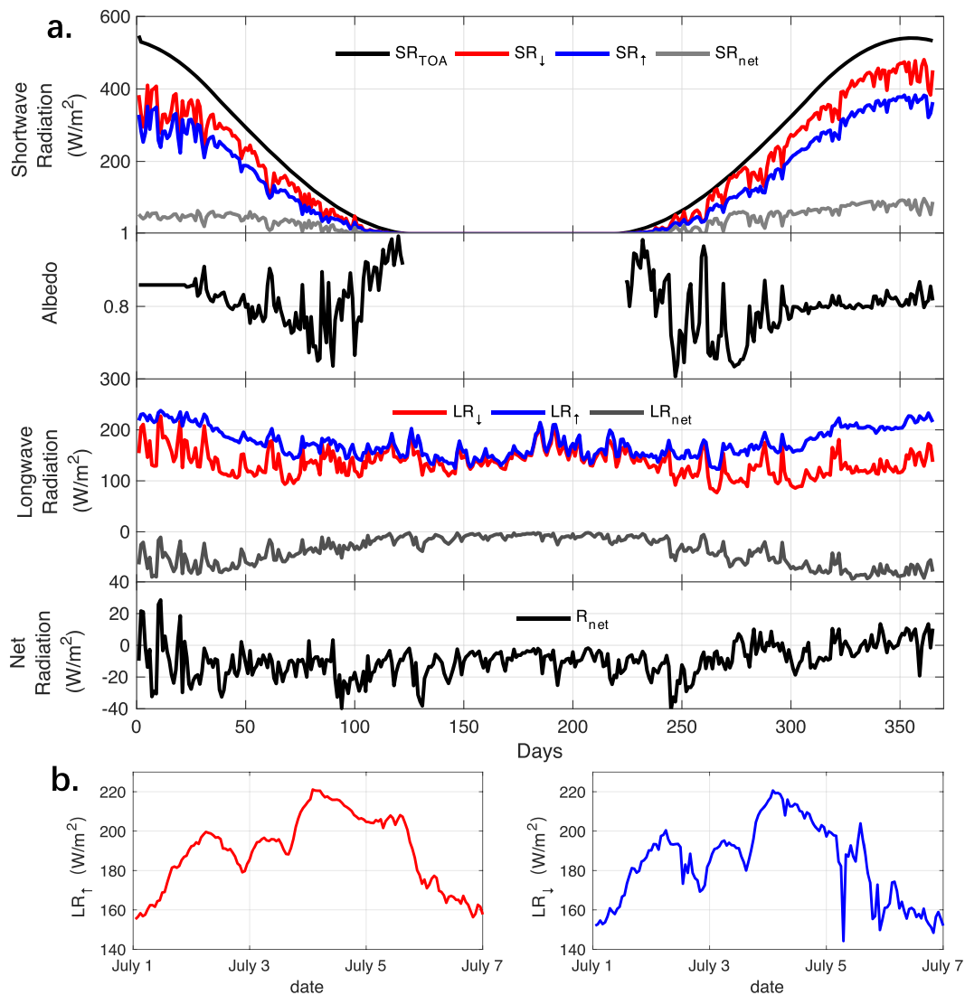
Figure 4. (a) Daily mean values of incident and reflected shortwave radiation, downward and upward longwave radiation, albedo, and net radiation. (b) Hourly means of LR ↑ and LR ↓ during one intrusion event in July 2011.
