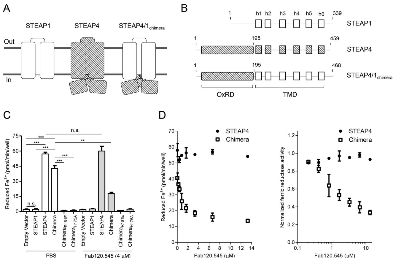
Figure 5. Cellular ferric reductase activity of STEAP protein variants. A , schematic topological representation of naturally occurring STEAP1 and STEAP4 and the designed fusion protein STEAP4/1 chimera . Domains of STEAP1 are shown in solid white , whereas STEAP4 domains are depicted in diagonal stripes . B , domain composition of STEAP1, STEAP4, and STEAP4/1 chimera constructs used for cellular ferric reductase experiments. C , cell-surface ferric reductase activity of STEAP protein variants supplemented with PBS or with 4 μM Fab120.545. The experiment was performed in triplicate, and error bars represent the S.D. D , cell-surface ferric reductase activity of STEAP4 and STEAP4/1 chimera with different concentrations of added Fab120.545. Error bars represent the S.D. from triplicate experiments. The right panel shows the same data normalized to an activity of 1 at 0 μM Fab120.545, with a logarithmic x axis .
