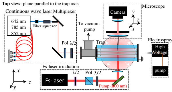
Fig. 1. Schematic of the top view of the experimental setup.
