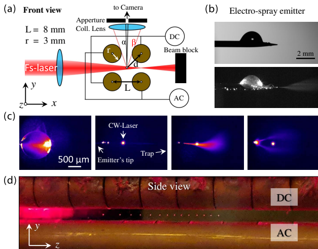
Fig. 2. (a) Schematic of the front view of the experimental setup. (b) Transmission (top) and dark field (bottom) microscopy images of the electro-spray emitter. (c) Dark field microscopy images of the electro-spray cone geometries. (d) Picture of the side view of the trap with gold nanoparticles.
