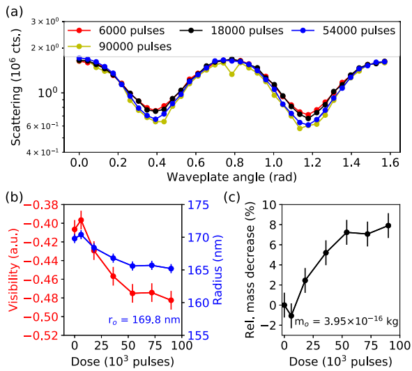
Fig. 5. (a) Experimental polarimetry curves at 785 nm of a single trapped gold nanoparticle after several fs-laser pulse exposures. This nanoparticle is the same one whose size characterization is presented in Fig. 4. Note that we set a logarithmic scale to stress the relative change of the curves. (b) Experimental visibility and radius as a function of the fs-laser dose. (c) Relative mass decrease in percentage as a function of the fs-laser pulse dose. The insets r_0 and m_0 indicate the radius and mass of the nanoparticle prior to laser exposure.
