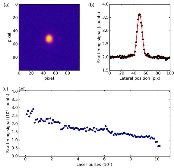
Fig. 3. (a) False color image of the scattered intensity (at 800 nm) of a single gold nanoparticle. (b) Integrated scattering intensity of the image in (a). (c) Fs-laser scattering signal of a single trapped nanoparticle as a function of the number of consecutive pulse exposures.
