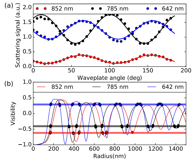
Fig. 4. (a) Graph of the polarimetry measurements performed using three different cw-laser wavelengths. The solid lines are fits using a sine function. (b) Visibility of gold nanoparticles as a function of the radius at three different wavelengths. The visibility curves were calculated using Mie theory. The horizontal lines show the experimental visibilities extracted from the fits in (a) using Eq. (4), and the circles illustrate the intersections with the Mie calculations.
