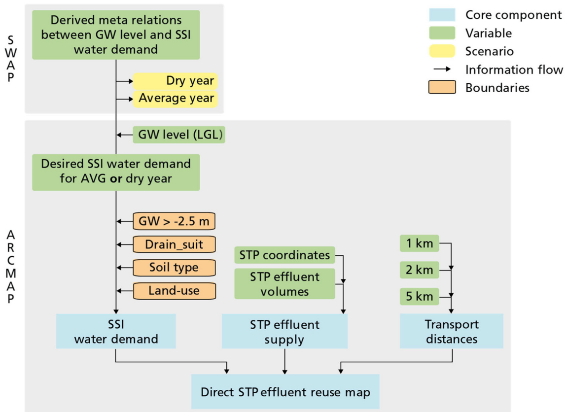
Fig. 1. Workflow for the creation of a direct STP effluent reuse through SSI map. Core components are the building blocks for the creation of this map, variables are prone to change over time, scenarios refer to the weather conditions, boundaries implicate the suitability of Dutch croplands for SSI.
