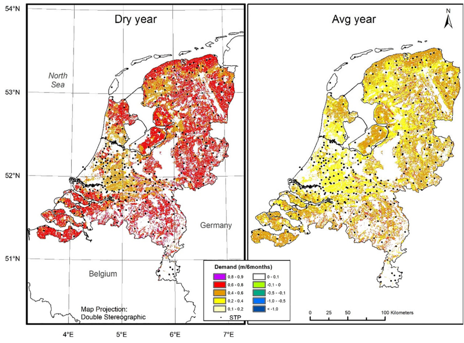
Fig. 2. SSI water demand [m] per 25m grid cell for SSI suitable croplands.
