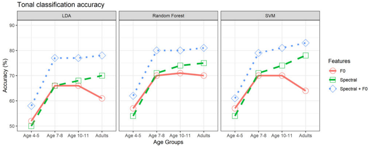
Figure 2. Tonal classification accuracy (chance level: 25%)
