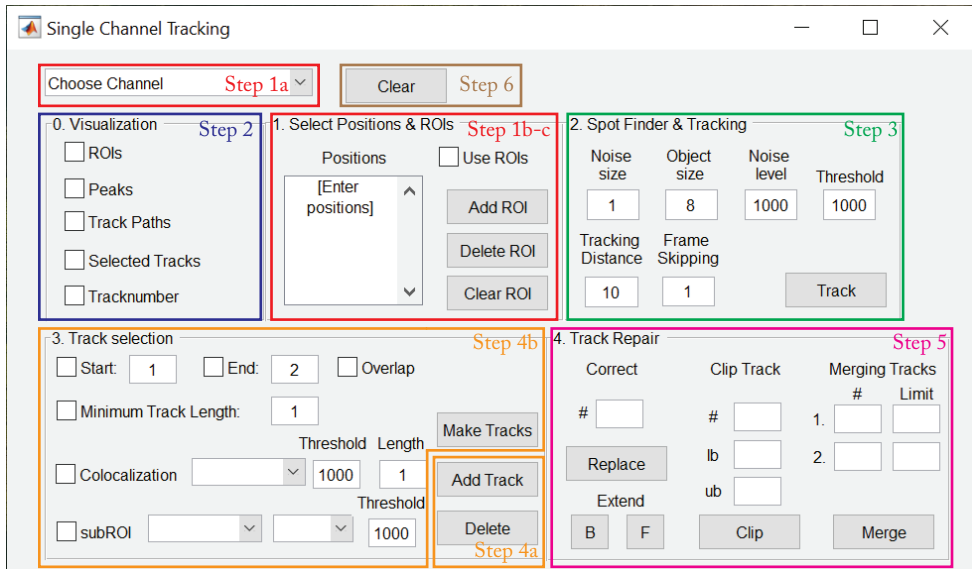
Fig. 5 | Screenshot of TransTrack 'analysis' window.
