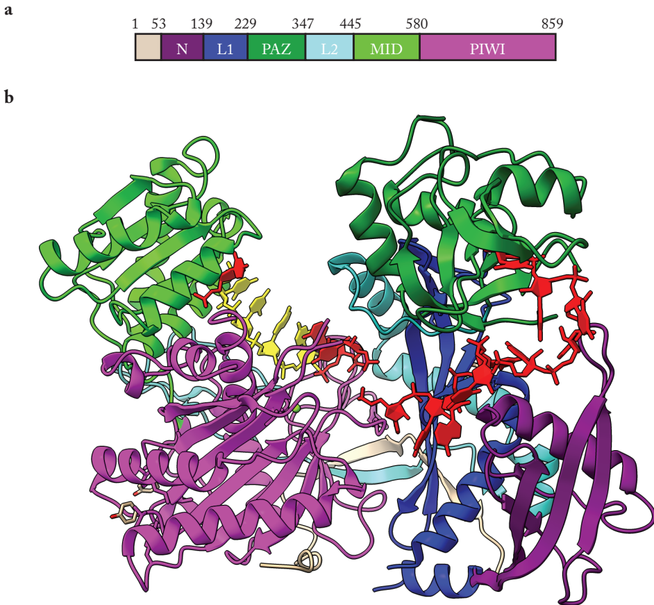
Fig. 3 | Crystal structure of AGO2 loaded with a gRNA.
