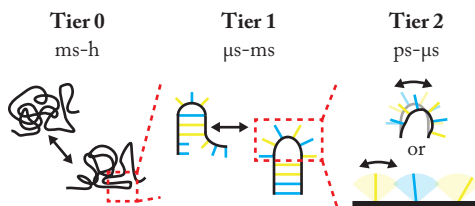
Fig. 6 | RNA structure dynamics at different time scales.
