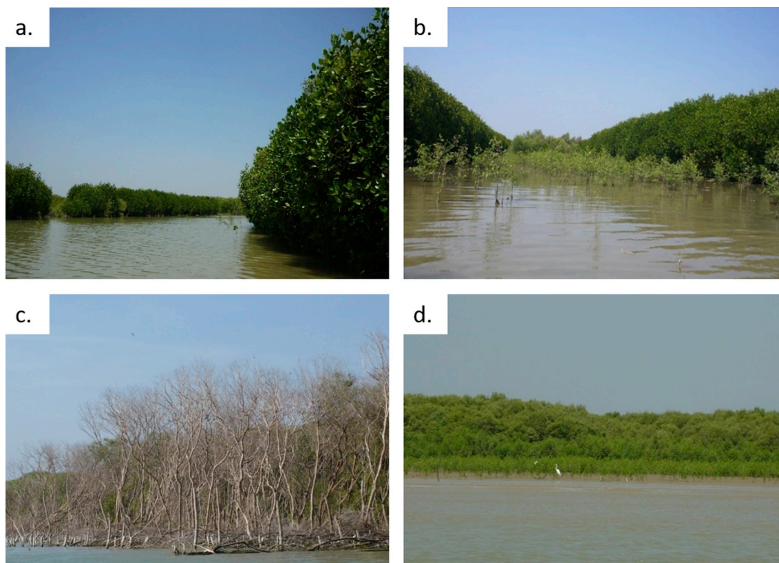
Fig. 3. Examples of mangrove retreat and recruitment in Demak (photos by Celine E. J. van Bijsterveldt). a. Abandoned aquaculture pond with little recruitment. b. Sheltered pond landward of a mangrove stand with Avicennia marina recruitment inside the pond and planted Rhizophora mucronata trees outlining the old pond bunds. c. Mangrove retreat at the sea side of a mangrove stand. d. Mangrove recruitment seaward of a mangrove stand. Three subsequent stages of mangrove recruitment are visible.
