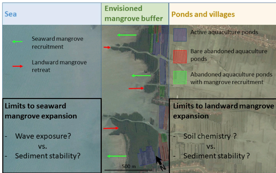
Fig. 2. Envisioned mangrove greenbelt buffer along the eroding aquaculture coastline of Demak, Java, Indonesia. Natural expansion of existing mangrove stands in seaward direction is occurring with varying success, possibly due to wave exposure or sediment instability. Natural mangrove expansion of existing mangrove stands landwards into abandoned aquaculture ponds also occurs with varying success, possibly related to unfavourable soil chemistry due to poor drainage or sediment instability. The role of these variables in landward and seaward mangrove expansion is investigated here.
