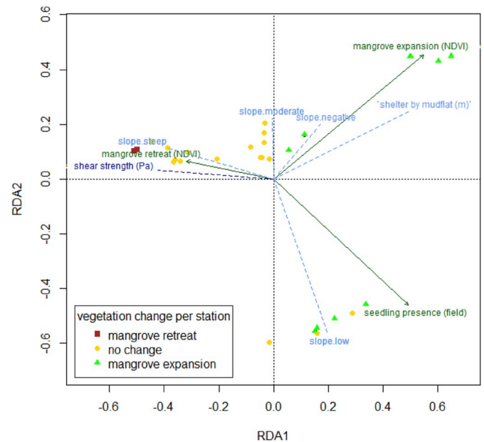
Fig. 6. Statistical analysis of parameters that drive seaward mangrove expansion. The RDA correlation plot shows the 29 stations that were investigated, coloured according to the condition as observed in the field and with GIS: seedling presence or mangrove expansion (green triangles), stations that did not change state over the wet season (yellow dots) and stations that showed mangrove retreat (brown squares). We related three seaside mangrove conditions (1: mature mangrove retreat landward based on NDVI change over the wet season of 2015–2016, 2: mature mangrove expansion seaward based on positive NDVI change over the same wet-season and 3: seedling presence in the field) with environmental parameters related to soil stability and wave exposure. The relation between the three seaside mangrove conditions (green, solid arrows) and the environmental parameters related to wave exposure (light blue dashed arrow) and soil stability (dark blue dashed arrow) can be deduced from the direction of the arrows similarly as in Fig. 5. In general, all environmental parameters that work along the horizontal axis explain 17% of the variance in seaside mangrove dynamics ( p < 0.01 ) and along the vertical axis explain 11% ( p < 0.05 ) of the variance. (For interpretation of the references to colour in this figure legend, the reader is referred to the Web version of this article.)
