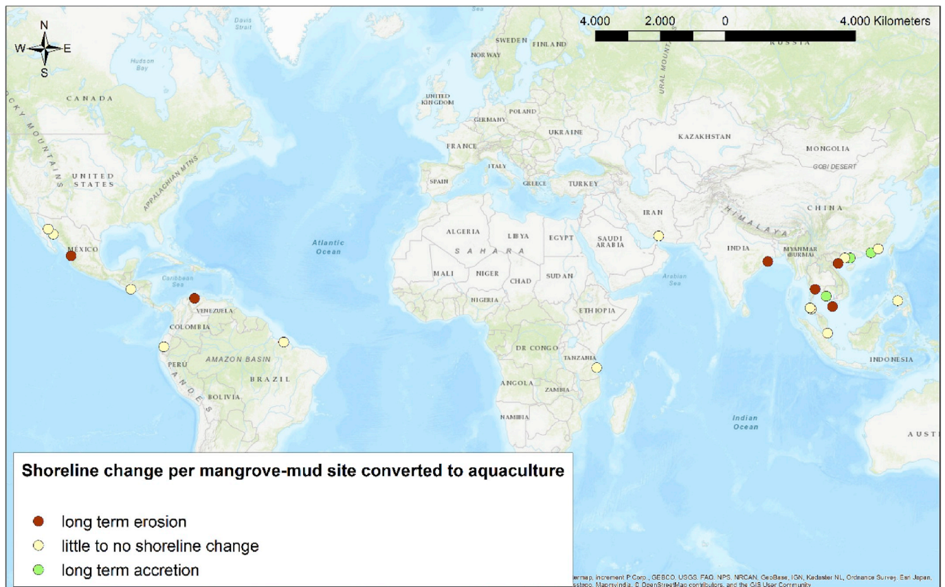
Fig. 1. Long term shore line changes from 1984 until 2016 as reported by Luijendijk et al. (2018) averaged per aquaculture coast. Aquaculture coasts displayed are sites designated by RAMSAR as internationally important wetlands, distinguished by mangroves and mudflats that have been (partly) converted to aquaculture (RAMSAR, 2018).
