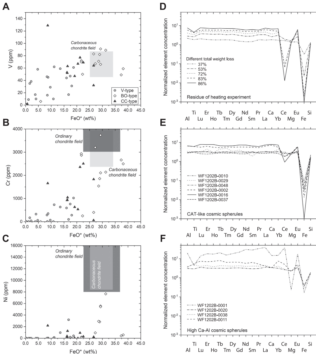
Fig. 11. (A–C) Binary plots of (partially) siderophile elements V, Cr, and Ni versus FeO*, as determined by LA-ICP-MS in this work. Fields for ordinary chondrites and carbonaceous chondrites (2 SD of the mean) based on Cr, Ni, and FeO* data from Jarosewich (1990) and V data from Friedrich et al. (2002). (D–F) Comparison of average major and trace refractory element concentrations in residues of heating experiments with varying total weight loss in % (Wang et al., 2001) with the CAT-like and high Ca-Al CS patterns determined in this work. The compositions of the CSs are normalized to CI chondrite (McDonough and Sun, 1995), while those of the residues are normalized to the starting solar composition (Wang et al., 2001).
