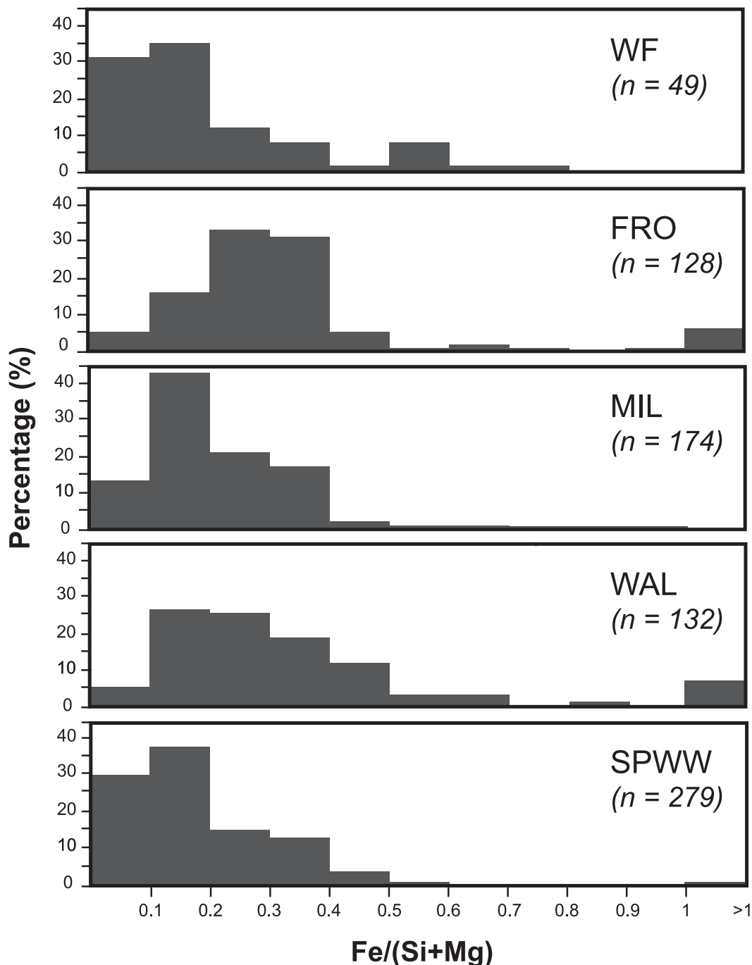
Fig. 6. Molar \text{Fe}/(\text{Si} + \text{Mg}) histograms for Widerøefjellet Mountain (WF; this work), Frontier Mountain (FRO, magnetic extract; Suavet et al., 2009 ), Miller Butte (MIL; Suavet et al., 2009 ), Walcott Névé (WAL, heavy fraction [methylene iodide, \rho = 3300 \text{ kg/m}^3 ] and magnetic extract of the light fraction; Suavet et al., 2009 ) and South Pole Water Well (SPWW; Taylor et al., 2000 ) micrometeorites. All data except for Widerøefjellet extracted from Suavet et al. (2009) .
