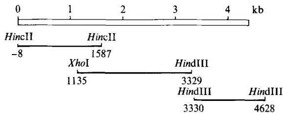
Fig. 8. E2 gene cloning strategy. cDNA from both clone PUR46. C1 of TGE virus and from the double mar mutant 1B. B5–1B. B1 selected from PUR46. C1 were cloned in the Bluescript plasmid using the indicated restriction enzyme fragments.
