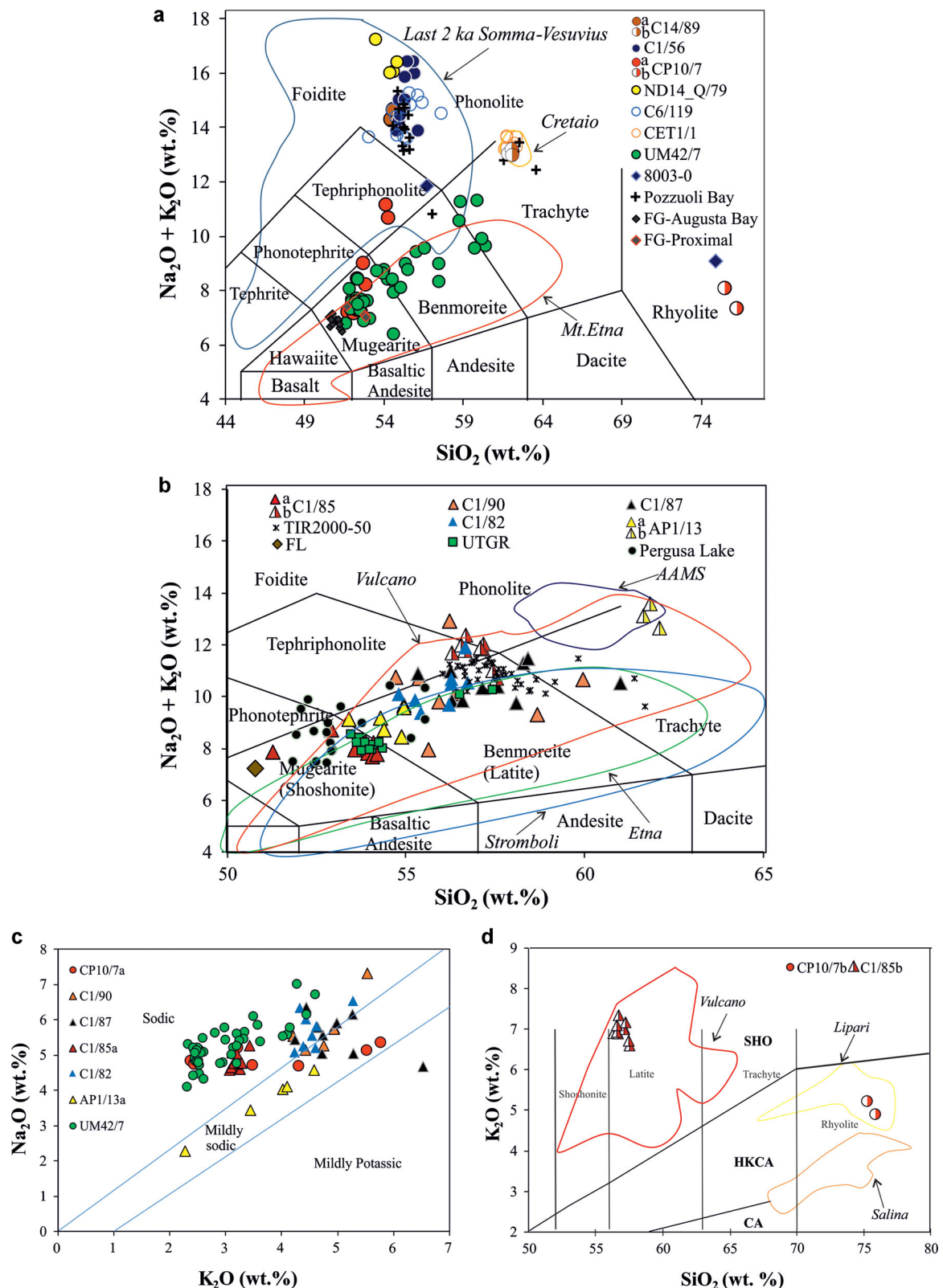
Figure 3. TAS classification diagrams (a, b) with composition of the studied tephras and cryptotephras. Compositional fields are labeled according to the Na- and K-series. The average compositional fields of proximal deposits and single glass data of some proximal and distal tephras are reported for comparison. Data for Somma-Vesuvius products are from Santacroce et al. (2008), Etna, Stromboli and Vulcano from Peccerillo (2005) and references therein, Cretaio from De Alteris et al. (2010), FG proximal and Augusta Bay from De Martini et al. (2010) and Smedile et al. (2011), AAMS group from Smith et al. (2011), Upper Tufi di Grotte Rosse (UTGR) and TIR2000-50 from Albert et al. (2012), 8003-0 from Paternè et al. (1988), C6/199 from Di Donato et al. (2019), Pozzuoli Bay glasses from Sacchi et al. (2014), FG and FL from Coltelli et al. (2000, 2005). (c) \text{K}_2\text{O}/\text{Na}_2\text{O} diagram to show the Na-alkaline affinity of studied cryptotephra and (d) \text{SiO}_2/\text{K}_2\text{O} diagram to show the shoshonitic and HKCA features of cryptotephra CP10/7 and C1/85. Data for Salina and Lipari rhyolites are from Albert et al. (2017). [Color figure can be viewed at wileyonlinelibrary.com ]
