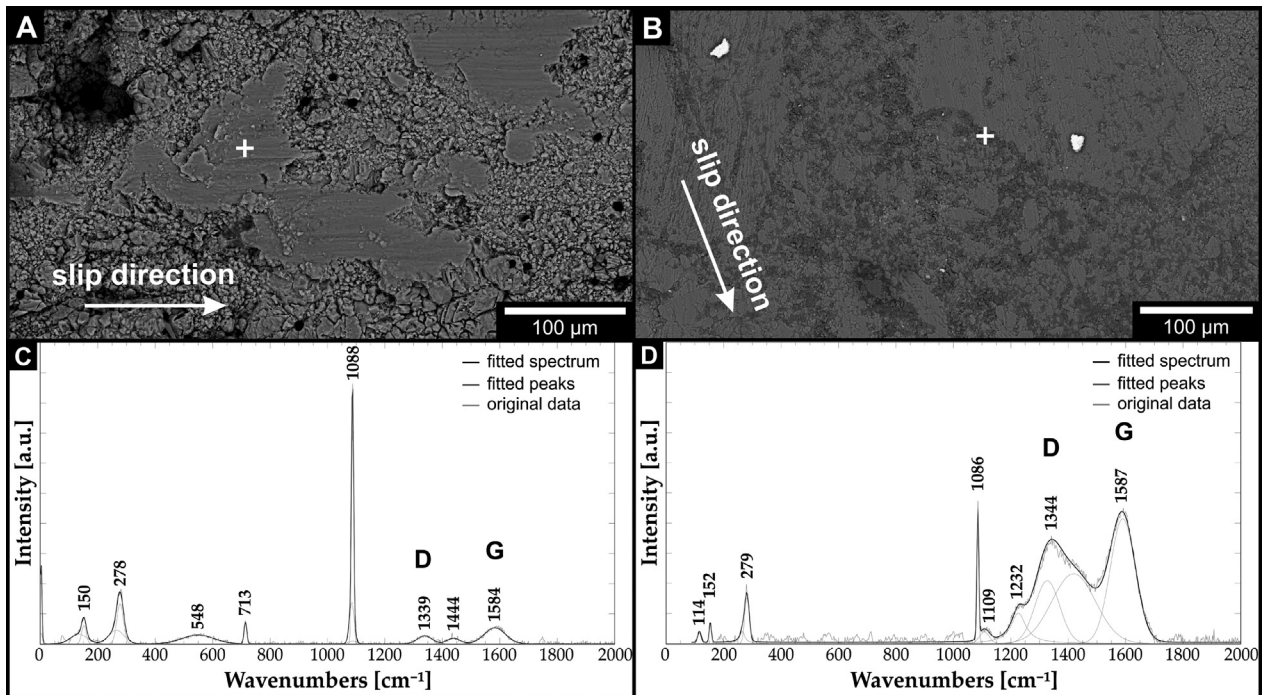
Fig. 4. Backscatterer electron images with locations of Raman spectroscopy measurements for Arkitsa (A and C) and Schinos (B and D) slip surfaces. A and B: Backscatterer electron images of the fault surfaces. A phase with low backscatter contrast (darker grey) is visible in B. C and D: Raman spectra showing the D and G peak position of a disordered carbon phase.
