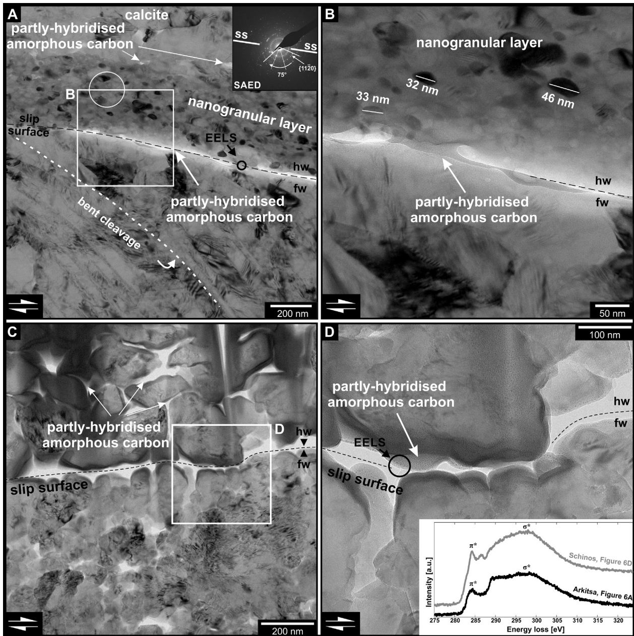
Fig. 6. TEM cross sections illustrating the relationship between hanging-wall ( hw ) breccia and footwall ( fw ) contact for Arkitsa (A–B) and Schinos (C–D). A: TEM bright field close-up from Fig. 5A. Non-crystalline carbon establishes the contact between hanging wall and footwall. The footwall consists of large, stressed calcite crystals with bent fractures. Nanogranular layer with non-crystalline carbon and calcite nanograins. White circle indicates SAED location (circle diameter = aperture diameter); black circle depicts EELS measurement (circle diameter = effective aperture diameter). Inset: SAED showing two sets of crystal orientation. ss = slip surface. B: TEM bright field close-up from A. Non-crystalline carbon connects hanging wall and footwall. The nanogranular layer produces Moiré fringes indicative of overlapping crystal lattices. Nanograins are not always in grain-to-grain contact. C: TEM bright field close-up image from Fig. 5B. The grain size of the hanging wall is 200 nm and larger. The grain size of the footwall directly at slip surface is about 100 nm. D: TEM bright field close-up image from C. The hanging wall and footwall are connected via non-crystalline carbon. Black circle depicts EELS measurement (circle diameter = effective aperture diameter). Inset shows EELS spectra from black circles in A and D.
