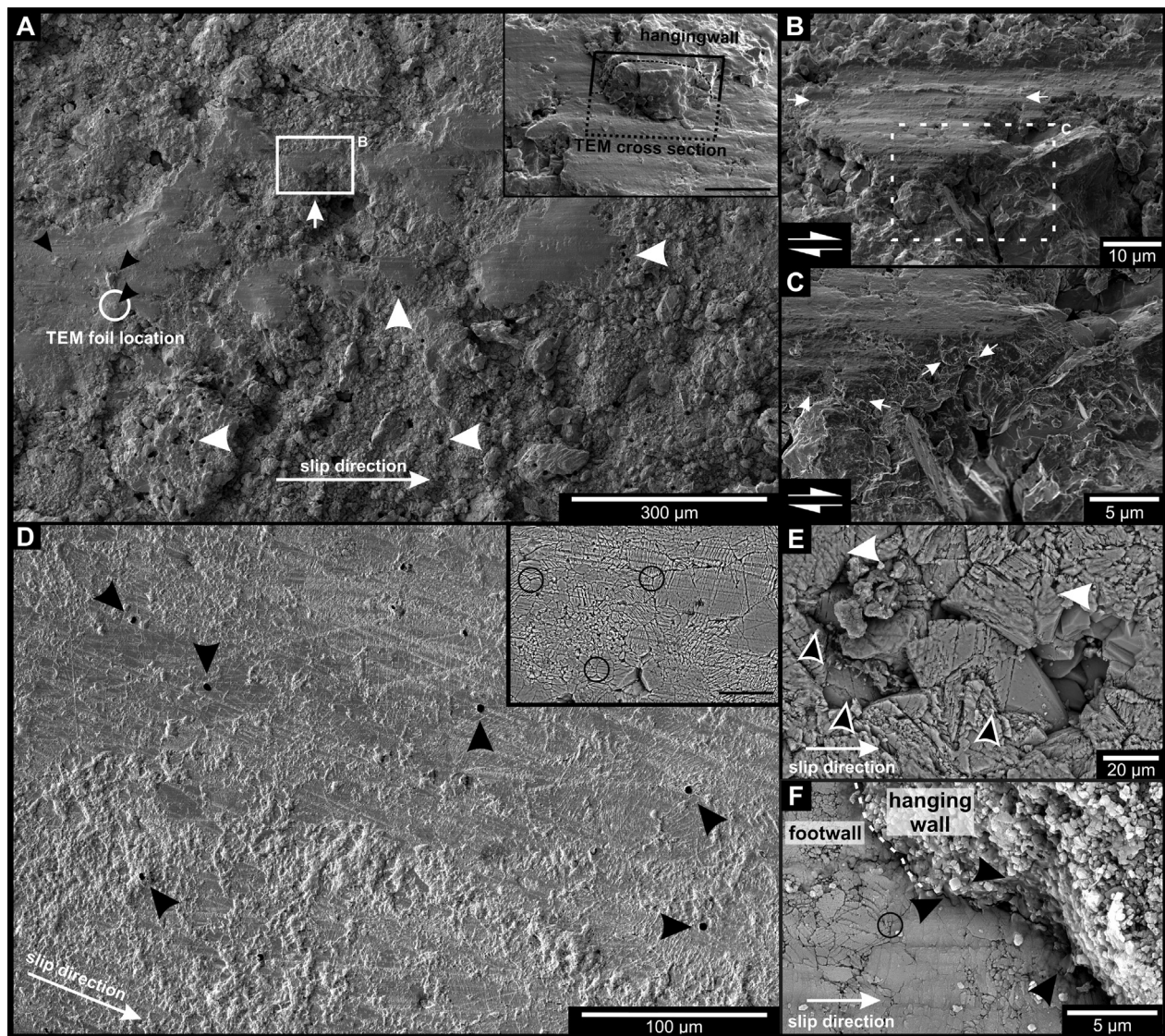
Fig. 3. Representative slip surface microstructures of the Arkitsa (A–C) and Schinos (D–F) exposures. A: Secondary electron overview image of the Arkitsa slip surface. Smooth slip patches with microgrooves parallel to slip direction. Uniform holes (white arrows) penetrate the slip surface. Residue of hanging wall on top of the slip surface patch (black arrows, white circle) with TEM sample location. Inset: Detailed view of TEM foil location from Fig. 5A, white circle. Scale bar = 5 \mu\text{m} . B: Close-up of slip surface from A. Fine-grained slip surface material situated on top of coarse fault rock grains. Microscope stage tilted to 52°. C: Close-up of section from B. Amorphous material covers roundish grains (black arrows). D: Secondary electron image of Schinos slip surface with microgrooves parallel to slip direction. Uniform holes penetrate the principal slip surface (black arrows). Inset: Backscatter electron image illustrating triple junction grain boundary contacts. Scale bar = 50 \mu\text{m} . E: Backscatter electron image top view onto the slip surface. Cracks in idiomorphic calcite crystals are visible a few micrometres into the crystal (black-white arrows). Amorphous material with low backscatter contrast covers parts of the slip surface and reduces surface roughness (white, dashed lasso) F: Backscatter electron image of the contact between footwall and hanging wall (dashed line). Black arrows indicate the locations of an amorphous material with lower backscatter contrast. Black circle shows grain boundary triple junction.
