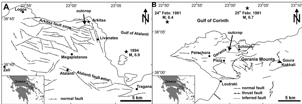
Fig. 1. Tectonic maps of the study areas. Insets show the geographical location within central Greece. A: Location of the studied exposure of the Arkitsa fault zone (modified after Jones et al., 2009; earthquake data: NOAA). B: Outcrop location of the Schinos fault segment north of Corinth (modified after Kaplanis et al., 2013 and Collier et al., 1998).
