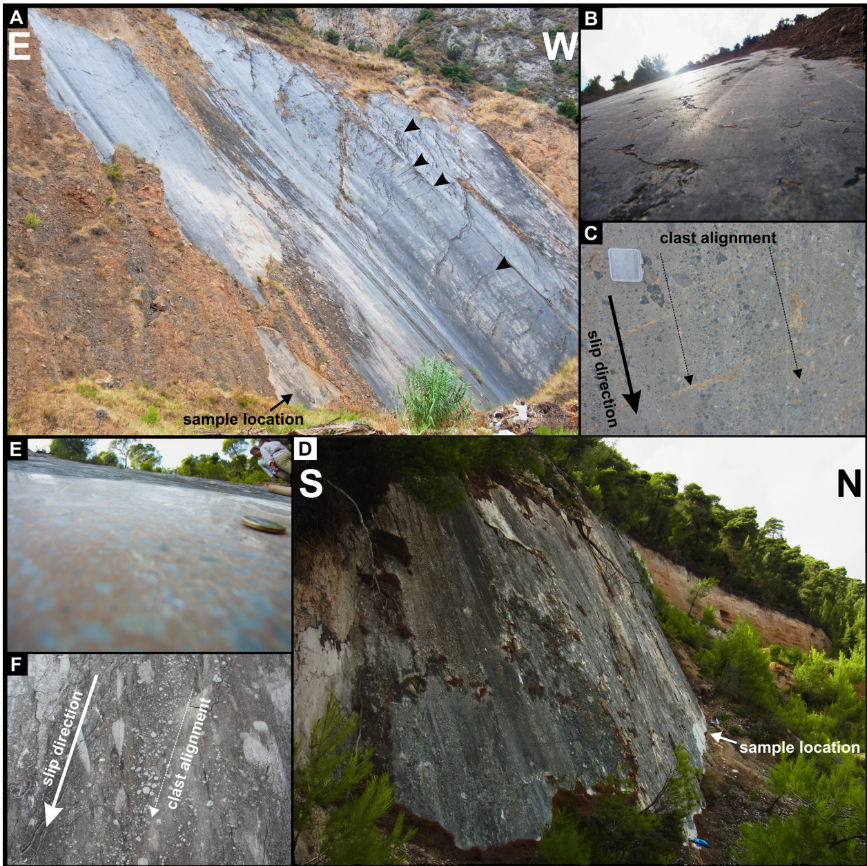
Fig. 2. Representative field structures from Arkitsa (A–C) and Schinos (D–F) fault exposures. A: Overview of Arkitsa fault exposure showing one of the three main slip planes with reddish-brown hanging-wall breccia cover on part of the slip surface. Black arrows indicate fractures perpendicular to slip direction. Person for scale, bottom right corner. B: Fault surface reflecting sunlight. C: Alignment of host rock fragments parallel to slip direction. Box approx. 5 \times 4 cm. D: Schinos fault surface exposure shows grey weathering of the slip plane. The slip plane is curved with the salient pointing out of the figure. Fault scarp to the north is now covered by alluvium. E: Image demonstrating fault surface reflectivity. Reflection of vegetation along the top edge and above the one-euro coin. F: Grey, weathered fault plane showing a strong alignment of light grey host-rock clasts parallel to slip direction (one-euro coin for scale, bottom edge).
