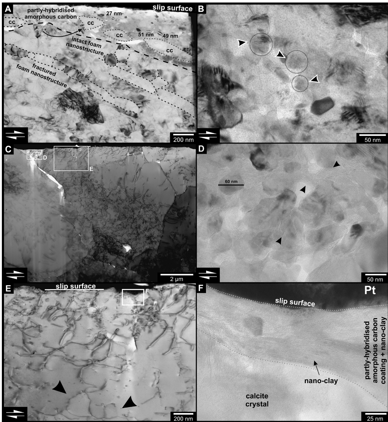
Fig. 8. Nanostructures of fault surface coating and nanograin abundance not associated with the principal slip surface. A: Bright-field TEM image from the Arkitsa exposure. Amorphous slip surface coating with calcite nanograins and crystal fragments from underlying foam nanostructure (black arrow). A sharp contact separates the underlying nanostructure from the slip surface coating. Nanostructure with former fracture planes (dashed lines), which originate from the principal slip surface, and overprint the existing nanostructure. B: Calcite nanograins away from the principal slip surface hosted inside non-crystalline carbon. Tip direction of black-white arrows indicate lattice fringe orientation of new grains. C: Bright-field STEM image overview. Large grains (5 \mu\text{m} ) with a heterogeneous dislocation density distribution. D: Calcite nanograins in non-crystalline carbon as a filling between two grain boundaries directly at the principal slip surface. Clay minerals wrap around the nanograins (black arrows). E: Bright-field STEM close-up from C showing the dislocation structure directly at the principal slip surface. Black arrows point to frozen dislocation loops. F: Bright-field TEM image from the Schinos exposure. Amorphous slip surface coating mixed with nano-clay on top of calcite crystal. cc = calcite.
