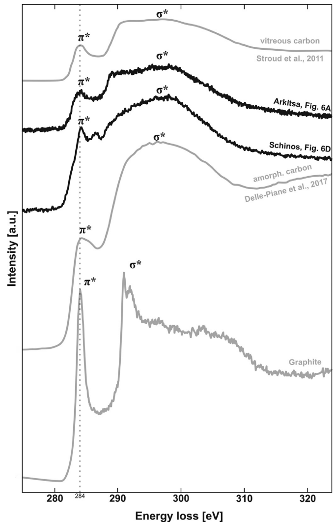
Fig. 9. Comparison of electron energy loss spectra. Calcite decomposition products presented here have a small intensity difference of \pi^* to \sigma^* peak. The EEL spectrum from vitreous (glass-like) carbon (Stroud et al., 2011) exhibits a similar \sigma^* -peak shape compared to the acquired spectra of this study. Reference spectrum of graphite has three weak \sigma^* peak features which are absent in all other carbon spectra.
