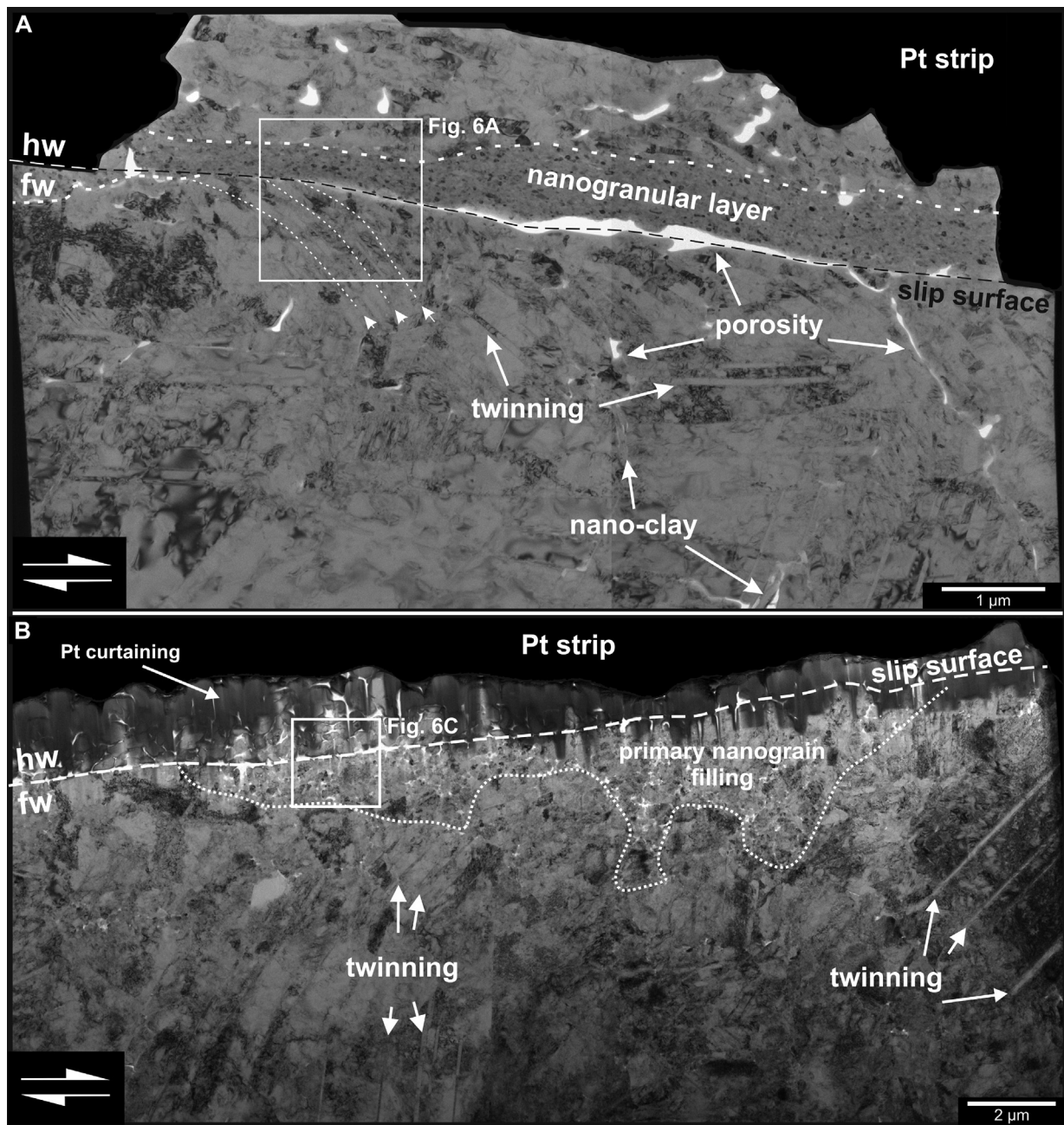
Fig. 5. Overview of TEM cross sections into the principal slip surfaces of Arkitsa and Schinos, including preserved hanging-wall residue. A: Bright-field TEM image overview of representative Arkitsa nanostructures. The hanging-wall breccia consists of small, elongated calcite fragments held in place by non-crystalline carbon. The nanogranular layer is part of the hanging-wall breccia and lies on top of deformed calcite crystals. Fractures (dashed lines) bend down from the principal slip surface into the deformed calcite crystals. Fractures and holes form porosity inside the mirror slip volume and are filled either with non-crystalline carbon and/or nano-clay (see arrows with labelling). B: Bright-field TEM image with representative Schinos nanostructural hanging-wall to footwall relation. The hanging wall consists of small grains of several hundred nanometres. Individual grains are surrounded by non-crystalline carbon. The footwall hosts a discontinuous, primary nanograin filling. The grain size increases abruptly with distance from the slip surface to grains of several micrometres in size. Larger grains contain twins. hw = hanging wall, fw = footwall.
