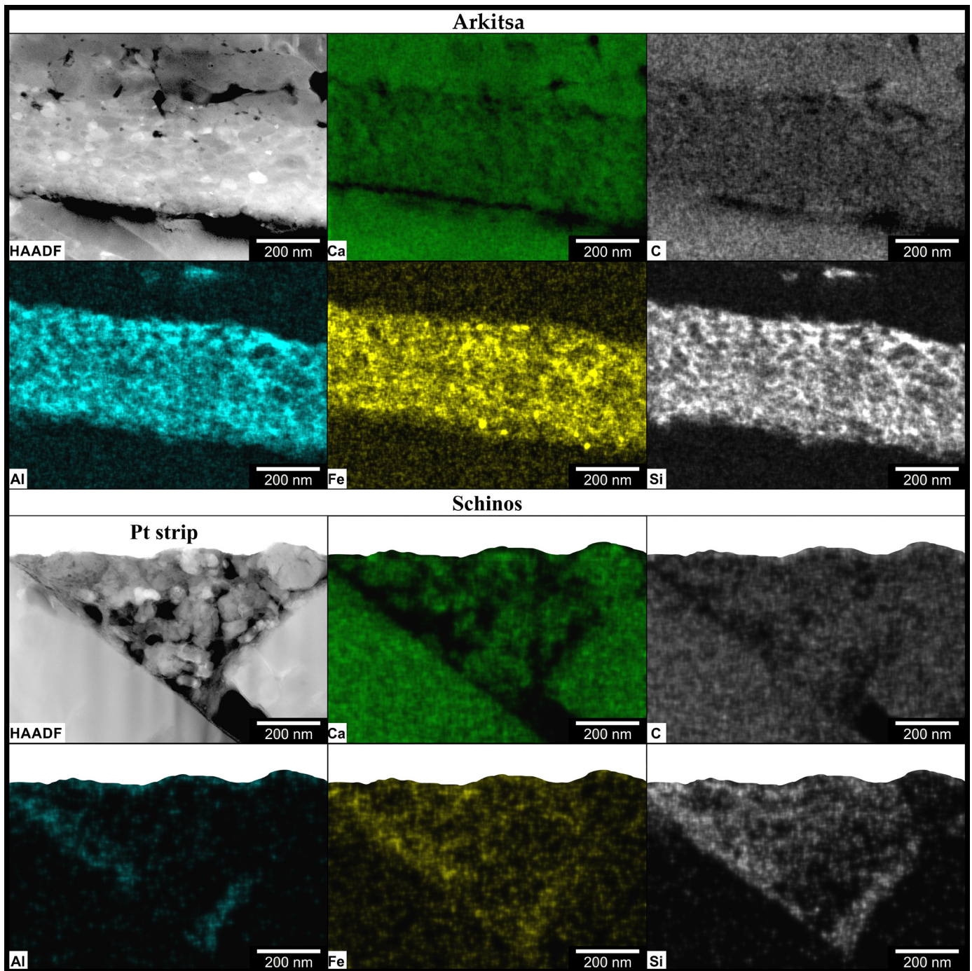
Fig. 7. TEM-EDX maps of calcite nanogranular layer from Fig. 5A (Arkitsa) and surface filling Fig. 8C (Schinos) visualizing the element distribution. Overlap of calcium (Ca) and carbon (C) distribution confirms that the grains inside are calcite. Aluminium (Al), iron (Fe) and silicon (Si) are concentrated in the interstitial region around the calcite grains.
