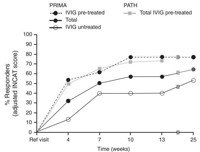
FIGURE 1 Cumulative INCAT response rate in PRIMA and PATH. INCAT, inflammatory neuropathy cause and treatment; IVIG, intravenous immunoglobulin; PATH, Polyneuropathy And Treatment with Hizentra; PRIMA, Priven Impact on Mobility and Autonomy
