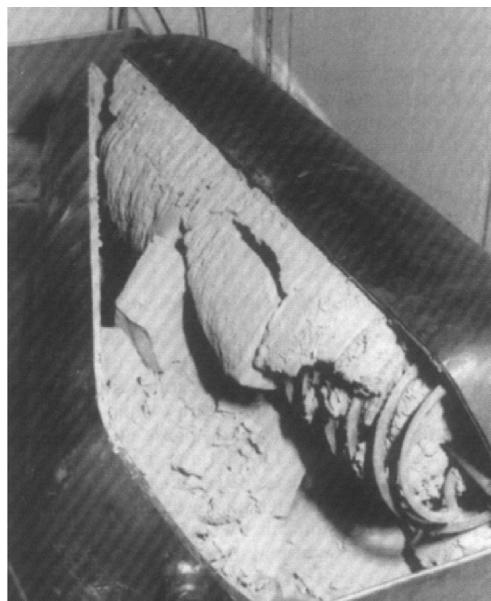
Fig. 36 – Left: layout of \text{MgH}_2 tank for a process steam generator. Right: The tank opened after 1.5 years of operation [345].
