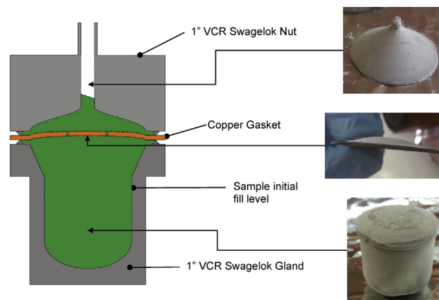
Fig. 32 – Following 150 rapid cycles at 400^\circ\text{C} the Mg powder has sintered into porous structure growing through 0.5 mm diameter holes in a Cu gasket and expanding up the 1/4'' gas transfer tube.
