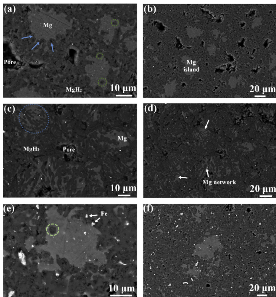
Fig. 15 – Backscattered electrons (BSE) scanning electron microscopy micrographs of the pellets hydrogenated to 80–90% of maximum theoretical hydrogen storage capacity (a,b- Mg pellet; c,d- Mg-2wt% MWCNTs, and e,f- Mg-2wt% Fe). The view plane is perpendicular to the compression axis. (a)-Circles mark individual unimpinged isotropic \text{MgH}_2 nuclei. Arrows point on impinged \text{MgH}_2 nuclei forming wavy Mg/ \text{MgH}_2 interface. (b) Lower magnification micrograph showing the isolated pockets of unreacted Mg surrounded by the \text{MgH}_2 phase. (c) Elongated anisotropic \text{MgH}_2 nuclei (marked by the circle), (d) Micrograph showing the developed Mg network along the sample. (e) Symmetrical \text{MgH}_2 nucleus formed next to the Fe particle. (f) Increased number of hydride nucleation sites results in smaller size of metallic Mg islands in comparison with the reference Mg pellet [273].
