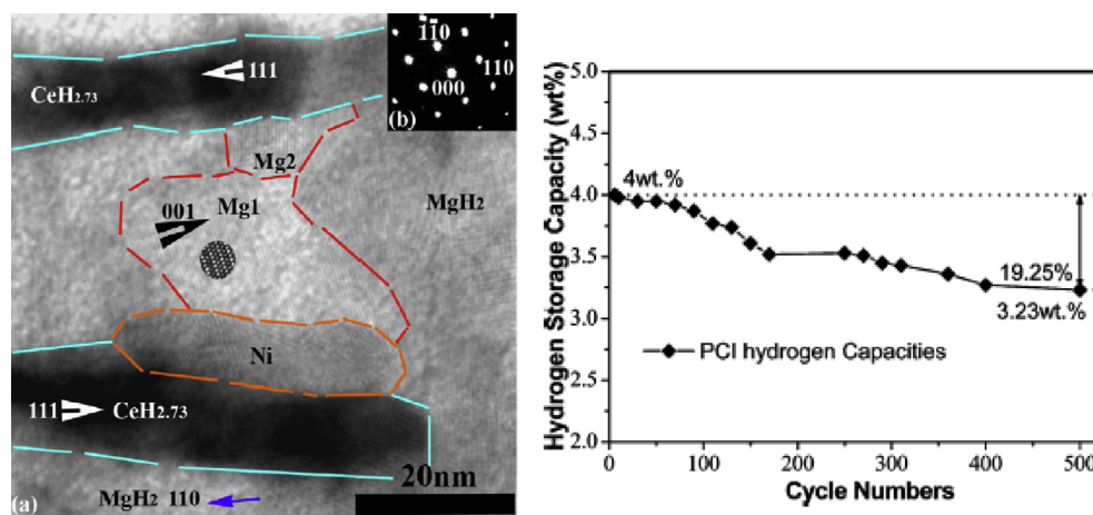
Fig. 18 – Left: TEM images of the microstructure of the partially dehydrogenated \text{MgH}_2 - \text{CeH}_{2.73} -Ni nanocomposites demonstrate the catalyst effect of \text{CeH}_{2.73} and Ni on \text{MgH}_2 dehydrogenation process. (a) Bright field image and (b) selected area diffraction patterns of \text{MgH}_2 (zone axis [011]). Right: Evolution of the maximum hydrogen sorption capacities versus cycle times of \text{MgH}_2 - \text{CeH}_{2.73} -Ni composite [286].
