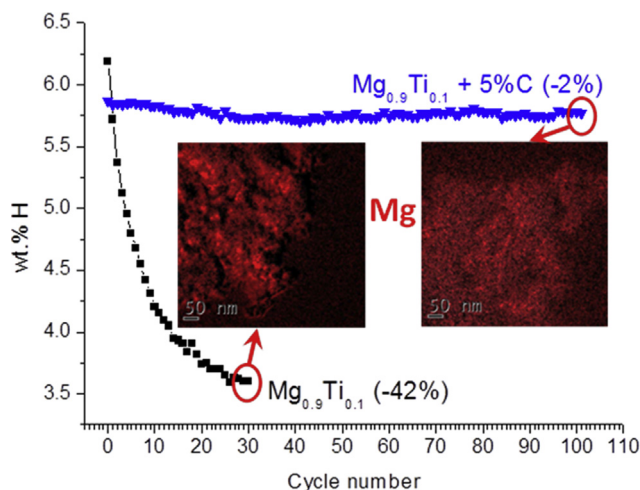
Fig. 13 – Reversible hydrogen storage capacity of HRBM MgH 2 -TiH 2 at T=350 °C. The values in brackets specify the capacity losses throughout the cycling. The insets show elemental maps of Mg in the cycled composites clearly indicating its grain refinement in the graphite-modified material [67].
