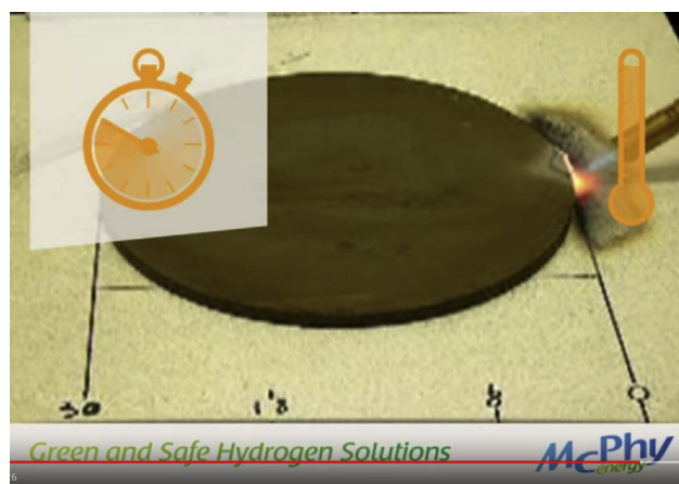
Fig. 37 – Fire testing of McPhy's \text{MgH}_2 composite. No explosion or fire propagation observed during one minute long test. The video is available at https://www.youtube.com/watch?v=RohMt2-UKQI .
