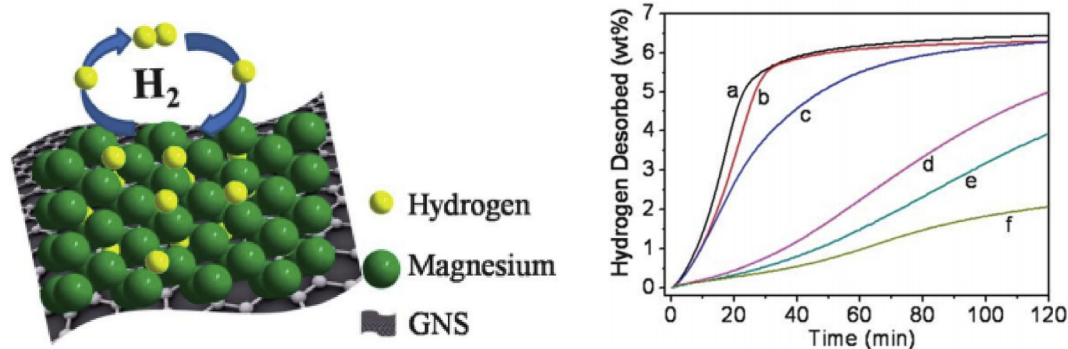
Fig. 11 – Schematic of hydriding/dehydriding reaction in \text{MgH}_2 -GNS composite, and hydrogen desorption curves of the sample at 300 °C: (a) \text{MgH}_2 -5GNS-20 h, (b) \text{MgH}_2 -5GNS-15 h, (c) \text{MgH}_2 -5GNS-10 h, (d) \text{MgH}_2 -5GNS-5 h, (e) \text{MgH}_2 -5GNS-1 h, and (f) \text{MgH}_2 -20 h [256].
