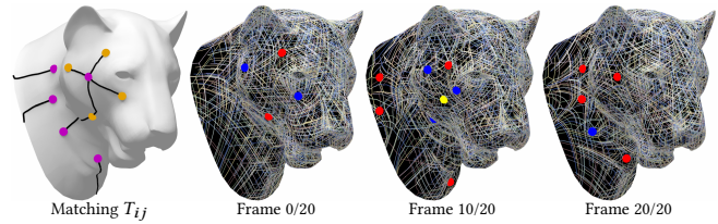
Fig. 2. Given two (3-RoSy) fields on a surface (frames 0, 20), we match the singular points (left; orange for the first field, purple for the second) using the signed matching problem (4). Our interpolant is designed to slide singularity indices along the geodesics; at t = 0.5 (frame 10) the singular points have split their indices according to the matching and moved along the geodesics between the start and end points.
