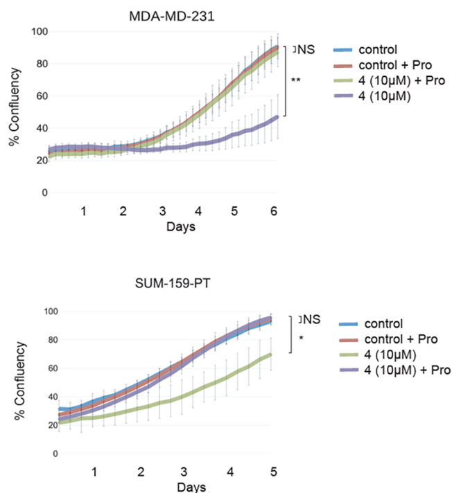
Fig. 7. Results of the cell proliferation assay for both MDA-MB-231 and SUM159PT breast cancer cell lines. Controls were performed both with and without exogenous proline showing normal growth in both cell lines. Compound 4 (10 \mu M) showed a 40% and 30% reduction in the MDA-MB-231 and SUM159PT cells, respectively. Cell growth was completely rescued in the presence of exogenous proline.
