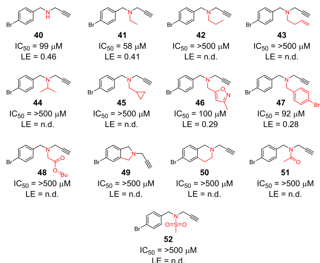
Fig. 4. Structure and activity of alterations to the N -methyl group (red).
