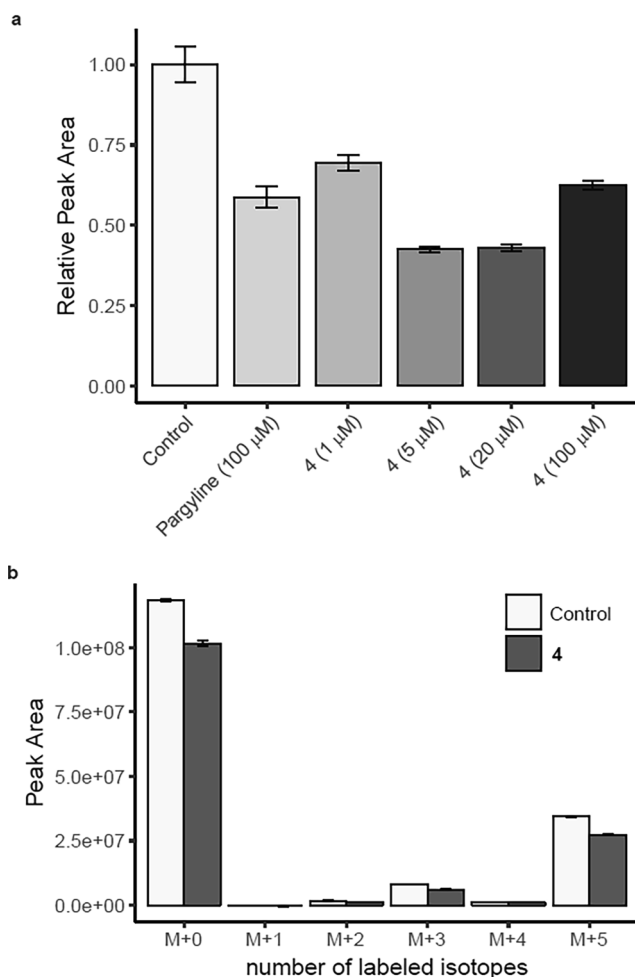
Fig. 6. (a) Results of the LC-MS based amino acid assay, showing the quantity of proline present in lysed human breast cancer cells (SUM-159-PT) after incubation with pargyline and compound 4. (b) Results of the glutamine flux study showing lower levels of M+5 proline after incubation with compound 4 ( 5 \mu M ).
