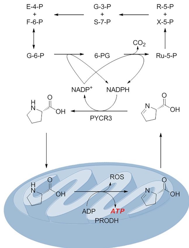
Fig. 1. The proline cycle and pentose-phosphate pathway (adapted from Ref. 2).
