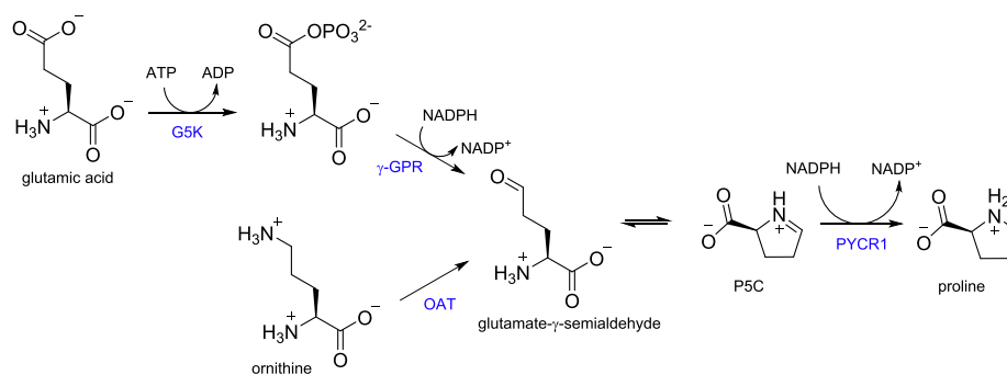
Scheme 1. The proline biosynthesis pathway (adapted from Ref. 1).
