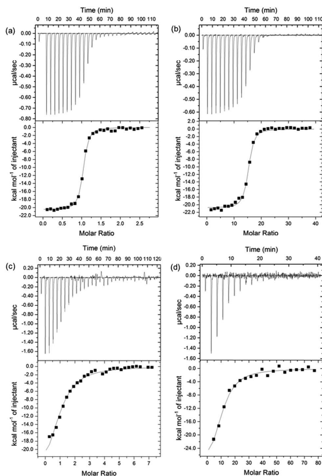
Fig. 3 Titrations of (a) 137 \mu\text{M} GM1os into 8.91 \mu\text{M} CTB at 25 °C; (b) 110 \mu\text{M} CTB into 0.5 \mu\text{M} P2-GM1os at 25 °C; (c) 376 \mu\text{M} GM1os into 9.32 \mu\text{M} CTB at 60 °C; and (d) 378 \mu\text{M} CTB into 1.0 \mu\text{M} P2-GM1os at 60 °C. CTB concentrations refer to the concentration of the B subunit.
