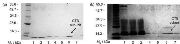
Fig. 4 The 'catch-and-release' behaviour of P2-GM1os functionalised beads applied to (a) a 10 \mu M solution of CTB in PBS pH 7.4; and (b) Vibrio sp. 60 growth medium, as demonstrated by gel electrophoresis. In each case lane 1 contains the analyte; lane 2 beads after exposure to analyte; lane 3 the supernatant after analyte loading; lanes 4 and 5 contain the bead washes with PBS at room temperature; lane 6 contains the eluate obtained after treatment with PBS at 60 ^{\circ} C and lane 7 the beads after elution. Gels were stained using Coomassie blue (a); or silver stain (b).
