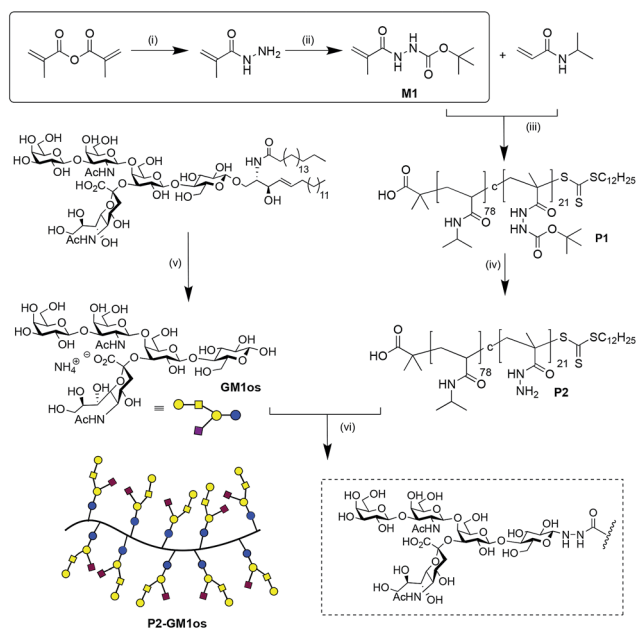
Scheme 1 Preparation of P2-GM1os . (i) \text{N}_2\text{H}_4 \cdot \text{H}_2\text{O} , \text{CHCl}_3 , rt, 1 h. (ii) Di- tert -butyl dicarbonate, THF, rt, 24 h. (iii) S -Dodecyl- S' -( \alpha, \alpha' -dimethyl- \alpha'' -acetic acid)trithiocarbonate, 2,2'-azobis(2-methylpropanitrile), DMSO, 70 °C, 18 h. (iv) 50% v/v \text{CH}_3\text{COOH} , \text{CH}_2\text{Cl}_2 , rt, 1 h. (v) EGCaseII, 25 mM \text{NH}_4\text{OAc} , pH 5.0, 0.2% v/v Triton X-100. (vi) 100 mM \text{NH}_4\text{OAc} , pH 4.5, rt, 18 h.
