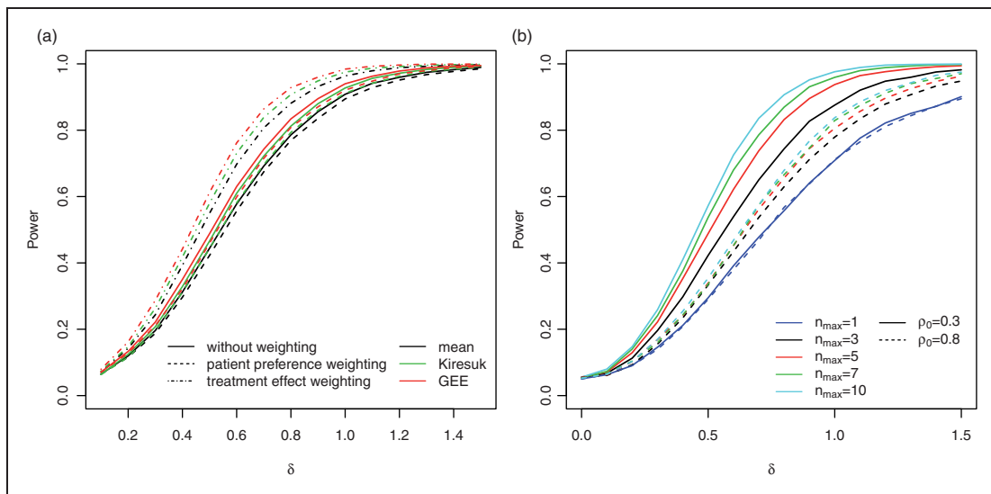
Figure 4. (a) The power of the three considered testing procedures without weighting, with patient preference weighting (Case (i) in Section 3.2) and with treatment effect weighting (Case (ii) in Section 3.2) in the reference scenario for \rho_0 = 0.3 and n_{max} = 5 . (b) The power of the GEE approach for different maximum number of goals ( n_{max} = 1, 3, 5, 7, 10 ) and correlations \rho_0 = 0.3, 0.8 . For the respective power curves for the t -tests applied to the mean and standardised mean scores, see Figures S1 in the Supplementary Material.
