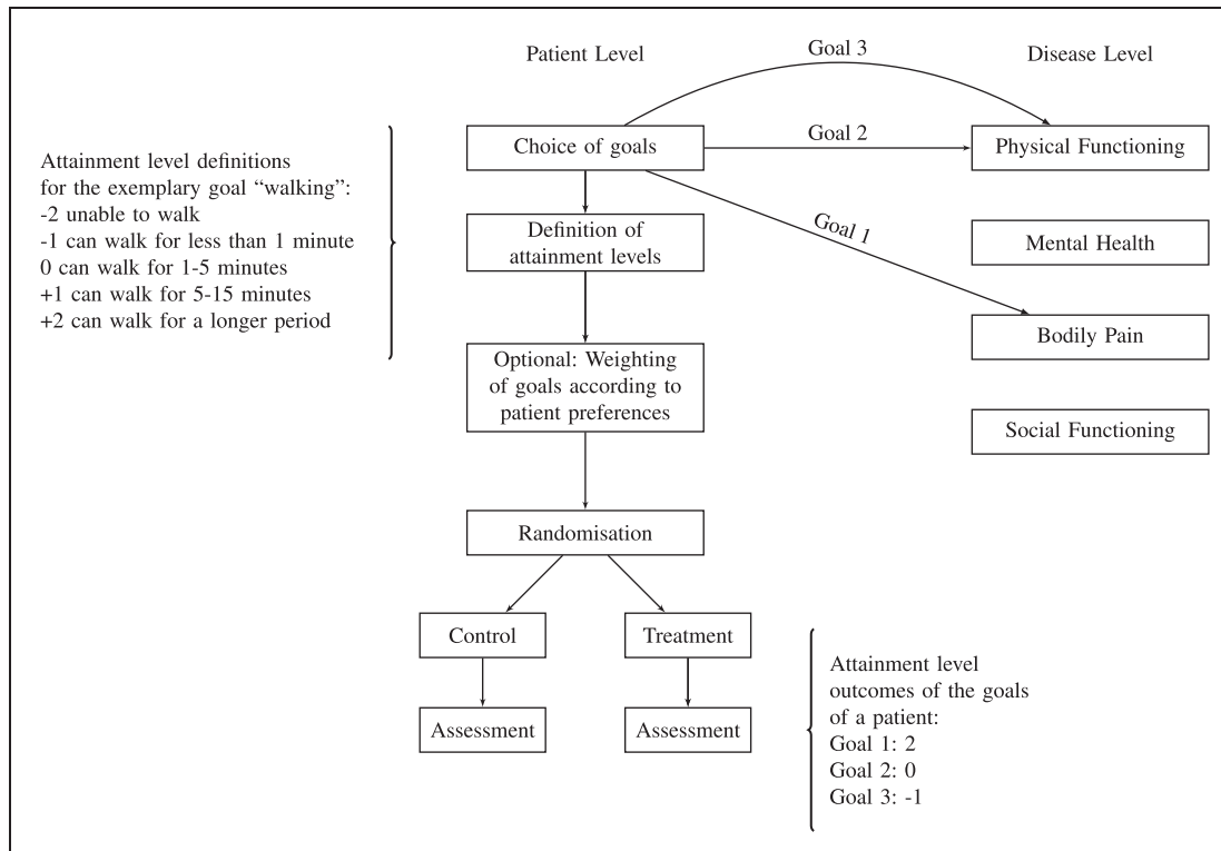
Figure 1. Illustration of the application of a GAS endpoint in a randomised clinical trial. Supported by an investigator, each patient chooses disease related goals he or she wants to attain. The type and the number of goals are chosen individually and can correspond to different dimensions of symptoms. In the example, the patient chooses two goals related to physical functioning and one goal related to bodily pain but no goal related to the other dimensions. For each goal criteria, specific attainment levels are defined before the intervention. Additionally, goals can optionally be weighted to quantify differences in importance and relevance of the goals. After the goals are set, patients are randomised and allocated to the treatment groups. After a predefined follow-up period, the attainment level for each goal is assessed according to the pre-specified criteria.
