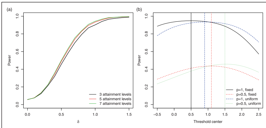
Figure 6. (a) The power for the GEE approach for discrete goal attainment scales with L = 3, 5, and 7 levels such that c_j = \Phi^{-1}(j/L), j = 1, \dots, L and other parameter values are as in the reference scenario. For the respective power curves for the t -tests applied to the per-subject mean and standardised mean scores, see Figure S1 in the Supplementary Material. (b) The Power of the t -test based on per-subject means if the discretisation of the continuous attainment levels, which is centred around 0 in the reference scenario, is based on other threshold centre values. For different threshold centre values t , we set c_j = \Phi_{t,1}^{-1}(j/0.2), j = 0, \dots, 5 , where \Phi_{t,1}^{-1} denotes the quantiles of the normal distribution with mean t and variance 1. The distribution of effect sizes was either assumed to be a mixture distribution on 0 and \delta (fixed effect) or 0 and a uniform distribution on [0, 2\delta] (uniform) with weights 1 - p and p .
