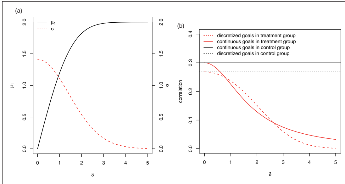
Figure 2. (a) The expected value of the goal attainment scores X_{ik} in the treatment group \mu_1 and their variance \sigma as function of \delta in the reference scenario described in Section 3.2. (b) The correlations of the continuous and discretised goal scores X_{ik}, X_{ik'} and Y_{ik}, Y_{ik'}, k \neq k' within a patient as function of \delta for \rho_0 = 0.3 .
