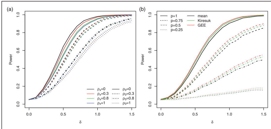
Figure 5. (a) The power of the t -test for standardised means for the case where correlations \rho_x \neq \rho_0 are chosen in equation (2) to compute the standardised means \bar{Z}_i for the reference scenario. Figure (b) shows the power under the assumption that the effect size follows a mixture distribution with weight 1 - p on 0 and weight p on a uniform distribution on [0, 2\delta] , using the t -test applied to the per-subject means (mean) and standardised per-subject means (Kiresuk), and the test based on the GEE model (GEE) for the reference scenario.
