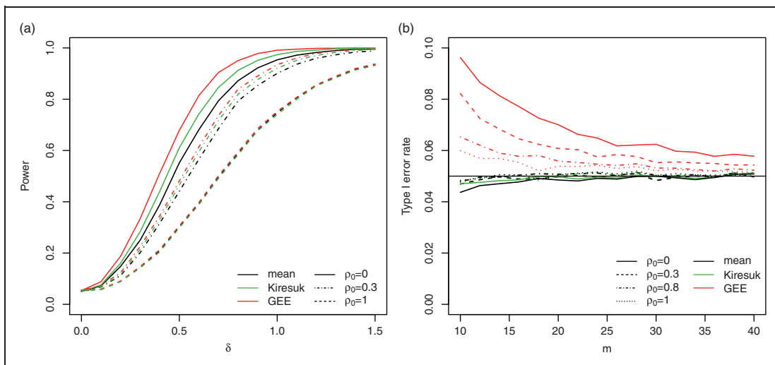
Figure 3. The power (a, 10^4 simulation runs) and type I error rate (b, 10^5 simulation runs) of the t -test based on the per-subject means (mean), the t -tests based on the standardised per-subject means (Kiresuk), and the test based on the GEE model (GEE) for the reference scenario.
