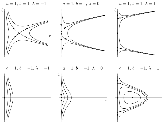
Fig. 1 Phase portraits of the planar reduced system as the bifurcation parameter \lambda passes through 0 for the hyperbolic ( a = b = 1 ) and the elliptic ( a = 1, b = -1 ) volume-preserving Hopf bifurcations
