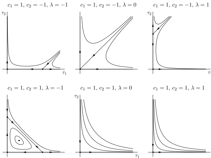
Fig. 2 Phase portraits of the planar reduced system as the bifurcation parameter \lambda passes through 0 for the hyperbolic ( c_1 = 1, c_2 = -1 ) and elliptic ( c_1 = c_2 = 1 ) cases of the volume-preserving double Hopf bifurcation
