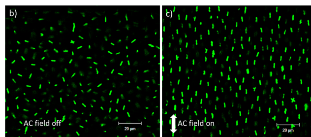
Figure 2. (a) Illustration of a capillary setup where the NU-1000 Si suspension in the cell is exposed to an alternating E-field perpendicular to the viewing direction (top) and cross-sectional view of the glass capillary setup (bottom). Confocal microscope images of NU-1000 Si suspensions in bromobenzene (b) without E-field, showing randomly oriented particles and (c) in the presence of 500 Hz, 37.5 V·mm -1 peak-to-peak E-field showing aligned particles.
