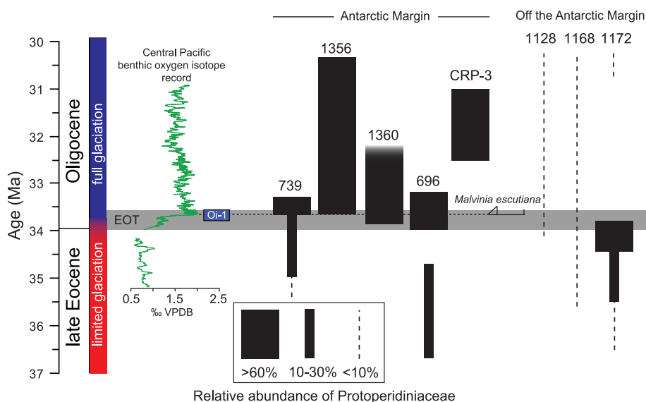
Fig. 3. Summary of the relative abundance of proto-peridiniacean dinocysts at circum-Antarctic drill sites. The deep-sea oxygen isotope record is after (4), and Oi1 marks the final large oxygen isotope shift of the EOT (gray band). Large specimens of S. cf. antarctica and M. escutiana occur from Oi1 onward. If no bar is indicated, there is no sedimentary record for that time interval. Proto-peridiniacean dinocysts abundant in the Upper Eocene of ODP site 1172 solely comprise Brigantedinium spp. and are likely related to oceanic upwelling conditions at this location (35) (supplementary materials).
