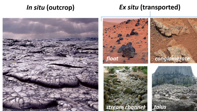
Fig. 1.18. For igneous rocks, the lithologic, textural, and chemical diversity of the sample collection is far more important than collecting only rocks with known outcrop-scale context. There are multiple geological processes that could transport diverse rocks to places where the rover could sample them. Igneous sampling strategies need to encompass both in situ (in outcrop) and ex situ (transported) options. Image notes: In situ: Hawaii; Ex situ: Upper left: Low Ridge, Gusev (NASA/JPL-Caltech/Cornell/NMMNH); upper right: Gale Crater (NASA/JPL-Caltech/MSSS) lower left and right: Generic images from the web.
