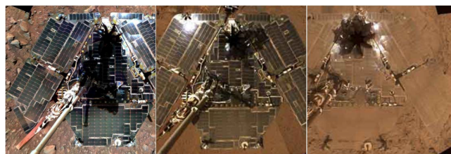
Fig. 6.2. Mastcam views of the change in the Spirit rover dust coverage. (Photo Credit: NASA). Pervasiveness of Martian dust illustrates exposure hazards for astronauts and potential back-contamination of Earth.
