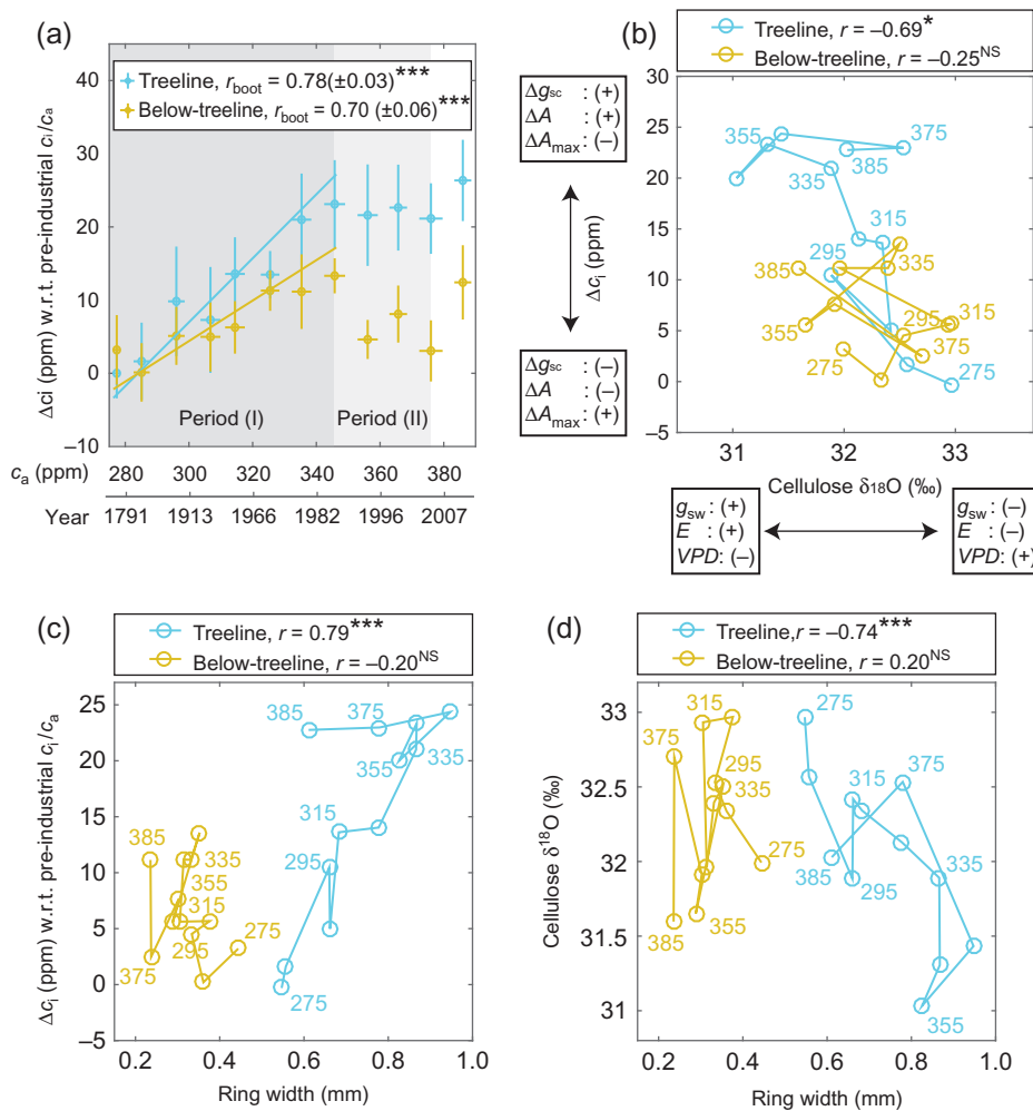
Figure 4. Interpretation of the dual-isotope model over the period AD 1700–2010. (a) Relationship between c_a and the deviation in \delta^{13}\text{C} -derived c_i from the 'active' (constant c_i/c_a ) response of \delta^{13}\text{C} to c_a , termed \Delta c_i . Data points and error-bars indicate the average and one-standard deviation confidence intervals calculated over 10 ppm c_a bins. The c_a intervals indicated by the shaded periods (I) and (II) indicate distinct responses of \Delta c_i to c_a (see Fig. S3c available as Supplementary Data at Tree Physiology Online ); significant positive responses of \Delta c_i to c_a were observed in period (I), whereas a shift to non-significant or negative responses was observed in period (II). Bootstrapped correlation coefficients ( r_{\text{boot}} ) and their standard deviations were calculated over 10 ppm c_a bins in period (I) only. (b) Temporal relationship between cellulose \delta^{18}\text{O} and \Delta c_i . The black boxes near the axes extremes indicate the interpretation of the adjusted dual-isotope model in terms of changes in stomatal conductance to water vapour ( g_{\text{sw}} ), transpiration ( E ) and vapour pressure deficit (VPD), and relative changes in stomatal conductance to CO 2 ( \Delta g_{\text{sc}} ), photosynthesis ( \Delta A ) and photosynthetic capacity ( \Delta A_{\text{max}} ). (c) Temporal relationship between annual average ring width and \Delta c_i . (d) Temporal relationship between annual average ring width and \delta^{18}\text{O} . Markers in panels (b–d) indicate the centre of 10 ppm c_a bins of the treeline and below-treeline sites. Subsequent data points are connected by solid lines, with bin-average c_a indicated for every second bin. The correlation coefficients in panels (b–d) indicate the sign of the relationship calculated across the averages of 10 ppm c_a bins over the period AD 1700–2010. Significance levels of correlations are indicated by *** for p < 0.001 , * for p < 0.05 , and NS for p \geq 0.05 .
