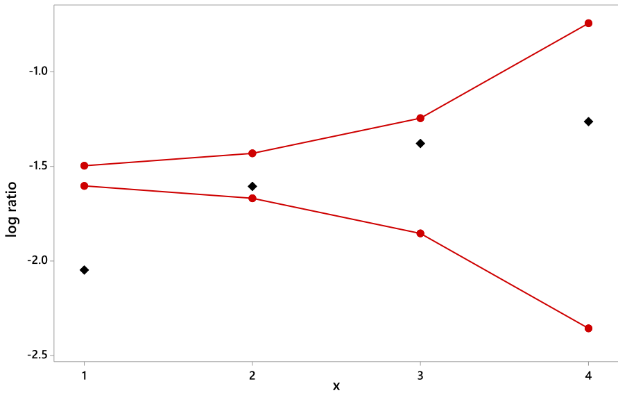
Fig. 5 Geometric ratio plot under the null for the domestic violence data of Example 1
