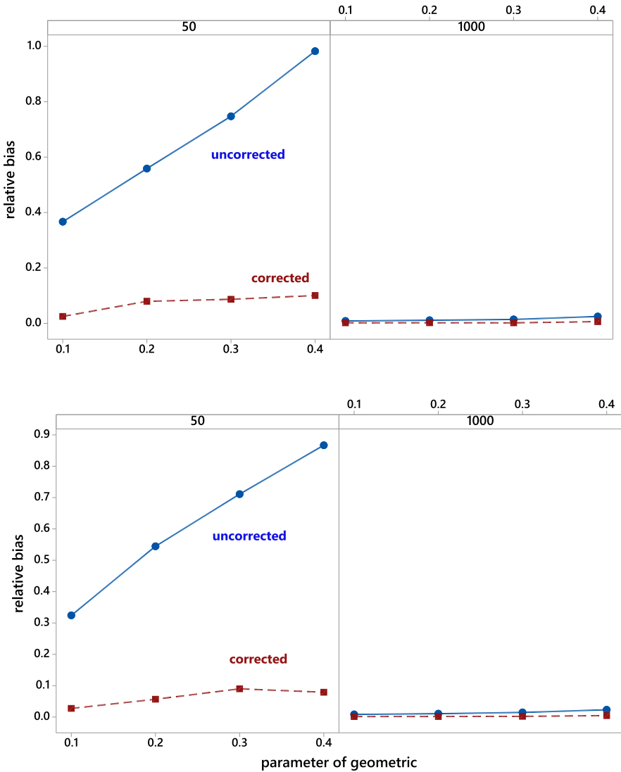
Fig. 7 Comparison of the modified Chao estimator n + f_2^3/f_2^2 with its bias-corrected version (16) for a geometric distribution with parameters \theta = 0.1, 0.2, 0.3, 0.4 (upper panels) and with 20% one-inflation (lower panels)
