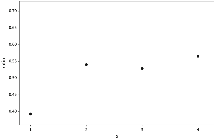
Fig. 3 Geometric ratio plot for the H5N1 outbreak data of Example 3
