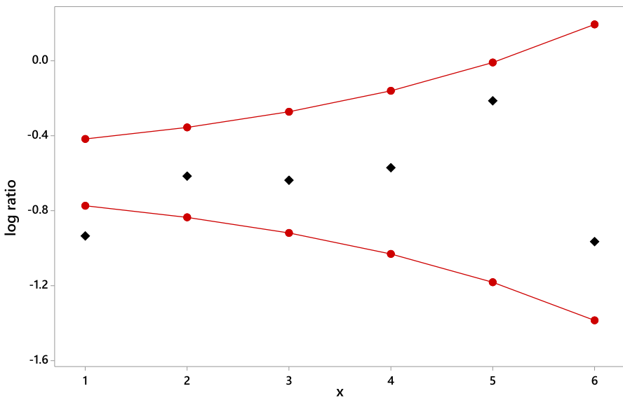
Fig. 4 Geometric ratio plot under the null for the H5N1 outbreak data of Example 3
