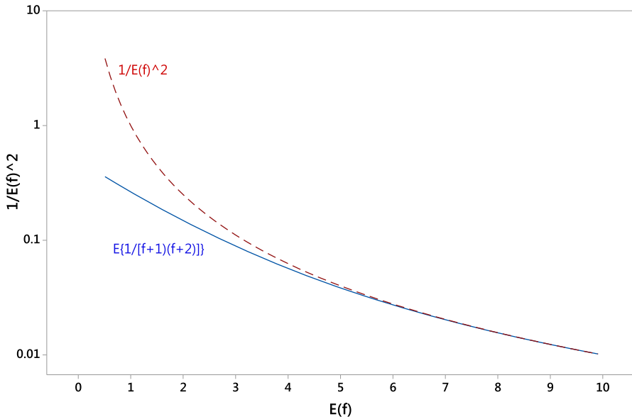
Fig. 9 E[1/(f+1)(f+2)]^2 and 1/E(f)^2 as a function of E(f)
