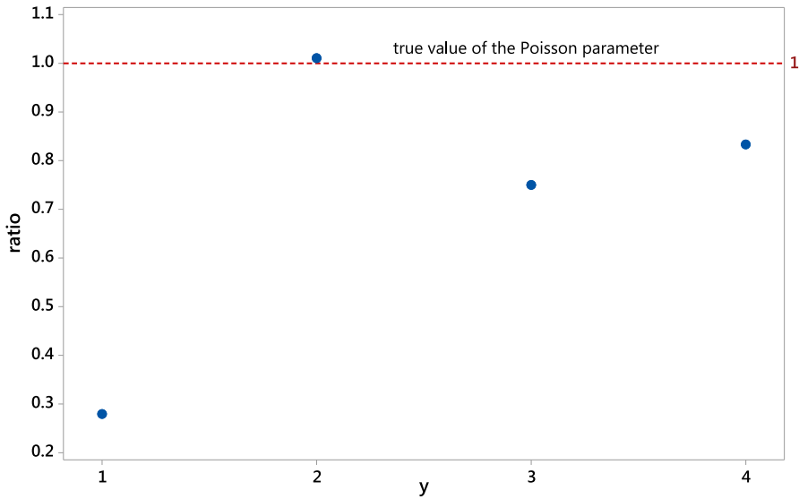
Fig. 2 Poisson ratio plot for the synthetic data of Example 2
