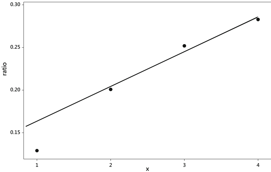
Fig. 1 Geometric ratio plot for perpetrator domestic violence identifications in the Netherlands 2009
