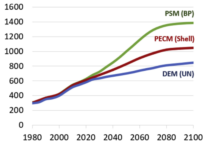
Fig. 4. Total primary energy of Shell's Sky scenario under different accounting methods. Comparison is made with production efficiencies from Table 1. Data from Ref. [11].
