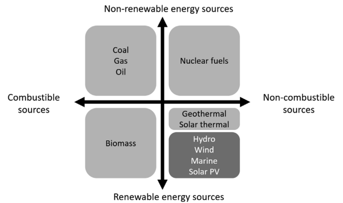
Fig. 3. Primary energy sources. Light grey areas indicates sources with heat as conversion step. Dark grey indicates sources that directly produce electricity. Marine includes wave and tidal energy, Wind includes off- and on-shore wind, Solar PV (Solar Photovoltaic).
