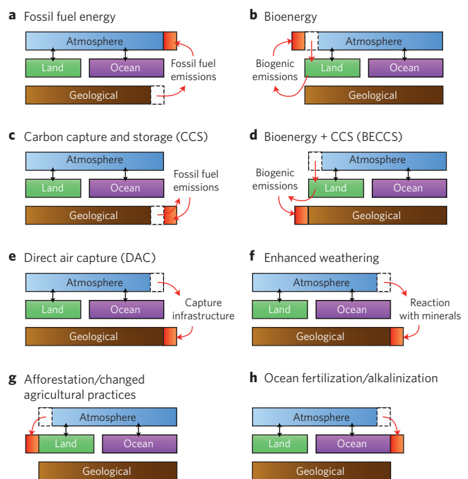
Figure 1 | Schematic representation of carbon flows among atmospheric, land, ocean and geological reservoirs.
