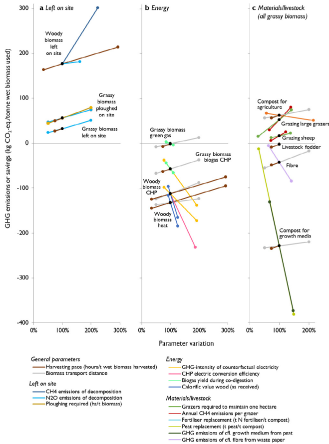
Fig. 5. Sensitivity analysis of total GHG emissions of residual biomass applications. Sensitivity to parameter variations is shown based on the percentage of change in the parameter range (x-axis) and the related GHG emissions or savings (y-axis). Parameter ranges are presented in Table 2.
