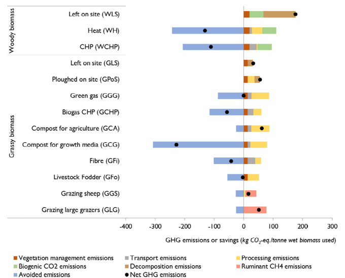
Fig. 3. GHG emissions and savings of current residual biomass applications at biomass scale. GHG emissions from various sources are presented as positive values. GHG savings, achieved through the replacement of counterfactuals, are presented as negative values. Net GHG emissions are the sum of emissions and savings and are presented as black dots. Climate change mitigation potential of residual biomass use.
