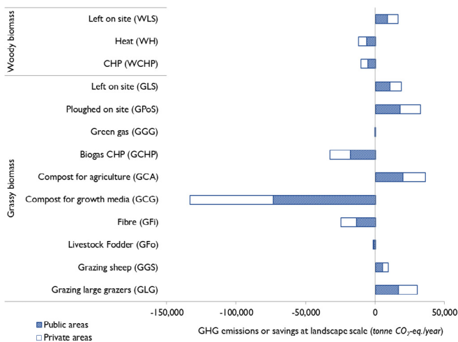
Fig. 4. GHG emissions and savings of current residual biomass applications at landscape scale. The total GHG emissions or savings of each application, multiplied with the biomass available in the study area (cf. Fig. 2) each year are shown. Biomass availability from publicly and privately-owned areas was distinguished which together represent the entire study area.
