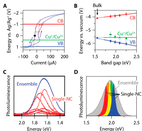
Figure 9. (A) Cyclic voltammetry measurements on CuInS 2 NCs in electrolyte solution in chloroform revealing a redox feature ascribed to the Cu + /Cu 2+ couple at approximately 0.5 V (vs. Ag/Ag + ). The conduction band (CB) and valence band (VB) edges are also indicated. (B) Potentials extracted for Cu + /Cu 2+ (green data points), the CB (red), and the VB (blue) for stoichiometric NCs with different band size. Linear trends are extrapolated to the bulk band gap, where the Cu + /Cu 2+ potential and the VB edge are approximately resonant. (C) Whitham et al. 75 measure single-nanocrystal emission bands with fwhm between 190 and 270 meV on a batch of CuInS 2 /CdS NCs with a slightly broader ensemble fwhm of 300 meV. (D) Zang et al. 67 measure emission spectra from single CuInS 2 /ZnS NCs with fwhm between 60 and 220 meV, much narrower than the ensemble fwhm of 352 meV. Colored lines are Lorentzian fits to the single-NC emission spectra, not the actual measurements. Panels A and B are adapted from ref 103. Copyright 2017 American Chemical Society. Panel C is adapted from ref 75. Copyright 2016 American Chemical Society. Panel D is adapted from ref 67. Copyright 2017 American Chemical Society.
