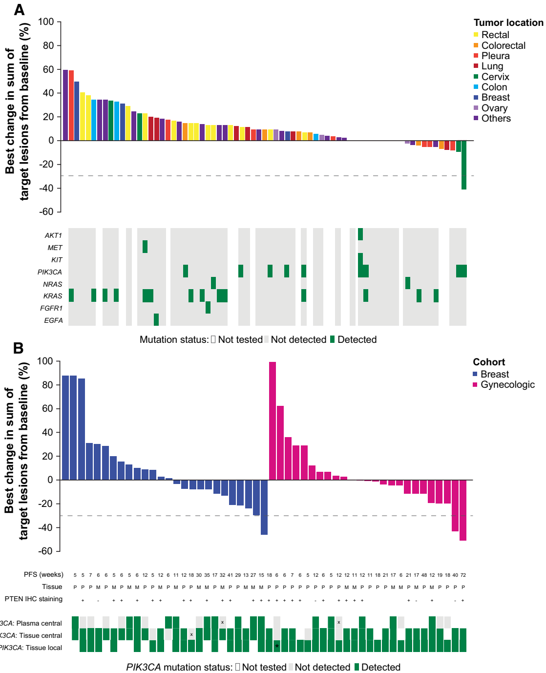
Figure 4. Waterfall plots of best percentage change in target lesion size from baseline in patients from (A) Parts A and B and (B) Part C, with associated molecular data. A, Exploratory mutation analysis by Sequenom in patients who provided suitable archival tumor tissue, who had baseline tumor assessment, and for whom best percentage change could be calculated. Mutations of potential interest in relationship to modulation of response to AZD5363 or known oncogenic drivers are shown. The AKT1 mutation detected in 1 patient was Q43X. B, Progression-free survival (PFS), PIK3CA -mutation status by local testing (tissue), central testing (cobas PCR, tissue and plasma), and PTEN status (immunohistochemistry, tissue) are shown. Only patients with baseline tumor assessment and measurable disease and for whom best percentage change could be calculated are included in the plot. The type of tissue used for central and exploratory assessment is indicated (M = metastatic, P = primary). Additional exploratory data on PIK3CA and ESR1 mutation testing in ctDNA by ddPCR are described in Supplementary Table S4 (including time lapse between tissue biopsy and plasma collection) and in the Supplementary Material.
