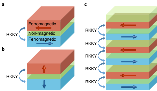
Fig. 1 | Schematic of synthetic antiferromagnets. a , Bilayers with in-plane magnetization. b , Bilayers with out-of-plane magnetizations. c , Multilayers. The arrows within each ferromagnetic layer indicate the direction of magnetization. Depending on the magnetic configurations the RKKY coupling and dipolar fields add ( a ) or subtract ( b ), leading in part to the large degree of tunability of multilayers.
