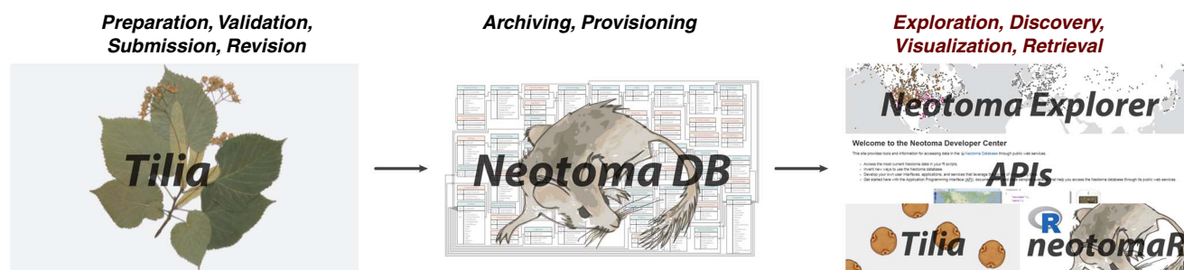
Figure 4. (color online) Diagram of the Neotoma software ecosystem. Data preparation and cleaning for upload to Neotoma are handled by the Tilia software ( https://www.tiliat.com/ ), which has password-protected access for data stewards to upload data sets, update age models, and correct errors. Data are stored in the Neotoma relational database, which is deployed in SQL Server and currently hosted at Pennsylvania State University's Center for Environmental Informatics. Neotoma data can be discovered, explored, viewed, and obtained through multiple platforms. Neotoma Explorer and its graphical map-based interface is designed for first-pass data explorations, new users, and educational and student groups. The application programming interfaces (APIs) and neotoma R package are intended for programmatic access and for users who wish to do large-volume searches of Neotoma data holdings. Tilia can also download data sets from Neotoma, which is useful for data visualizations and for data stewards needing to update data sets or looking for examples of prepared Tilia files.
