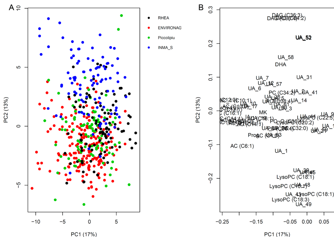
Figure 3. PCA analysis of significant metabolites. (A) Scores scatter plot of first two components, colored by cohort. (B) Loadings scatterplot of first two components. Abbreviations: AC: acylcarnitine, UA: unassigned, PC: phosphatidylcholine, LysoPC: lysophosphatidylcholine, Prog: progesterone, Ret: retinol, DAG: diacylglycerol, IA: indolelactic acid, MK: methoxykynurenate, DHA: docosahexaenoic acid. Numbers following unassigned compounds refer to compound numbers (see Table S1).
