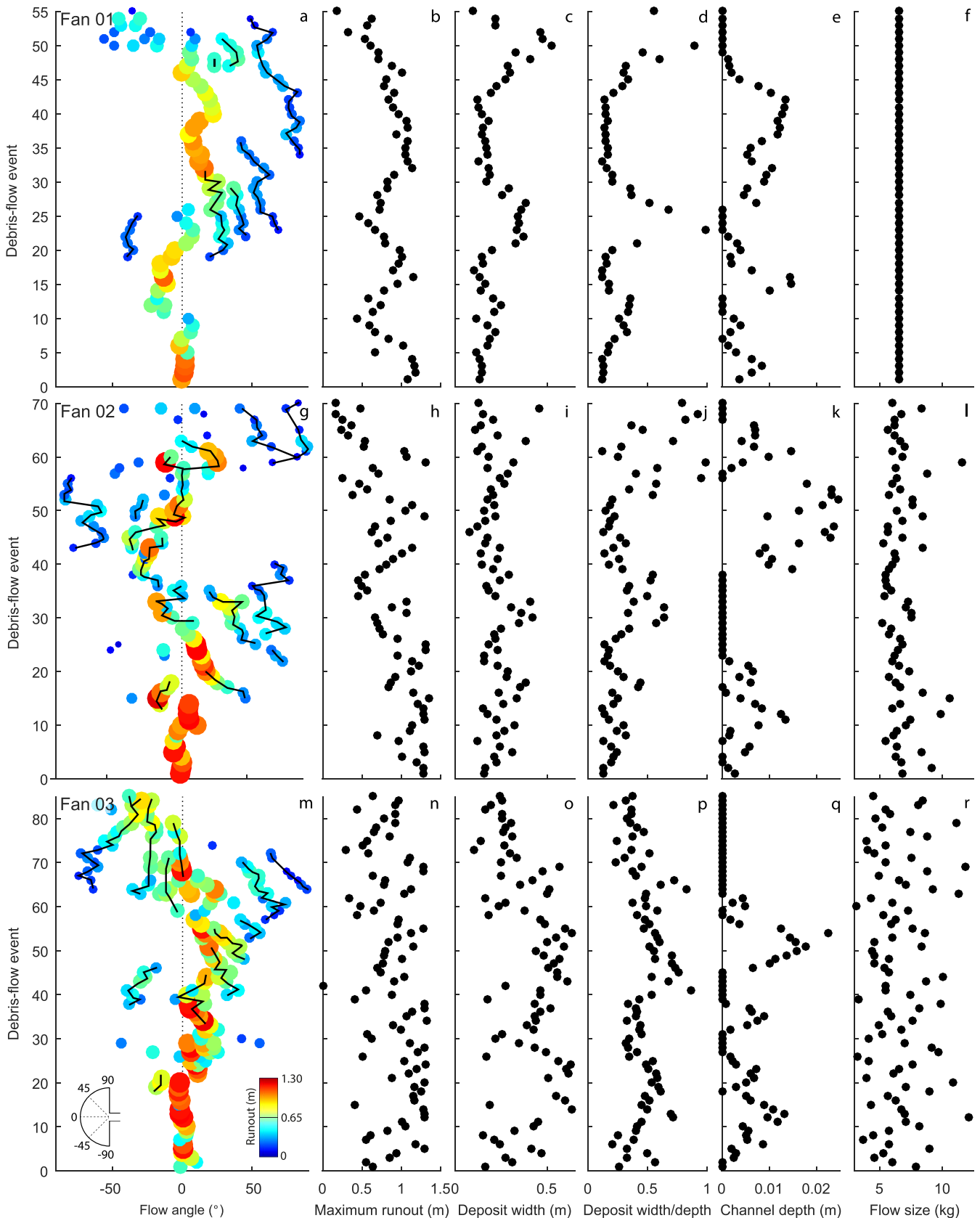
Figure 5. Summary of the spatio-temporal patterns of debris-flow activity on fans 01–03. (a) Flow angle and runout distance of the channels active during the debris-flow events that formed fan 01. Flow angle was previously published in De Haas et al. (2016); the other variables are newly reported here. Solid line segments join successive flows in the same channel. (b) Maximum runout distance during each debris flow on fan 01. (c) Deposit width during each event on fan 01. (d) Deposit width/depth ratio for each debris flow on fan 01, defined as deposit width divided by maximum runout distance. (e) Channel depth after each debris-flow event on fan 01, measured 10 cm downstream of the fan apex. (f) Debris-flow mass in kilograms. (g–l) As above for fan 02. (m–r) As above for fan 03. [Colour figure can be viewed at wileyonlinelibrary.com ]
