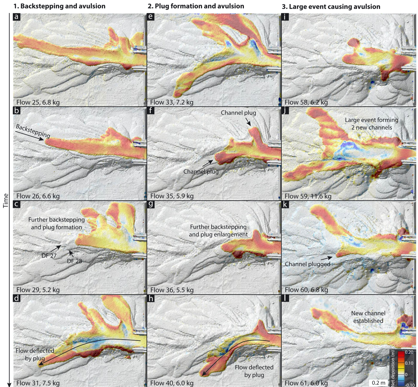
Figure 7. Common debris-flow–magnitude sequences leading to avulsion on fan O2, formed by a steep-tailed double-Pareto flow distribution (Figure 3b). (a–d) Backstepping and avulsion sequence during debris flows 25–31. A sequence of small- to moderate-sized flows induced a sequence of backstepping deposition (b, c), which was followed by avulsion during the large flow 31 (d). (e–h) Channel plug formation by two small debris flows that blocked the main channel (f, g), followed by avulsion during a moderate-sized flow (h). (i–l) A very large debris flow created two new channels (j), one of which became blocked by a flow snout in the next, smaller flow (k). Avulsion then proceeded into the topographically favored right-hand channel (l). [Colour figure can be viewed at wileyonlinelibrary.com ]
