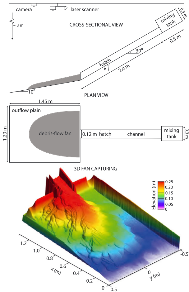
Figure 1. Experimental flume setup. The 3D fan image shows the final morphology of fan 01. The flume setup is similar to that used in De Haas et al. (2015b, 2016). Figure modified from De Haas et al. (2016). [Colour figure can be viewed at wileyonlinelibrary.com ]
