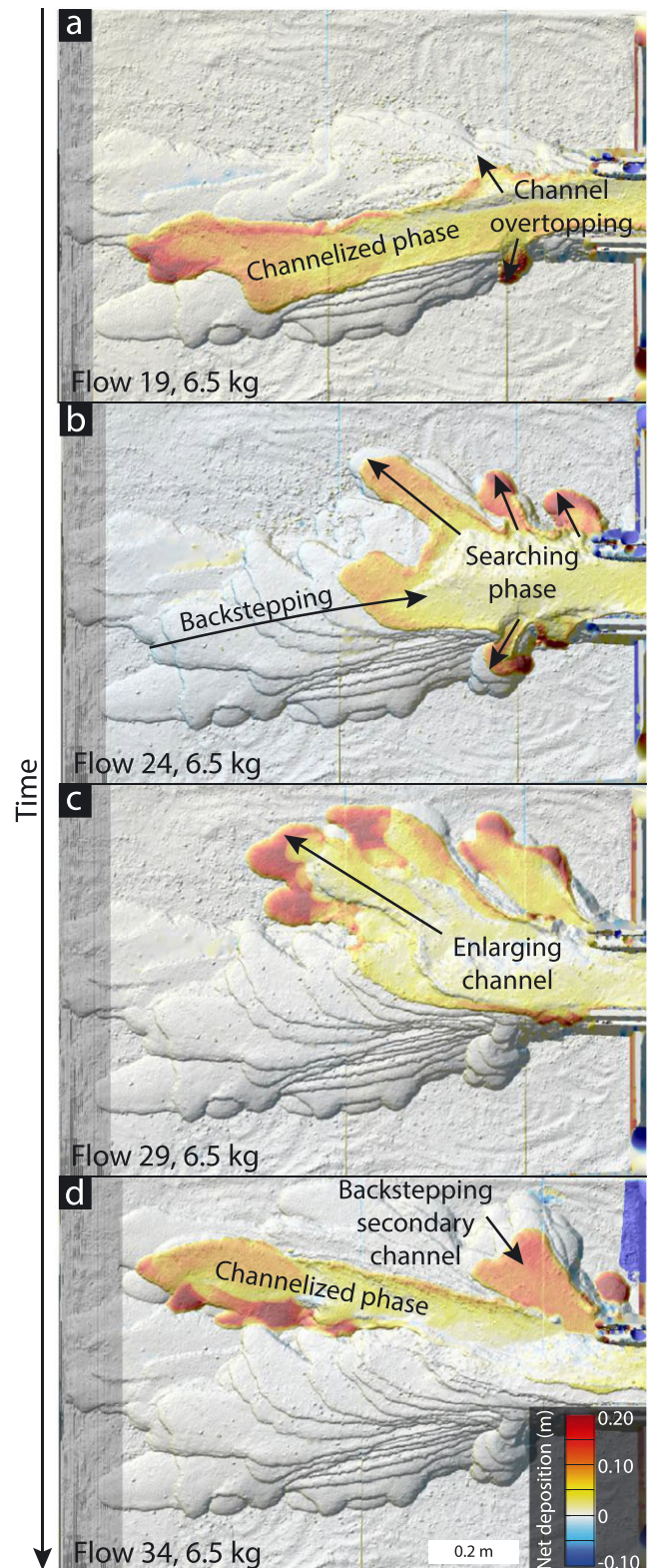
Figure 6. Typical avulsion sequence on fan 01, formed by a uniform flow magnitude-frequency distribution (Figure 3a). The sequence shows evolution from a well-defined channel (a) through gradual backstepping of deposition toward the fan apex, followed by a searching phase (b), avulsion to a new channel pathway and enlargement (c), and channelization (d). Note that a secondary channel formed but was plugged and abandoned during this sequence. [Colour figure can be viewed at wileyonlinelibrary.com ]
