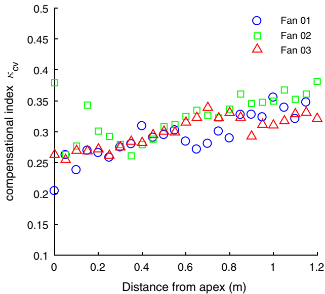
Figure 10. Compensation index from fan apex (left) to fan toe (right) for fans 01–03. [Colour figure can be viewed at wileyonlinelibrary.com ]
