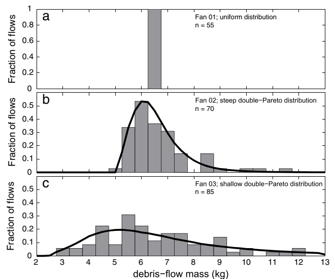
Figure 3. Magnitude–frequency distributions of the experimental debris-flow fans. The lines denote the double-Pareto distributions from which the debris-flow magnitudes were randomly extracted. The bars denote the actual number of events in each experiment, divided into 0.5 kg bins. The mean debris-flow mass is \sim 6.5 kg for all experiments: (a) fan 01 with a uniform distribution; (b) fan 02 with a steep-tailed double-Pareto distribution; (c) fan 03 with a shallow-tailed double-Pareto distribution.
