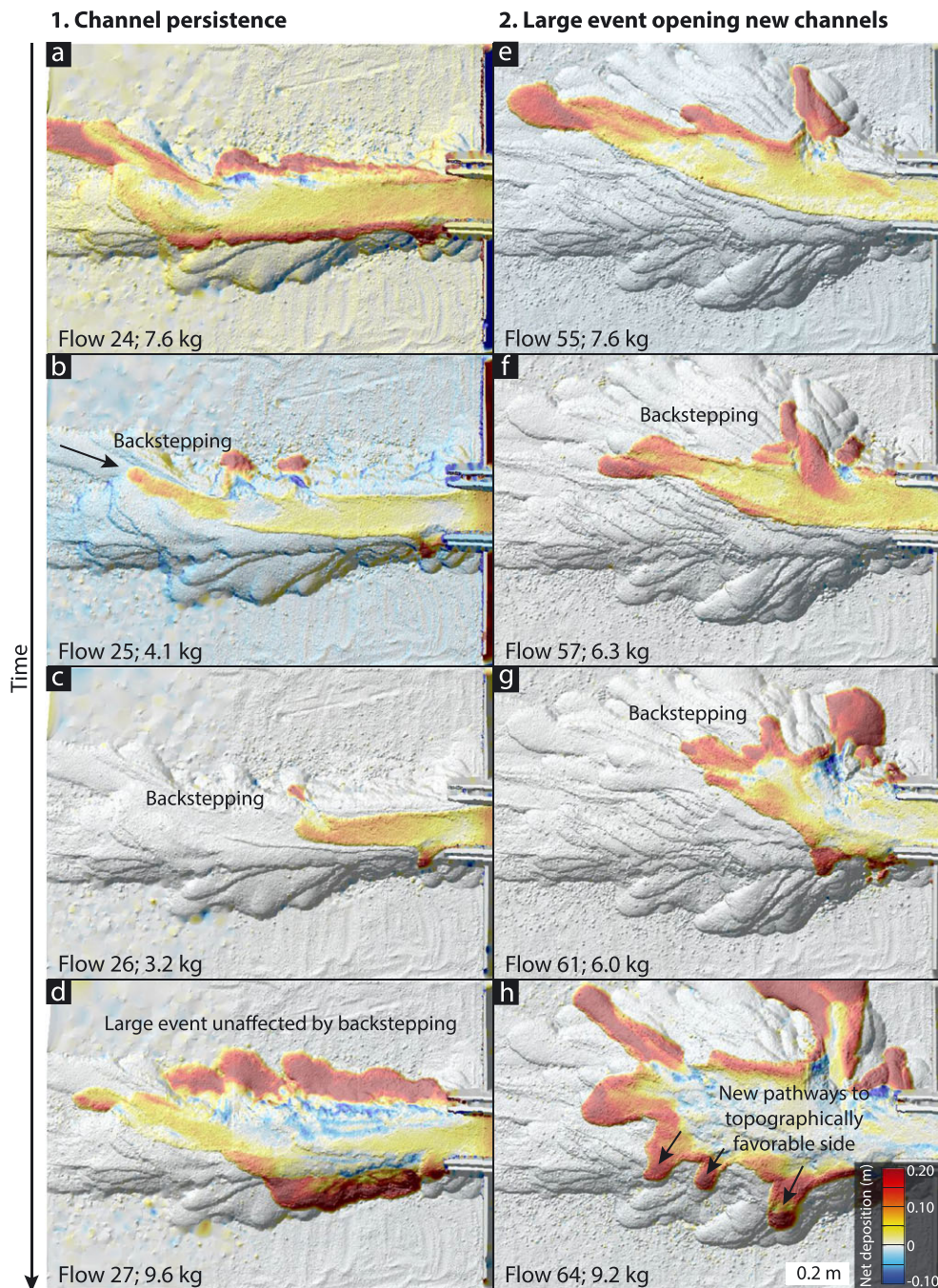
Figure 8. Common spatio-temporal patterns of debris-flow activity on fan 03, formed by a shallow-tailed double-Pareto flow distribution (Figure 3c). (a–d) Persistent channel position during debris flows 24–27. The direction of the large debris flow 27 (d) was unaffected by the backstepping plug deposits from the small flows 25 and 26 (b, c). Flow 27 partly eroded the channel plug and filled the channel surrounding the plug. Overbank surges were widespread during the relatively large flows 24 and 27 (a, d). (e–h) After a partial backstepping sequence from debris flow 55 to 62 (e–g), large flows 63 and 64 opened up three new channel pathways on the left side of the fan (h, shown by arrows) that allowed subsequent avulsion towards the left. [Colour figure can be viewed at wileyonlinelibrary.com ]
