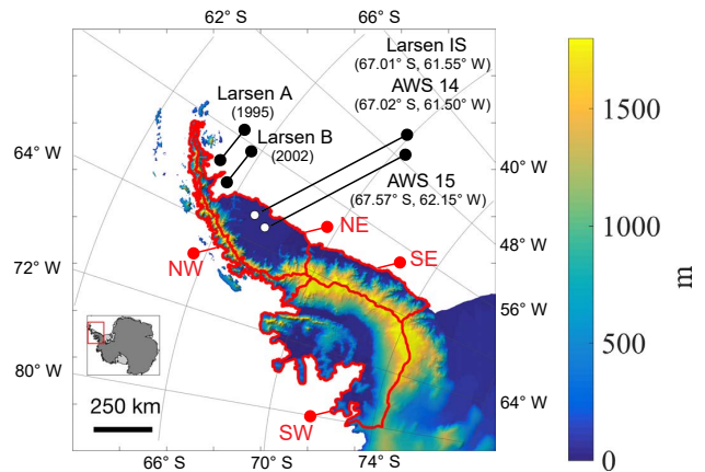
Figure 1. Full MAR domain showing topographic relief from bedmap2 ( https://www.bas.ac.uk/project/bedmap-2 , last access: November 2017) at 1 km, former ice shelves with dates of collapse, locations of automatic weather stations (Larsen IS and AWS 14 stations are located within the same MAR grid-cell) and basins corresponding to SW (basin 24), NW (basin 25), NE (basin 26), and SE (basin 27) from Zwally et al. (2012).
