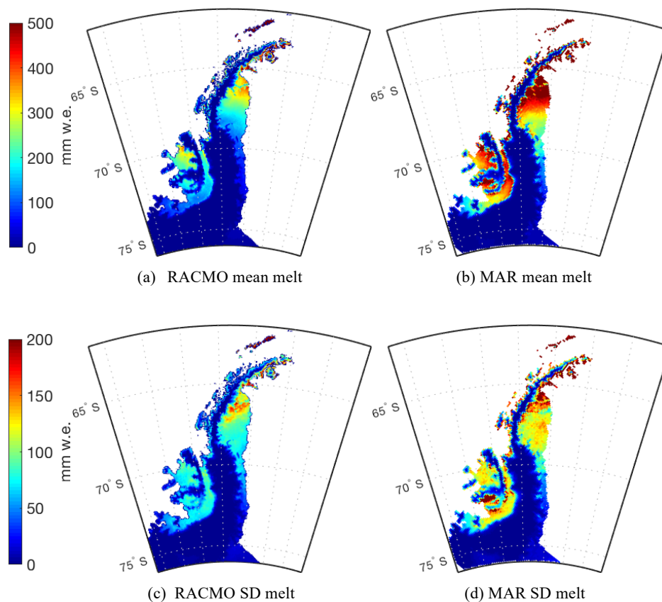
Figure 3. Meltwater production (2000–2009). RACMO2.3p2 at 5.5 km resolution, mean annual meltwater production (a), and standard deviation (c); and MAR v. 3.5.2 at a 10 km resolution, mean annual meltwater production (b), and standard deviation (d).
