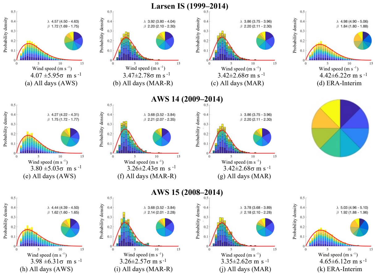
Figure 8. Probability distribution (y axis) of summer (DJF) wind speeds (x axis) and direction proportions inset. Wind directions corresponding to colours in 45° increments shown right of (g). Curve shows Weibull curve shape ( \beta ) and scale ( \lambda , m s -1 ). Datasets for AWS (col 1), MAR-R (col 2), MAR from 1999–2014 period (col 3), and ERA-Interim for the AWS-restricted period (col 4). Shown for station Larsen IS (row 1, a, b, c, d), AWS 14 (row 2, e, f, g), AWS 15 (row 3, h, i, j, k). Values below figures are expected values.
