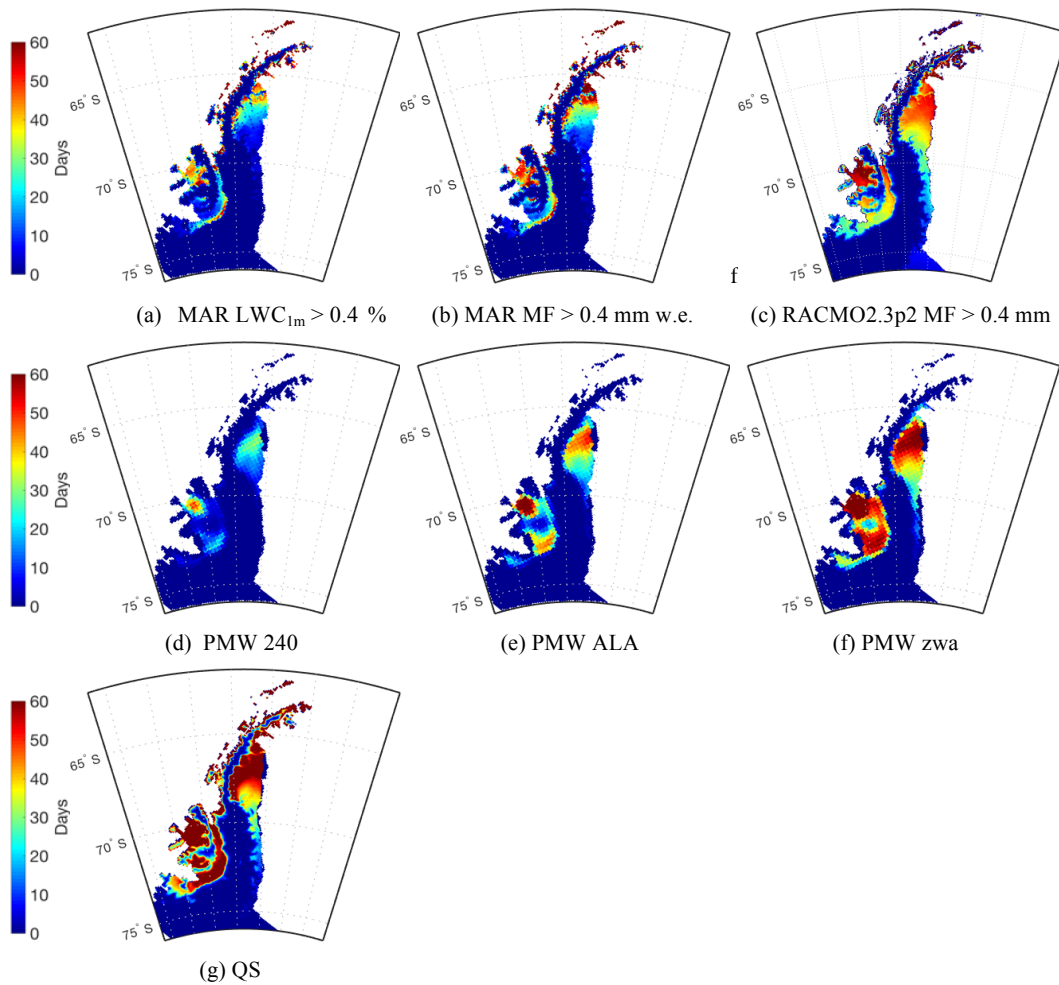
Figure 5. Average number of melt days (2000–2009) from multiple sources (a) MAR, liquid water content > 0.4\% for three consecutive days. (b) MAR total melt flux > 0.4 mm w.e. for 1 day or more (c) RACMO2.3p2, Melt Flux > 0.4 mm w.e. Satellite-based metrics include (d) PMW 240 algorithm, (e) PMW ALA, and (f) PMW Zwa (g) QuikSCAT. All satellite-based estimates include a melt day only when part of a sustained three-day period of melt.
