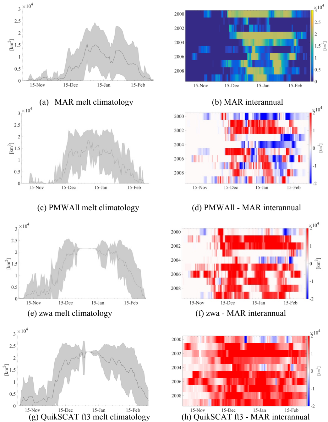
Figure 6. CL-region, described in text and shown in inset in for (a), average and inter-annual melt occurrence in MAR, PMW, and QuikSCAT data. (a) MF0.4 melt extent climatology with one standard deviation shown in grey envelope. (b) Melt extent for MF0.4 from 1999–2009. (c) Melt climatology PMW All. (d) Interannual difference melt extent PMWAll – MAR. (e) Melt climatology PMW zwa. (f) Interannual difference in melt extent PMWzwal – MAR. (g) Melt climatology QuikSCAT ft3. (h) Interannual difference in melt extent QuikSCAT ft3 – MAR.
