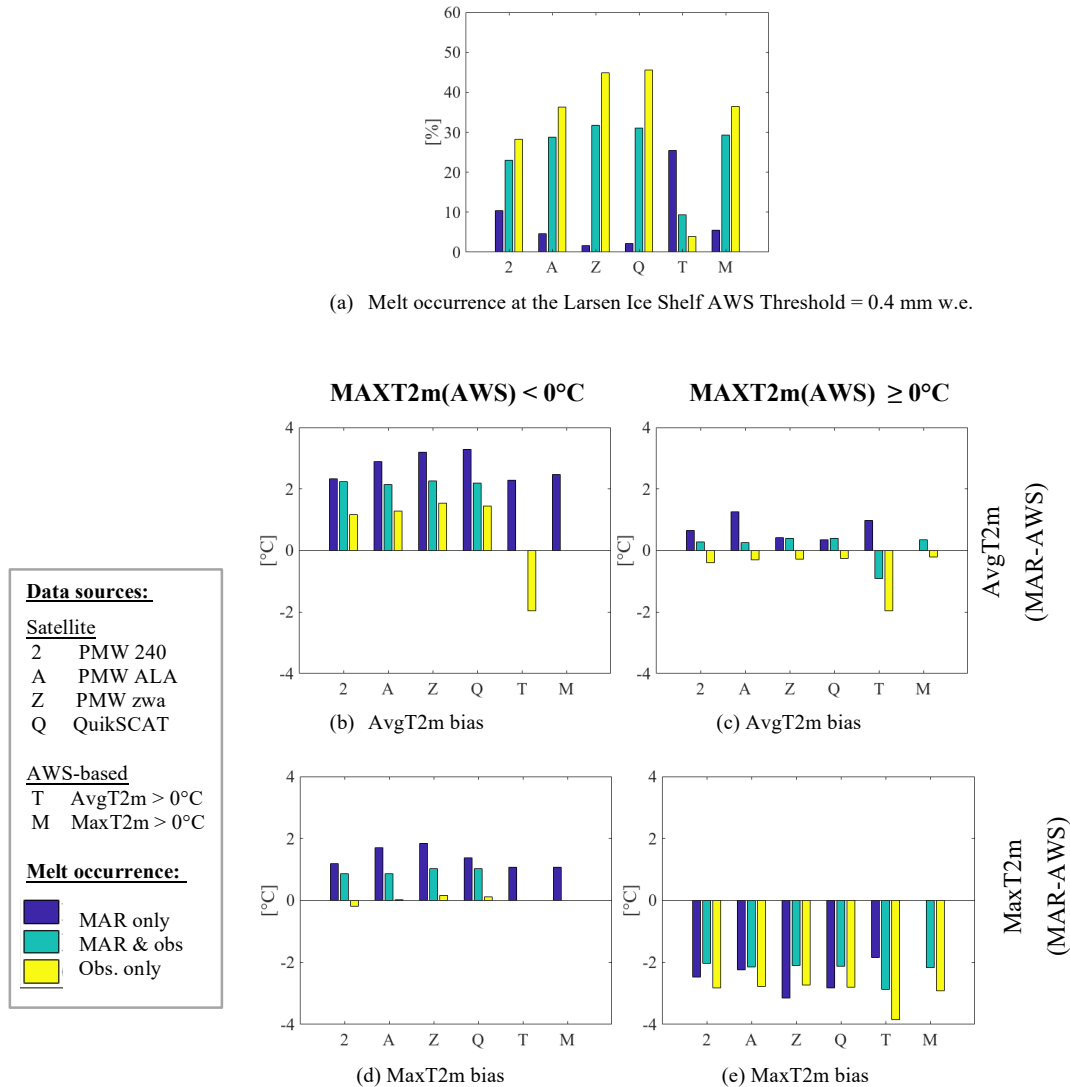
Figure 4. Melt occurrence and temperature biases at the Larsen Ice Shelf AWS Station. Percentage of total days (DJF, 2001–2010) showing melt occurrence from observational sources as compared to MAR v3.5.3 melt occurrence using the MF 0.4 metric (a). Temperature biases (MAR-AWS) for AvgT2m (b, c) and MaxT2m (d, e), when Max T2m is less than 0 °C (b, d) or greater than 0 °C (c, e).
