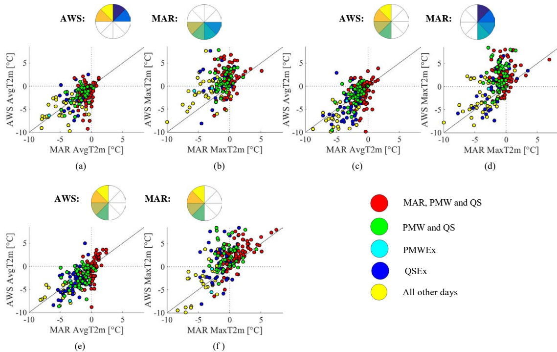
Figure 9. MAR vs. AWS temperatures at the Larsen Ice Shelf AWS station for DJF from 2001–2009 for melt occurrence criteria as shown bottom-right and described in text. Wind direction biases are shown for when northerly AWS flow is reported as southerly in MAR (a) AvgT2m (b) MaxT2m, when westerly AWS flow is reported as easterly in MAR (c) AvgT2m (d) MaxT2 and when AWS and MAR both report westerly flow (e) AvgT2m (f) MaxT2m.
