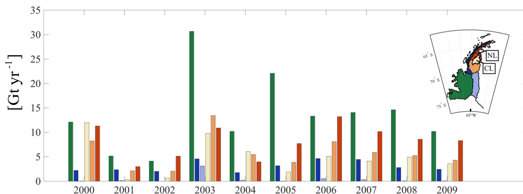
Figure 2. Annual meltwater production from MAR [ \text{Gt yr}^{-1} ] shown for masks shown in inset (“2001” corresponds to meltwater production from July 2000–June 2001). NW, SW, and SE basins are shown as in Fig. 1. NE basin is divided into the NL mask, the CL mask and the remaining portion of the NE basin ( \text{NE} - (\text{CL} + \text{NL}) ). The CL and NL masks are described in text.
