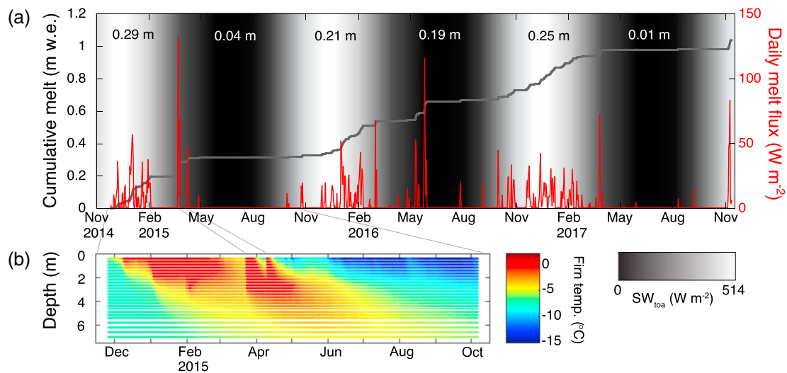
Figure 2. (a) Daily mean melt flux ( \text{W}/\text{m}^2 , red) and cumulative melt (m w.e., gray) for November 2014 to November 2017, computed from automatic weather station observations. Background gradient shows daily mean top-of-atmosphere incoming solar radiation, SW_{\text{toa}} : black is 0, white is 514 \text{ W}/\text{m}^2 . Text labels in the top of the panel denote cumulative melt (m w.e.) for austral summer (1 November to 31 March) and winter (1 April to 31 October) seasons. (b) Thermistor string observations of firn temperature ( ^{\circ}\text{C} ) as a function of depth (m), in 2015.
