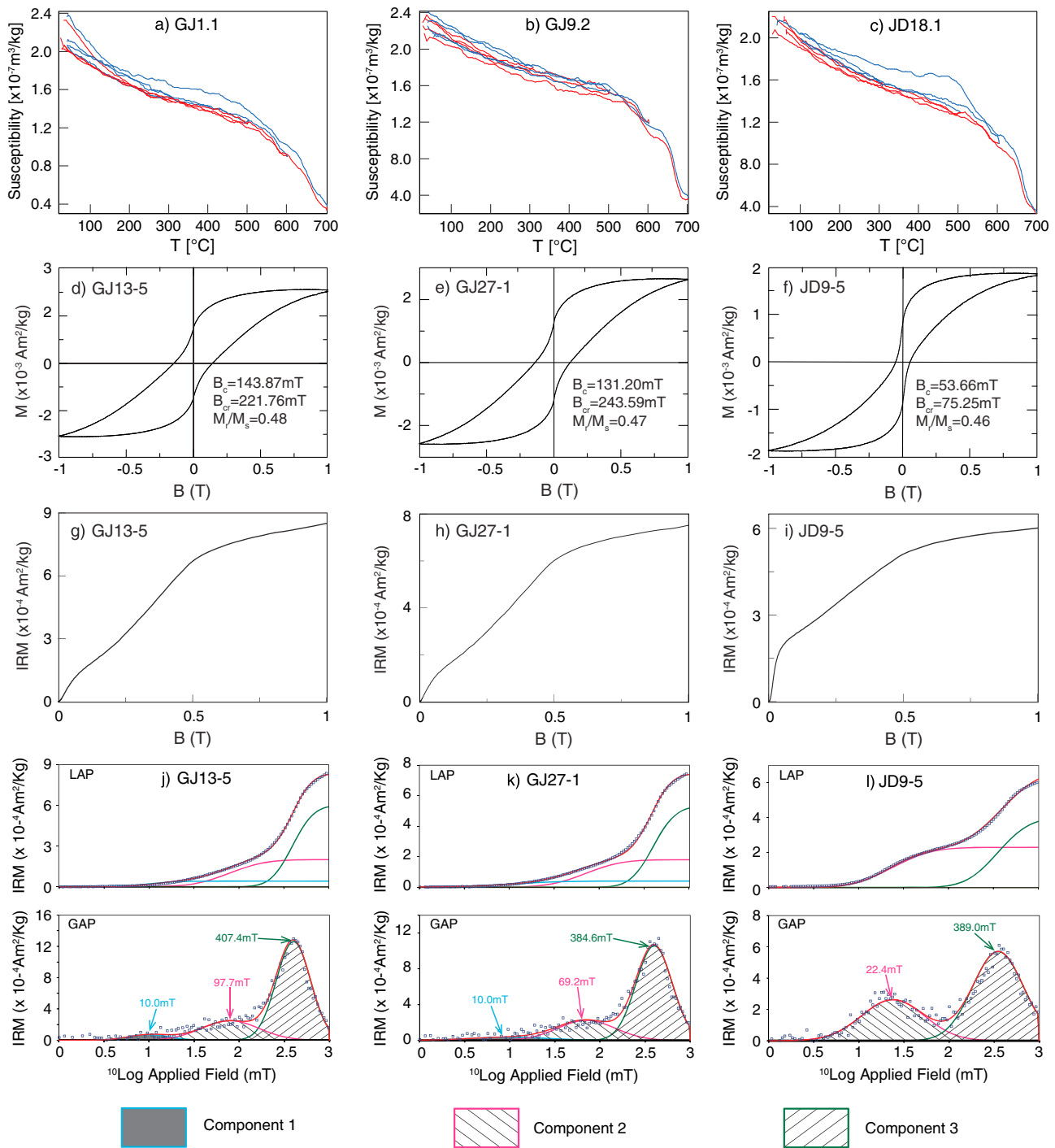
Figure 3. (a–c) Stepwise heating (red) and cooling curves (blue) of magnetic susceptibility in air for representative specimens. (d–i) Hysteresis loops and IRM acquisition curves for characteristic samples. (j–l) Isothermal remanent magnetization component analysis results of typical specimens with 150 data points acquired (Kruiver et al., 2001a). M, magnetization; B, magnetic induction; LAP, linear acquisition plot; GAP, gradient acquisition plot.
