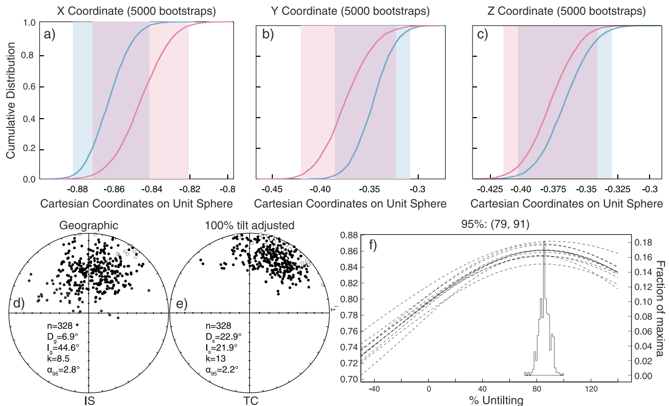
Figure 8. Nonparametric reversals test (a–c) and fold test (d–f) of ChRM directions isolated from the red beds from both Gongjue and Ranmugou formations in the Gongjue Basin (Tauxe, 2010; Tauxe & Watson, 1994).
