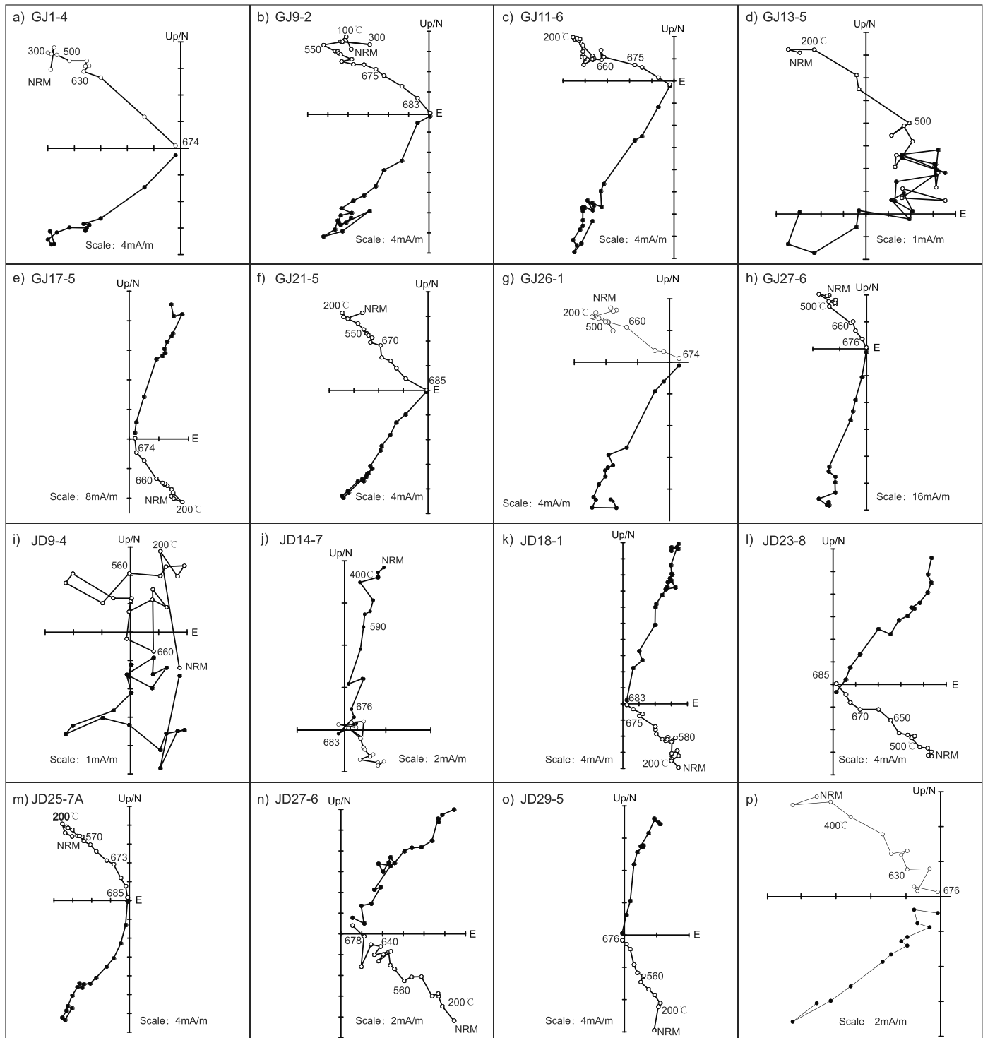
Figure 6. Representative demagnetization diagrams for specimens from the red beds in the Gongjue basin. All diagrams are displayed in stratigraphic coordinates. Closed (open) symbols represent declination (inclination).
