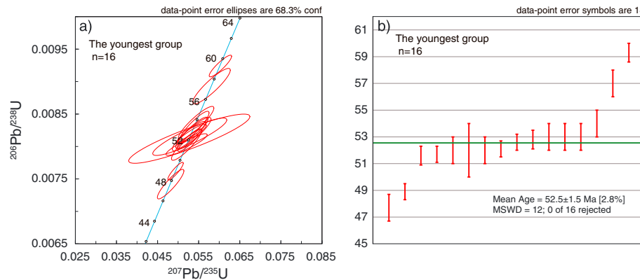
Figure 2. Concordia plots (a) and mean average (b) of the U-Pb dating of the 16 youngest detrital zircons from three samples (GJ24, JD8, and JD21). MSWD, mean square weighted deviation.
