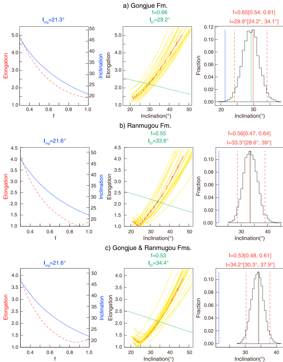
Figure 9. Correction for the inclination error of the ChRMs from the Gongjue formation (a), the Ranmugou formation (b), and the combined two formations (c) using the E/I method (Tauxe & Kent, 2004).
