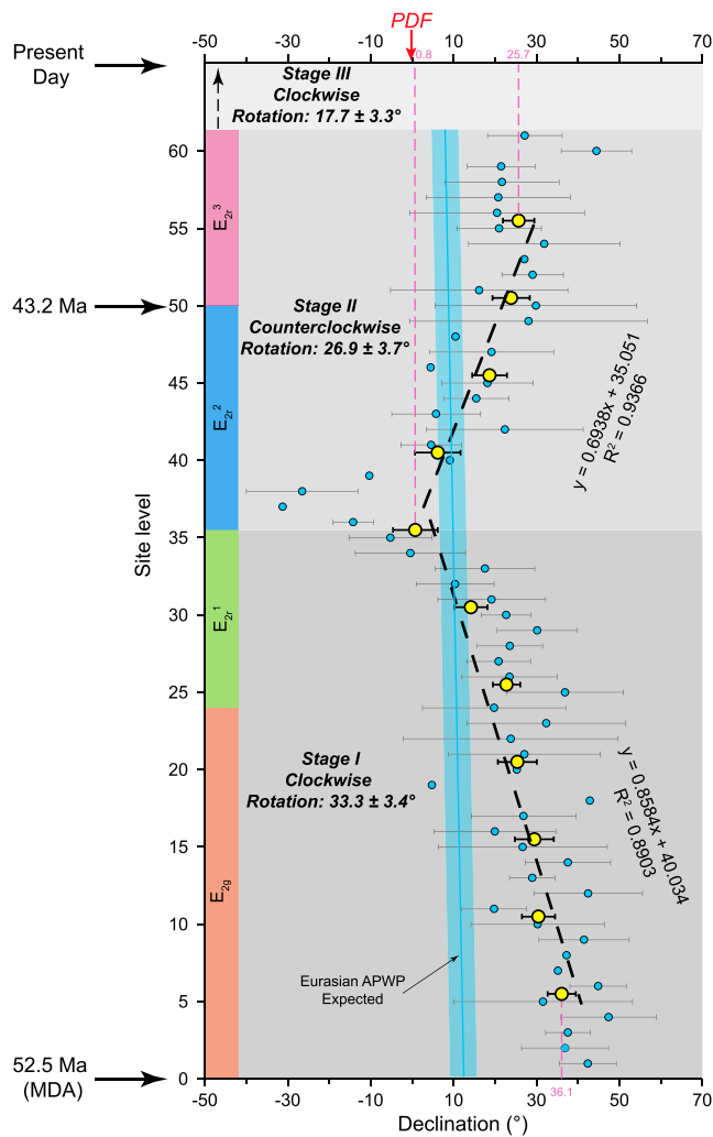
Figure 10. Stratigraphic analyses of the declinations and error bars of site-mean (blue dots) and 10 successive sites sliding window-mean (yellow dots) ChRM directions of the red beds in the Gongjue basin. Sites are plotted according to the site level; the distance of adjacent sites is assigned to be “1.” Details of the calculation can be found in the main text and Table S6. MDA, maximum depositional age; PDF, present day geomagnetic field.
