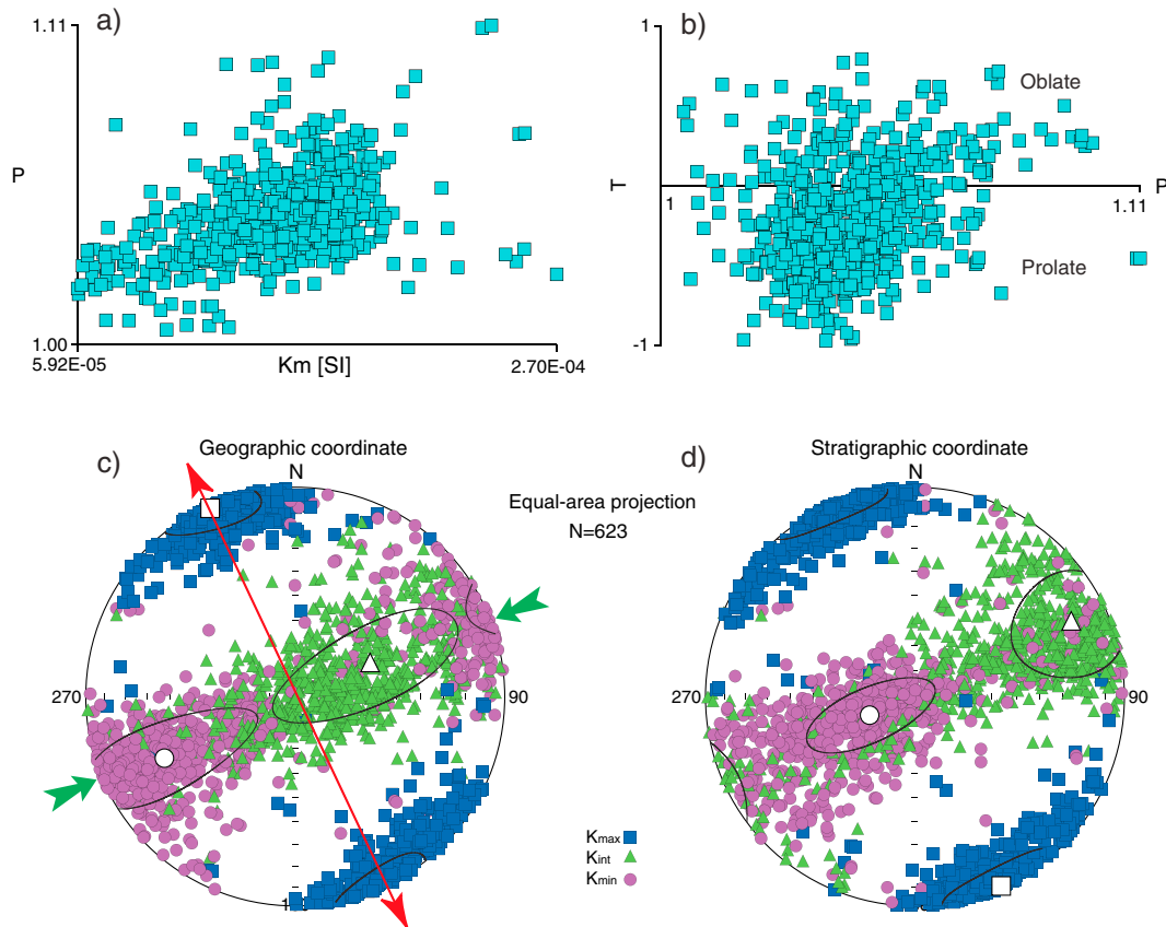
Figure 4. Magnetic fabric studies of the red beds in the Gognjue basin based on AMS measurements. (a) Magnetic susceptibility ( K_m ) versus anisotropy ( P ) plot. (b) Anisotropy ( P ) versus shape parameter ( T ) plot. (c, d) Stereoplots of the AMS results in geographic (c) and stratigraphic (d) coordinates. Solid symbols, individual directions; open symbols, mean directions with 95% confidence limit. The green and red arrows represent the inferred compression and extension directions, respectively.
