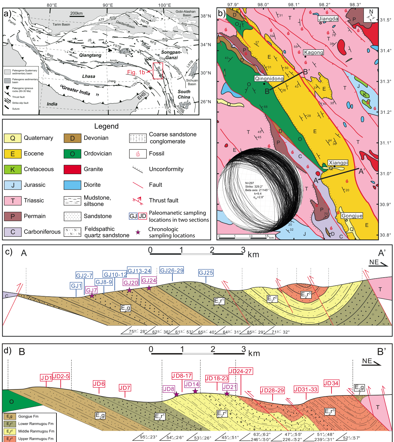
Figure 1. (a) Simplified tectonic map of the Tibetan Plateau, modified from Spurlin et al. (2005). ASRR, Ailao Shan-Red River fault; JS, Jinsha suture; BNS, Banggong-Nujiang suture; YZS, Yarlung Zangbo suture; EHS eastern Himalayan syntaxis; other abbreviations are the same as Spurlin et al. (2005). (b) Geological map of the Gongjue basin and surrounding area. (c, d) Profile of the two sampled sections in the middle and southern part of the basin. E_{2g} , Gongjue formation; E_{2r}^1 , lower/middle/upper of the Ranmugou formation.
