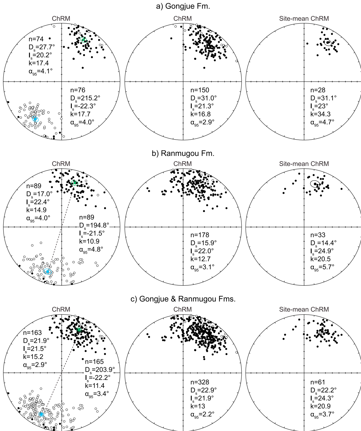
Figure 7. (a) Equal-area projections of individual ChRM directions (tilt corrected) from the Gongjue formation with both normal and reversed polarities (left), equal-area projections of ChRMs with reversed polarity transformed to antipodal directions (middle), and equal-area projections of site mean ChRMs with reversed polarity transformed to antipodal directions (right). (b) The same plots for individual ChRM directions from the Ranmugou formation (b) and combined two formations (c). Dots and circles represent mean ChRM directions and corresponding 95% confidence limit, respectively.
