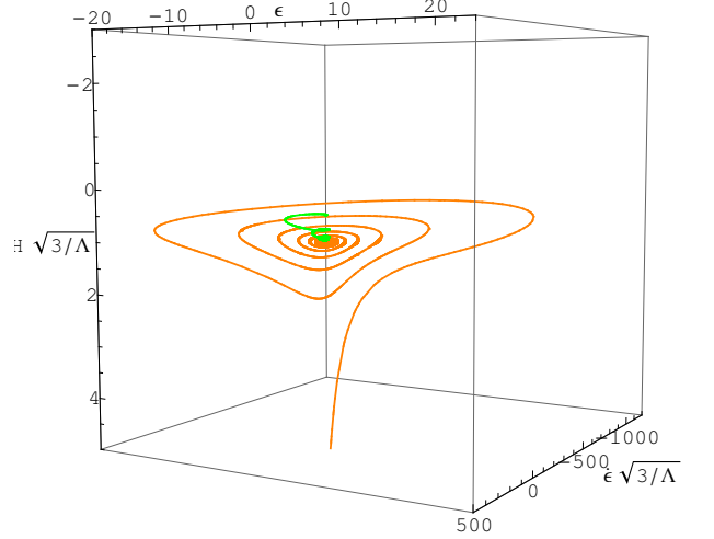
Figure 10: Parametric phase space plot for figure 9 in which the classical attractor is stable. Because of under-damping, one spirals towards the classical attractor. For clarity, we have only included the flow for two initial conditions H(0) = \sqrt{3}/\Lambda/2 and H(0) = 6\sqrt{3}/\Lambda . The twister like structure is clearly visible. Qualitatively, the phase space flow resulting from other initial conditions is identical.
