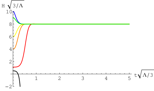
Figure 7: Dynamics of the Hubble parameter taking the full trace anomaly into account. We took b'' = 0 such that b'' - 2b'/3 > 0 yielding an unstable classical attractor. We have used \omega = 0 , \lambda = 1/50 , b' = -0.015 (Standard Model value).
