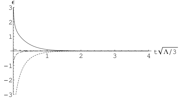
Figure 2: Validity of the assumption \epsilon \ll 1 . For the various initial conditions in figure 1, one can clearly see that this approximation is well justified.
