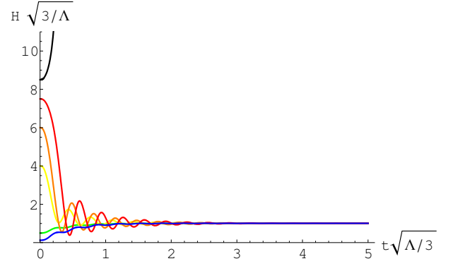
Figure 9: Dynamics of the Hubble parameter taking the full trace anomaly into account. We took b'' = b' such that b'' - 2b'/3 < 0 yielding a stable classical attractor. We have used \omega = 0 , \lambda = 1/50 , b' = -0.015 (Standard Model value). Clearly, the classical attractor is under-damped, resulting in various oscillations around H_0^C .
