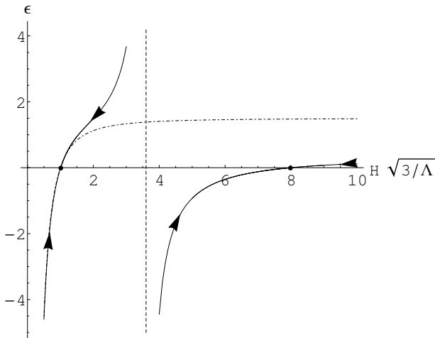
Figure 5: Phase space flow in quasi de Sitter spacetime. The phase space consists of two lines. The flow, indicated by the arrows, is towards the classical or quantum attractor represented by two dots. In this regime, both attractors are stable. The vertical dashed line indicates the branching point and the dashed-dotted line the classical evolution. We have used \omega = 0 , \lambda = 1/50 , b' = -0.015 (Standard Model value) and b'' = 0 .
