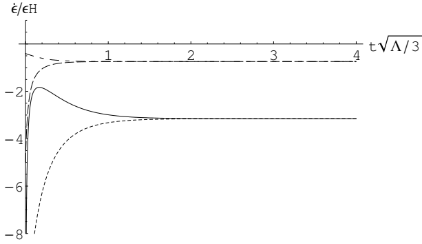
Figure 3: Validity of the assumption \dot{\epsilon} = 0 . For the various initial conditions in figure 1, we have calculated \dot{\epsilon}/(H\epsilon) . Clearly, this condition is violated at all times.
