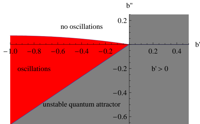
Figure 11: Parameter space for oscillations around the quantum anomaly driven attractor. The gray region (light shaded) is excluded either because b' > 0 or because the quantum attractor has become unstable. The red region (dark shaded) in parameter space shows oscillatory behaviour, whereas the white region is either critically damped or over-damped. We used \lambda = 1/50 .
