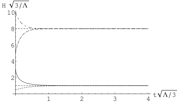
Figure 1: Dynamics of the Hubble parameter in quasi de Sitter spacetime in the presence of a non-zero cosmological constant, the trace anomaly, and matter ( \omega = 0 ). Depending on the initial conditions, the Hubble parameter evolves to either the classical de Sitter or the quantum anomaly driven attractor. We have used \lambda = 1/50 , b' = -0.015 (Standard Model value) and b'' = 0 .
