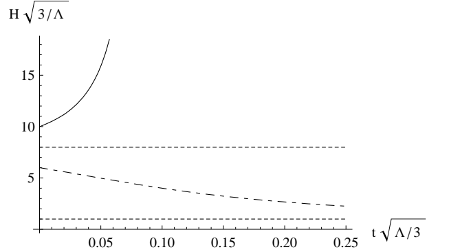
Figure 4: Instability of the quantum anomaly driven attractor in quasi de Sitter spacetimes. We have used \lambda = 1/50 , \omega = 1/3 , b'' = 7b'/6 < 5b'/6 .
