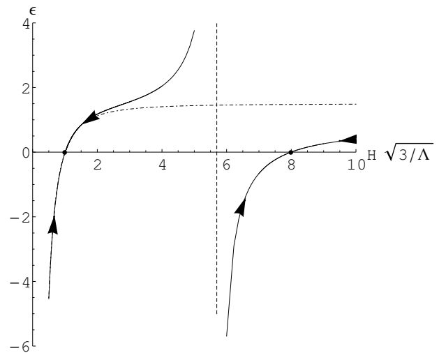
Figure 6: Phase space flow in quasi de Sitter spacetime for b'' = 2b'/3 such that the \square R does not contribute in the trace anomaly. Qualitatively, the dynamics does not change when compared to figure 5. Again, both attractors are stable. Apart from b'' , the value of the parameters are identical to figure 5.
