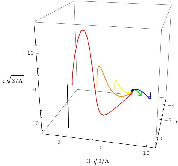
Figure 8: Parametric phase space plot for figure 7 in which the classical attractor is unstable. We have indicated the quantum anomaly driven attractor as a small black sphere.
