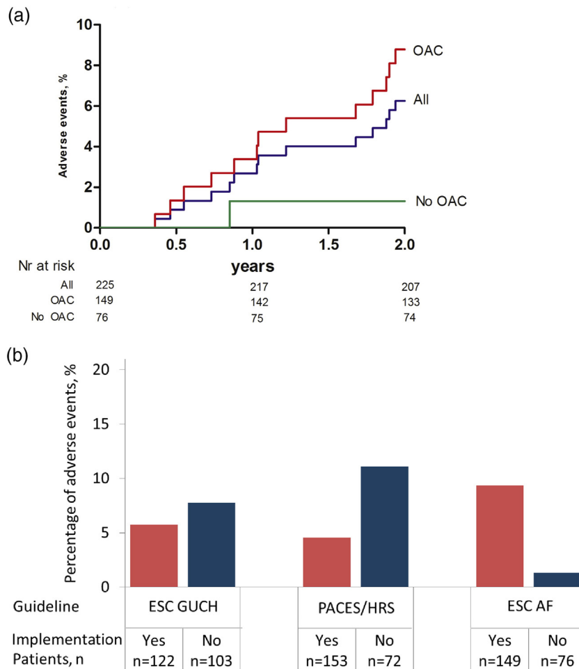
Fig. 2. a. Kaplan-Meier estimates of any adverse events in ACHD patients with atrial arrhythmias. Any adverse events were defined by death, thromboembolism and major bleeding. Adverse events are analyzed according to whether the patients were using oral anticoagulants. Abbreviations: ACHD = adult congenital heart disease, OAC = oral anticoagulants b. Percentage of adverse events in ACHD patients with atrial arrhythmias. Percentages of adverse events are illustrated according to whether the guidelines were implemented or not. Abbreviations: ESC GUCH = 2010 European Society of Cardiology (ESC) guidelines for the management of grown-up congenital heart disease, PACES/HRS = 2014 Pediatric and Congenital Electrophysiology Society (PACES)/Heart Rhythm Society (HRS) recognition and management of arrhythmias in adult congenital heart disease (PACES/HRS), ESC AF = 2016 ESC guidelines for the management of atrial fibrillation.
