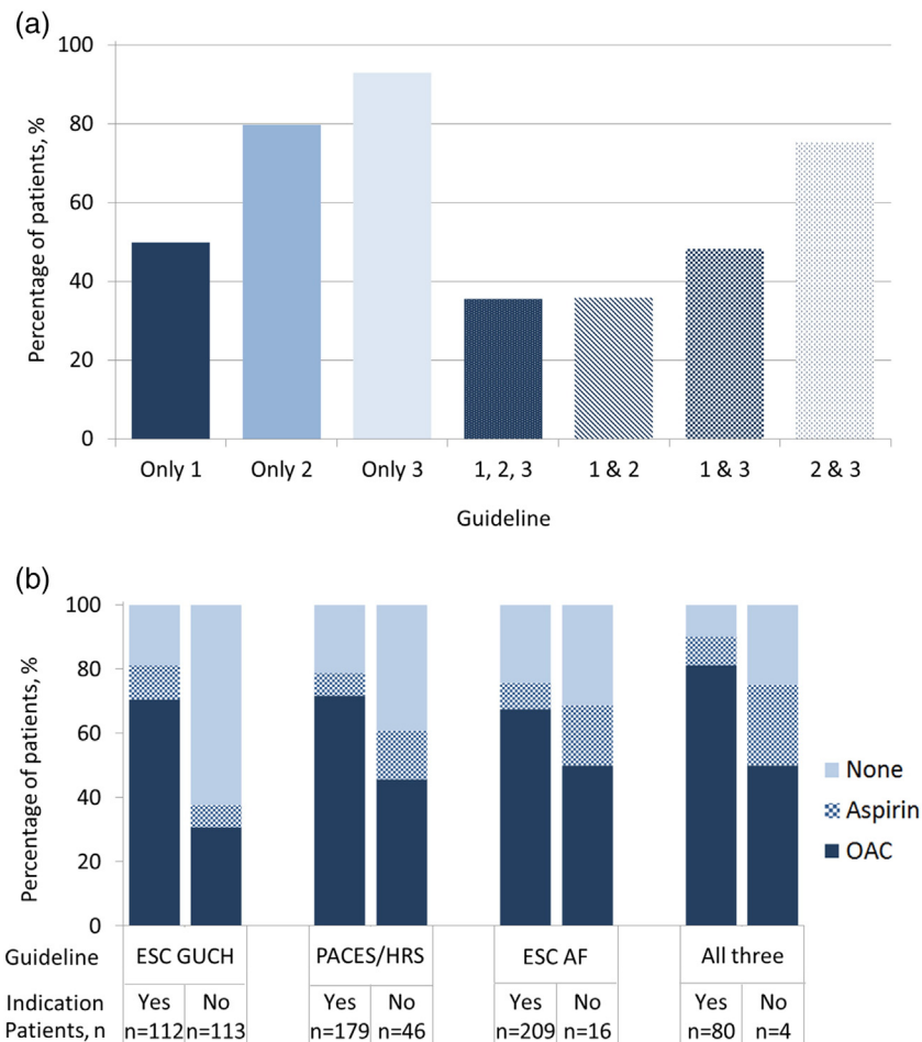
Fig. 1. a. Percentage of ACHD patients with atrial arrhythmias and an indication for oral anticoagulant. Percentage of patients, who were indicated for oral anticoagulant according to (combination of) each guideline. Guideline 1 = 2010 European Society of Cardiology (ESC) guidelines for the management of grown-up congenital heart disease (ESC GUCH). Guideline 2 = 2014 Pediatric and Congenital Electrophysiology Society (PACES)/Heart Rhythm Society (HRS) recognition and management of arrhythmias in adult congenital heart disease (PACES/HRS). Guideline 3 = 2016 ESC guidelines for the management of atrial fibrillation (ESC AF). Abbreviations: ACHD = adult congenital heart disease b. Percentage of oral anticoagulant prescription in ACHD patients with atrial arrhythmias. Percentages of patients with anti-thrombotic therapy (oral anticoagulant, aspirin or none) are illustrated by whether the patients were indicated for oral anticoagulant according to the guidelines. Abbreviations: ESC GUCH = 2010 European Society of Cardiology (ESC) guidelines for the management of grown-up congenital heart disease, PACES/HRS = 2014 Pediatric and Congenital Electrophysiology Society (PACES)/Heart Rhythm Society (HRS) recognition and management of arrhythmias in adult congenital heart disease (PACES/HRS), ESC AF = 2016 ESC guidelines for the management of atrial fibrillation.
