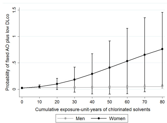
Figure 3. The association between years of chlorinated solvents exposure and probability of fixed AO plus low DLco, stratified by sex. Circles represent the probability of the outcome (fixed AO plus low DLco), and the bars represent the 95% confidence interval of that probability.
