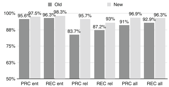
Fig. 11 Web individual PRC and RCL change
