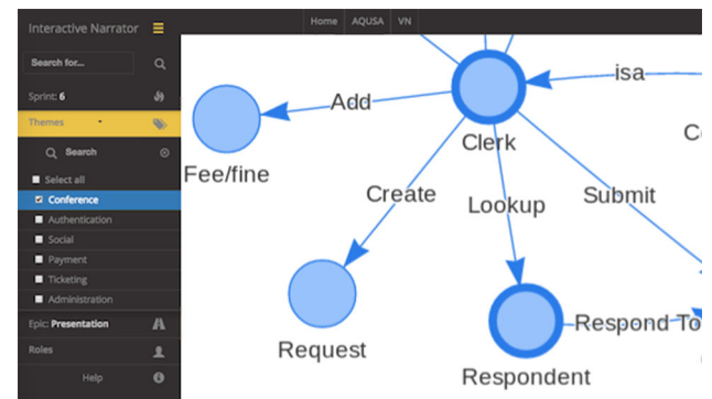
Fig. 4 Filter example showing entities and relationships for user stories in sprint 6 belonging to theme Conference and epic Presentation
