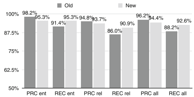
Fig. 12 Web set PRC and RCL change
